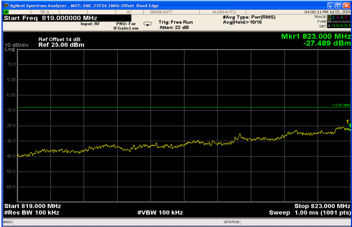
Channel 1013 - Lower Band Edge
