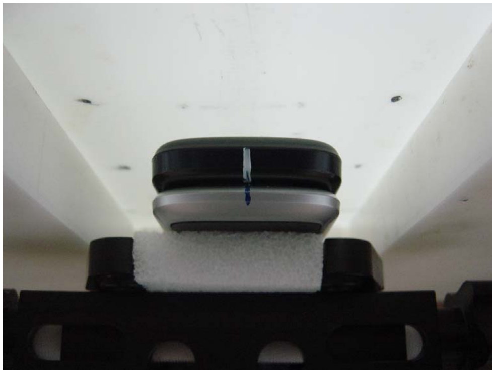
Figure 6: Phone Against the Flat Phantom (Back of phone 15mm from phantom)
