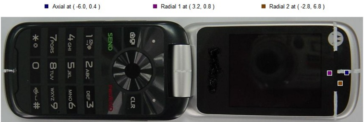
Figure 8. Location of Measured Points for T-coil measurements
