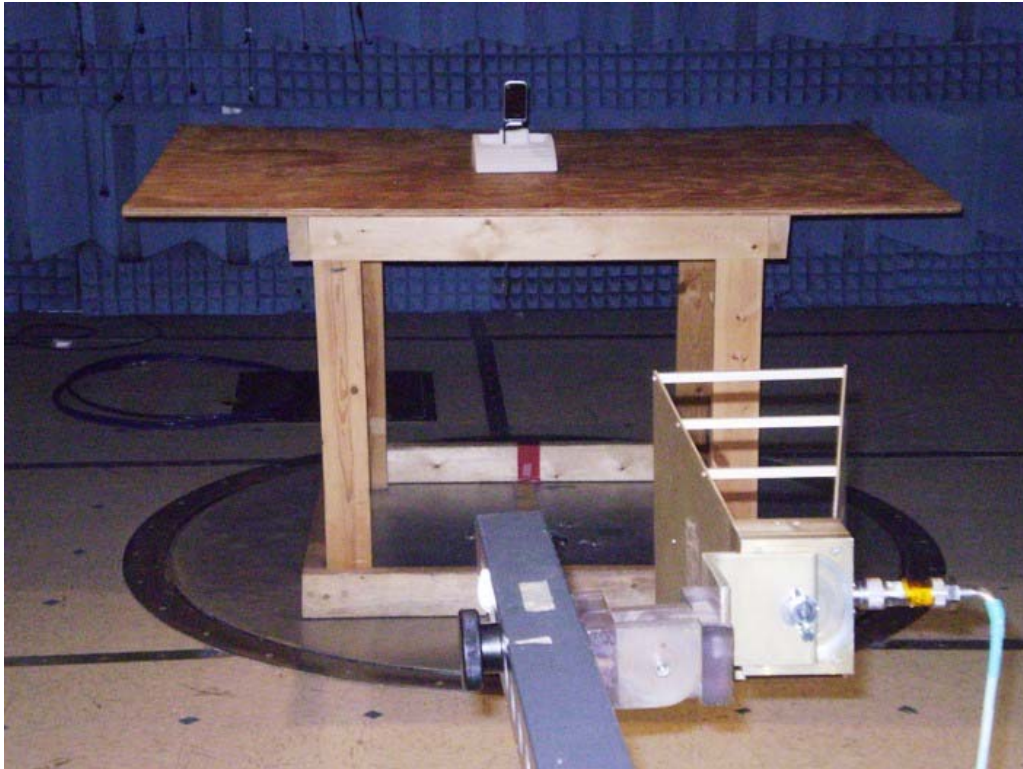
EMC Report #22903 Tx Radiated
