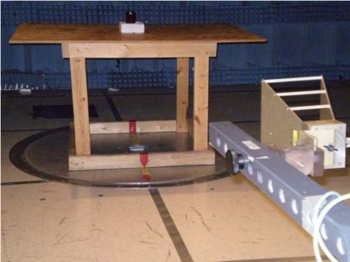
EMC Report #22333 Tx Radiated
