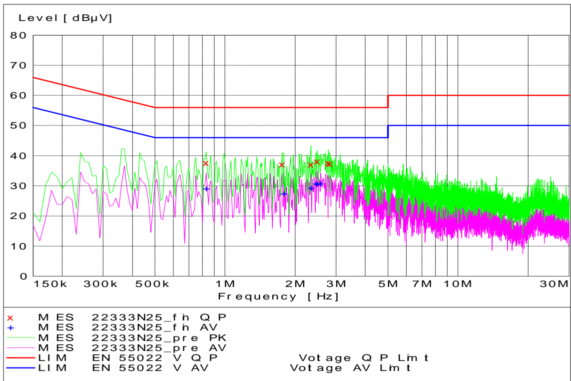
PCS Channel 25 - Tx Mode - Neutral Coupling
