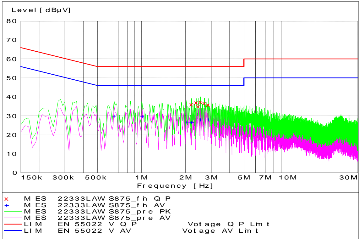
AWS Channel 875 - Tx Mode - Line Coupling
