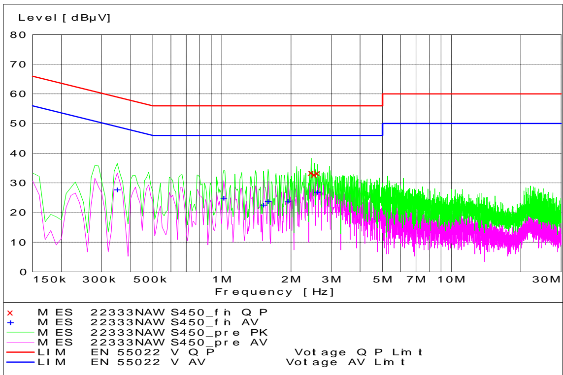
AWS Channel 450 - Tx Mode - Neutral Coupling
