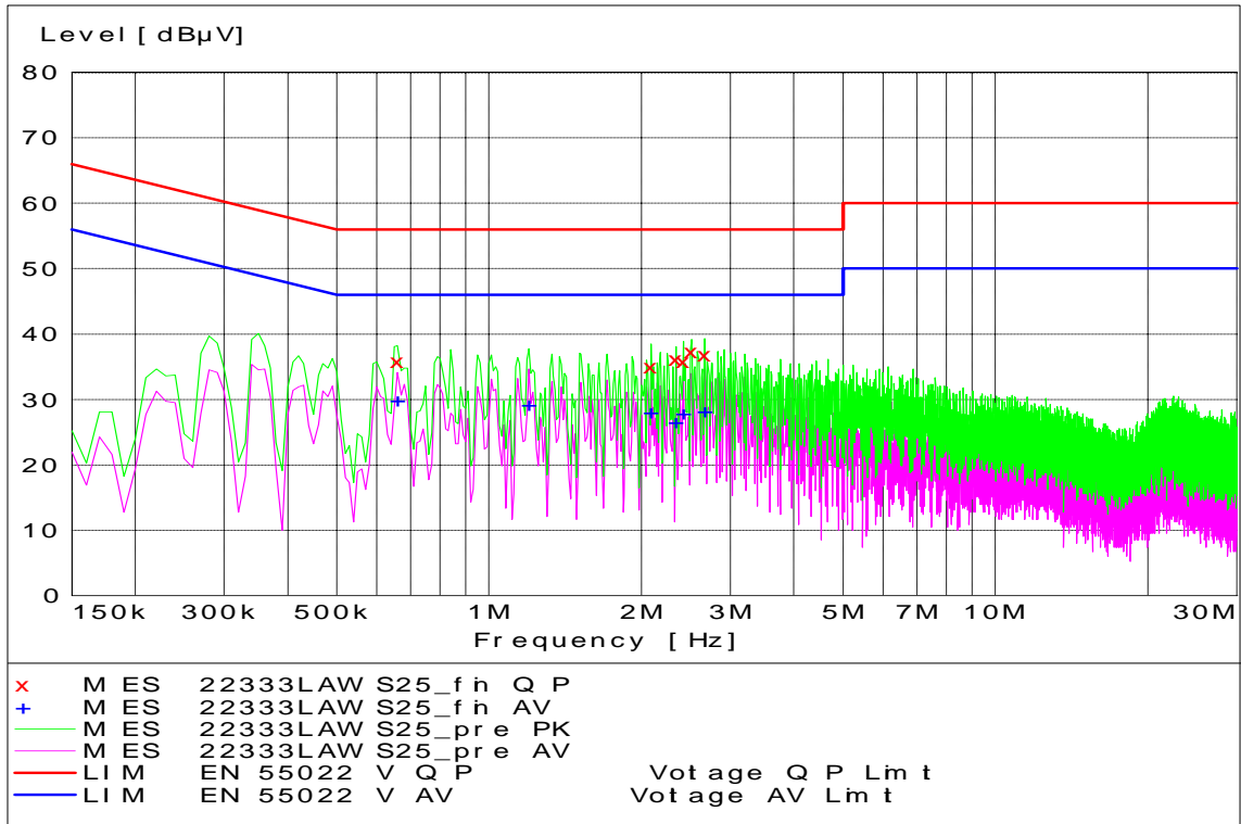
AWS Channel 25 - Tx Mode - Line Coupling
