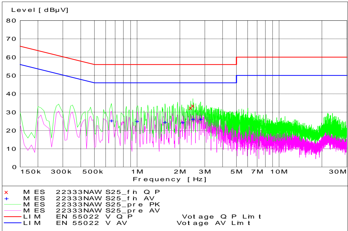
AWS Channel 25 - Tx Mode - Neutral Coupling
