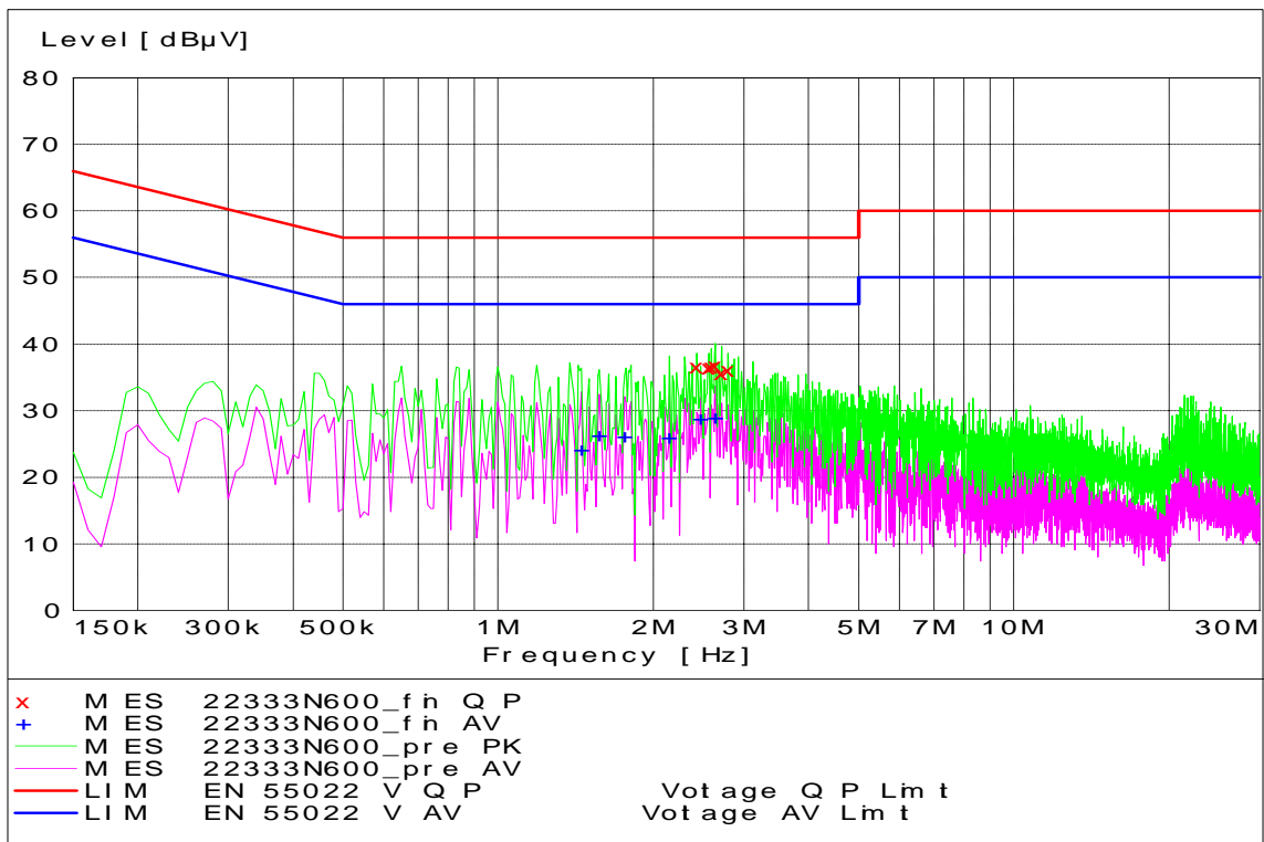
PCS Channel 600 - Tx Mode - Neutral Coupling
