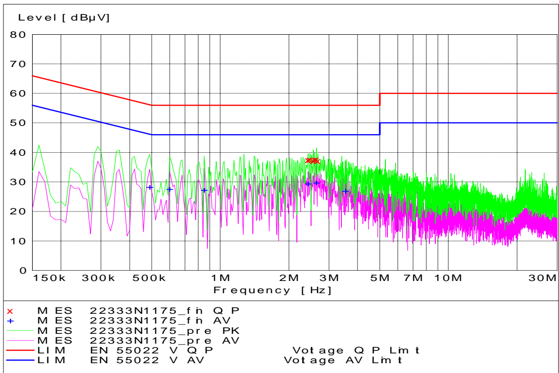
PCS Channel 1175 - Tx Mode - Neutral Coupling
