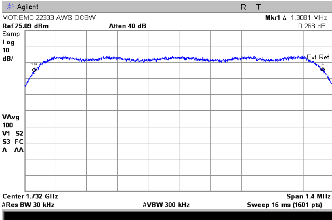
CDMA 1700 – Occupied Bandwidth – Channel 450 (1732.50 MHz)
