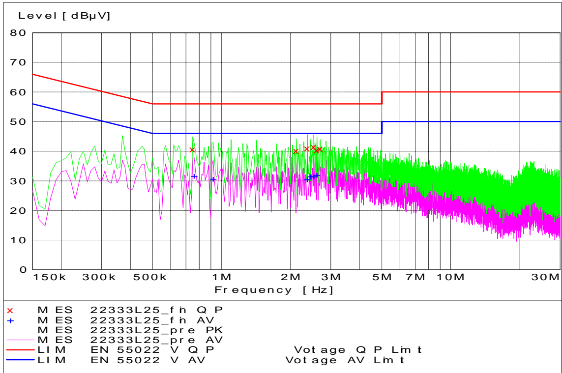
PCS Channel 25 - Tx Mode - Line Coupling
