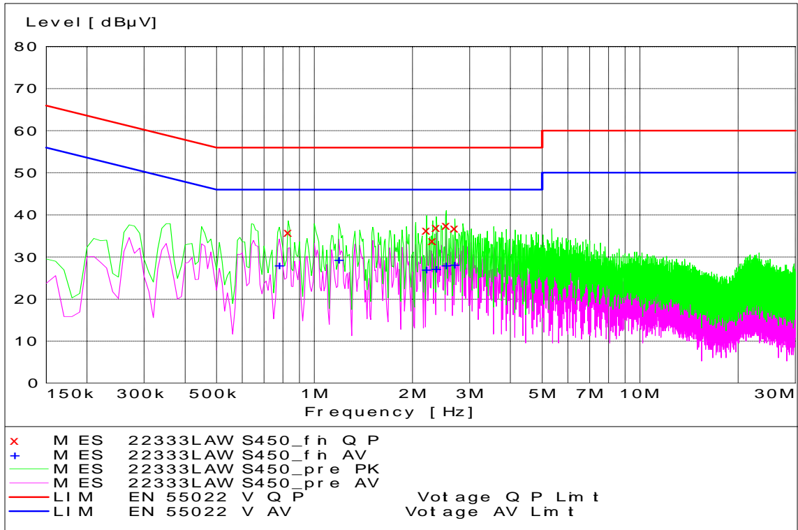
AWS Channel 450 - Tx Mode - Line Coupling
