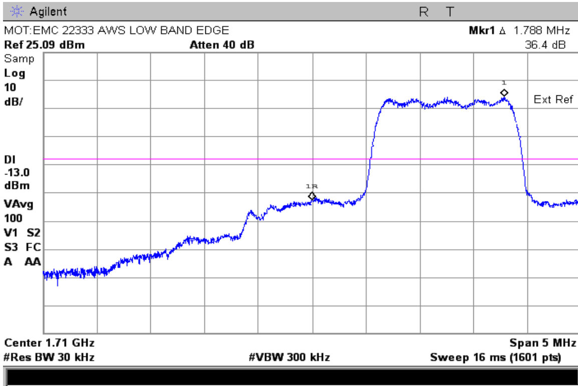
CDMA 1700 – Lower Band Edge – Channel 25 (1711.25 MHz)
