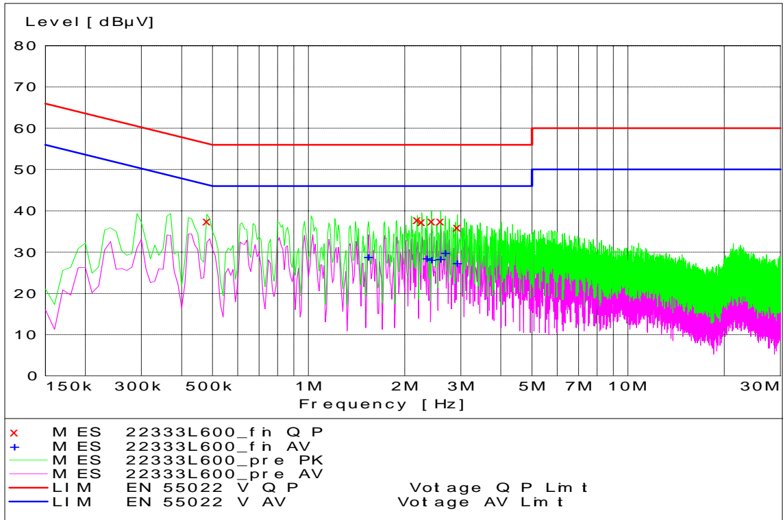
PCS Channel 600 - Tx Mode - Line Coupling
