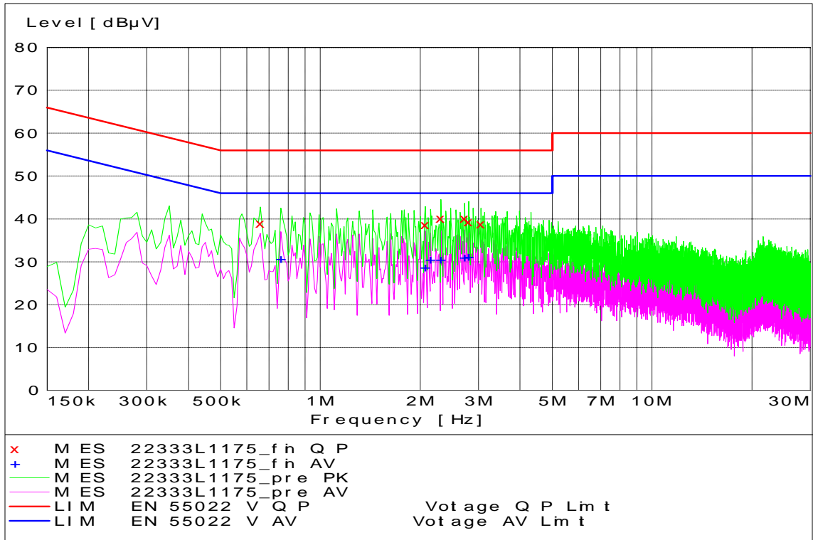
PCS Channel 1175 - Tx Mode - Line Coupling
