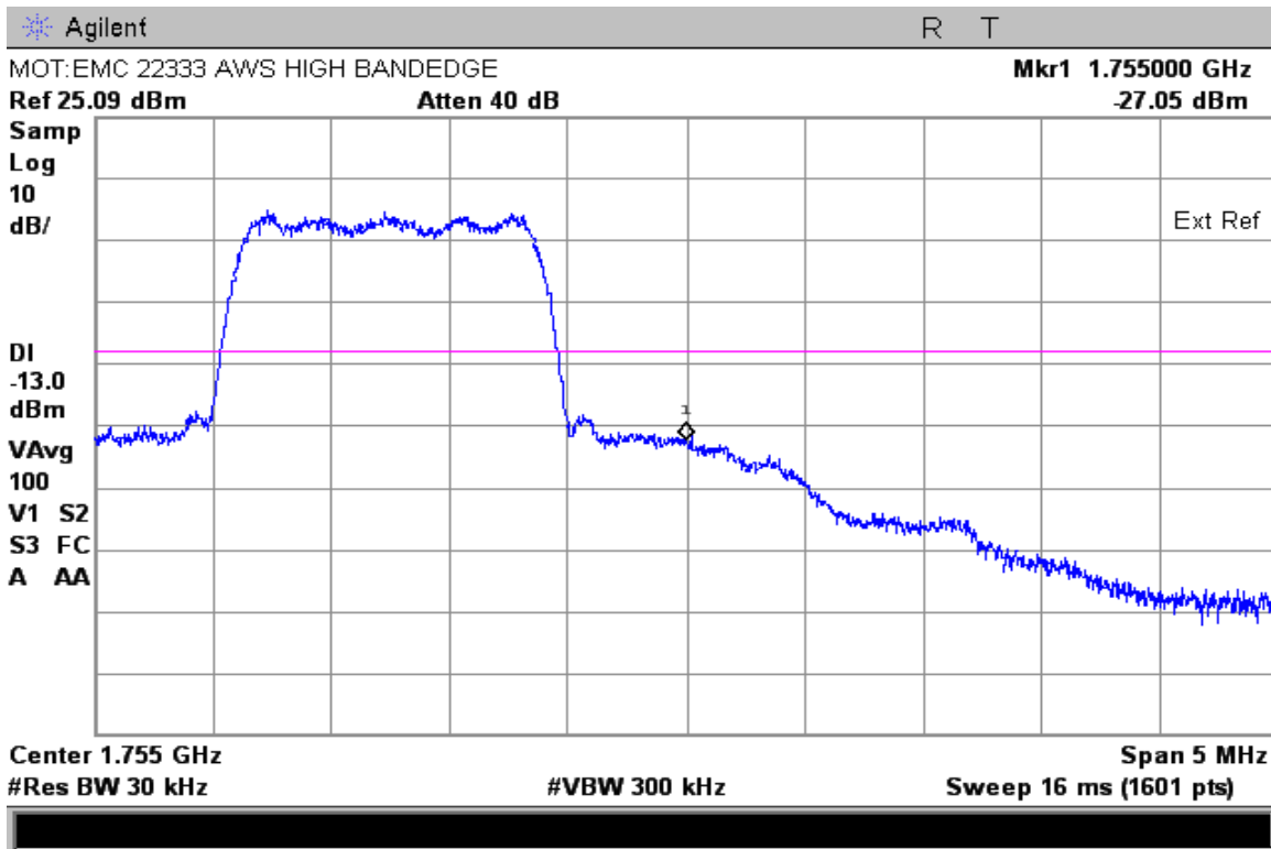
CDMA 1700 – Upper Band Edge – Channel 875 (1753.75MHz)
