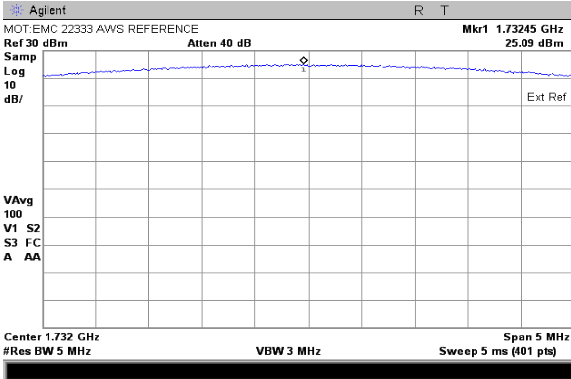
CDMA 1700 – Reference Level Plot – Channel 450 (1732.50 MHz)
