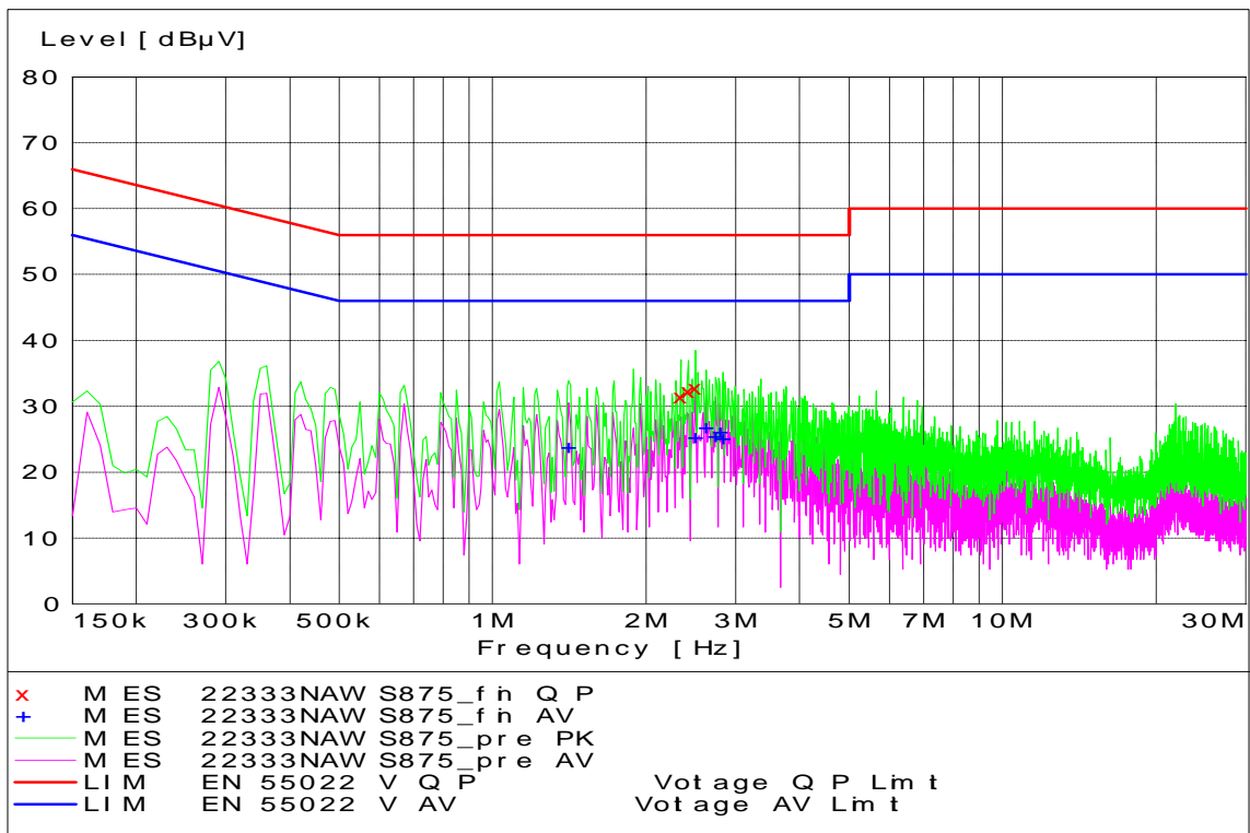
AWS Channel 875 - Tx Mode - Neutral Coupling
