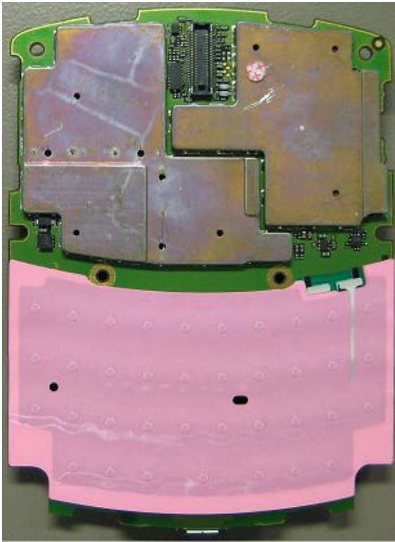
Main Board Top With Shields & Popples
