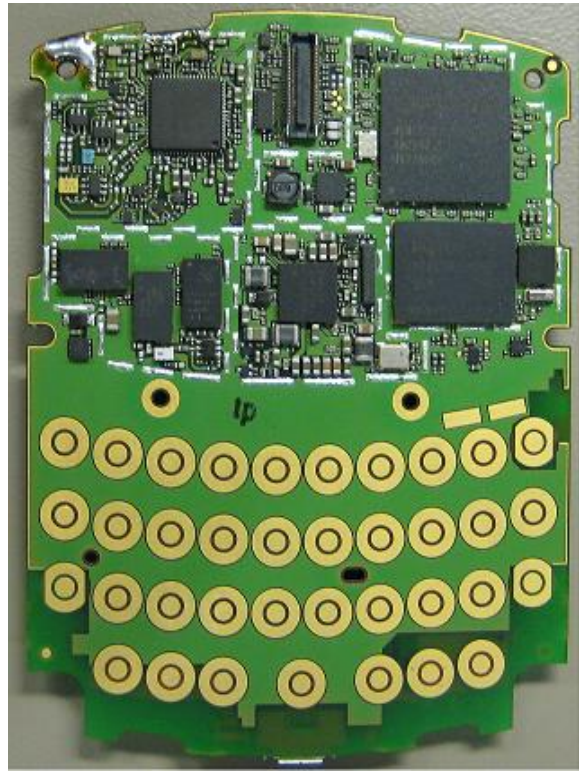
Main Board Top Without Shields & Popples
