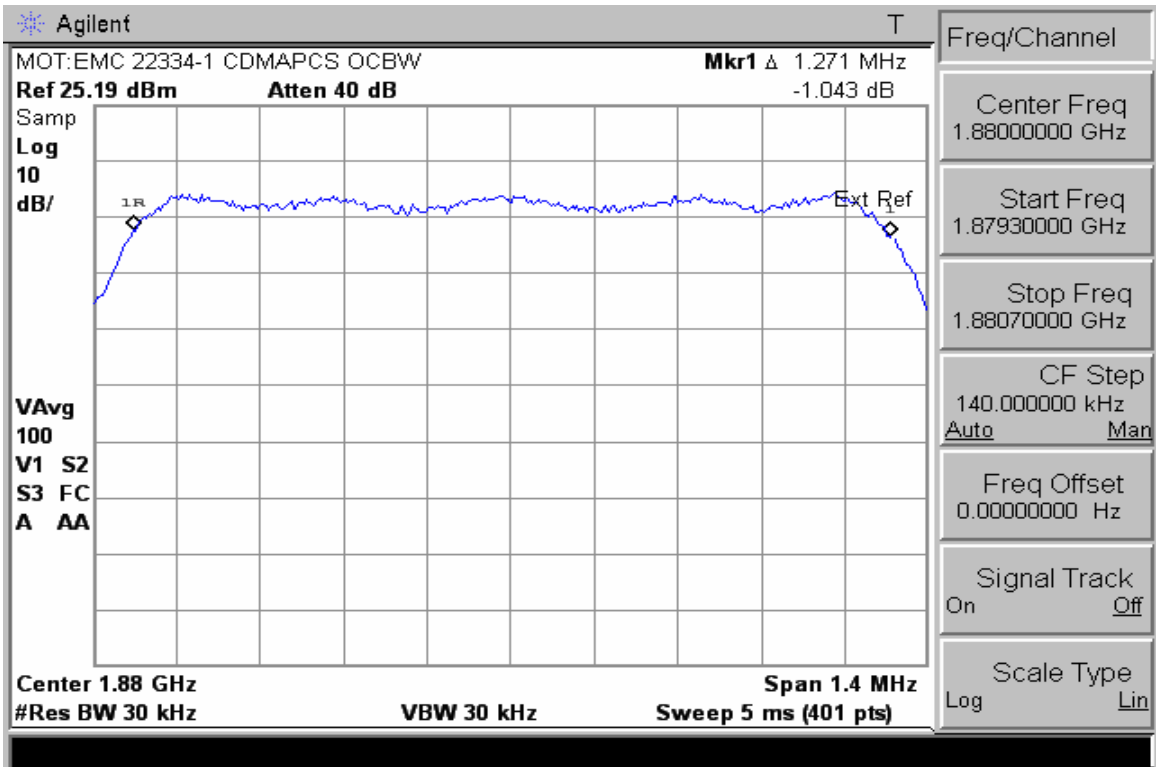
1900 CDMA – Occupied Bandwidth – Channel 600 (1880.00 MHz)
