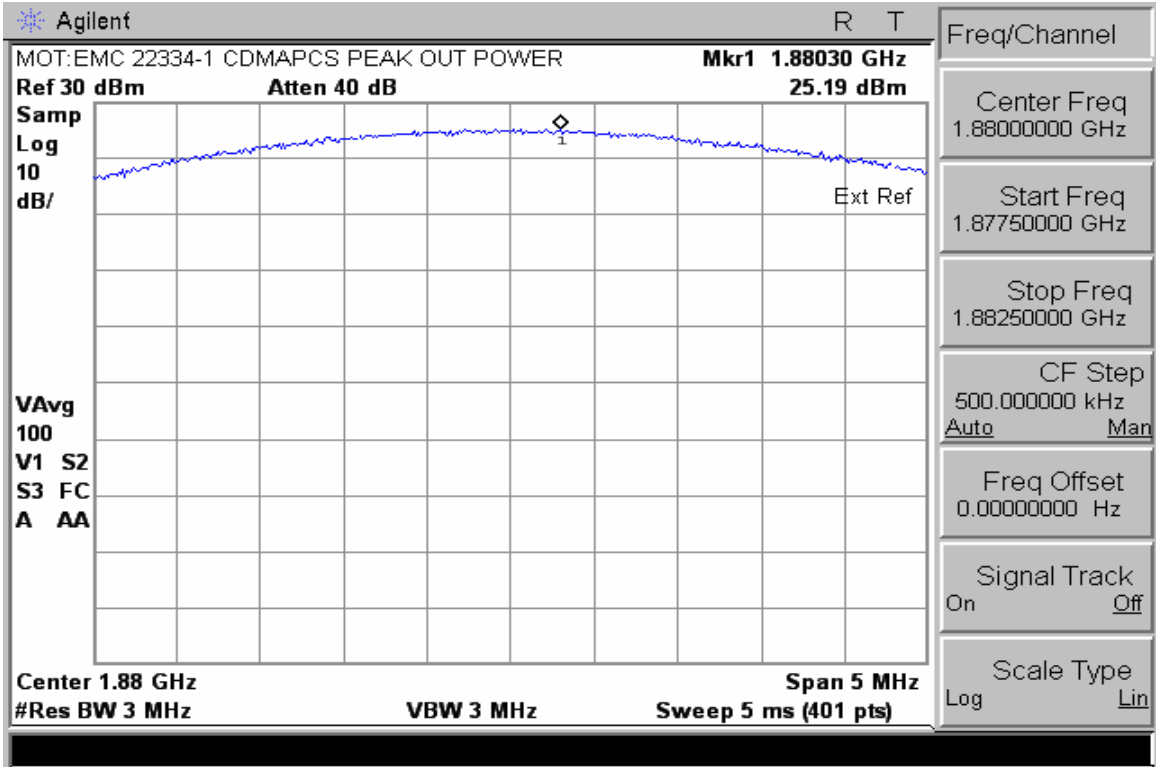
1900 CDMA – Reference Level Plot – Channel 600 (1880.00 MHz)
