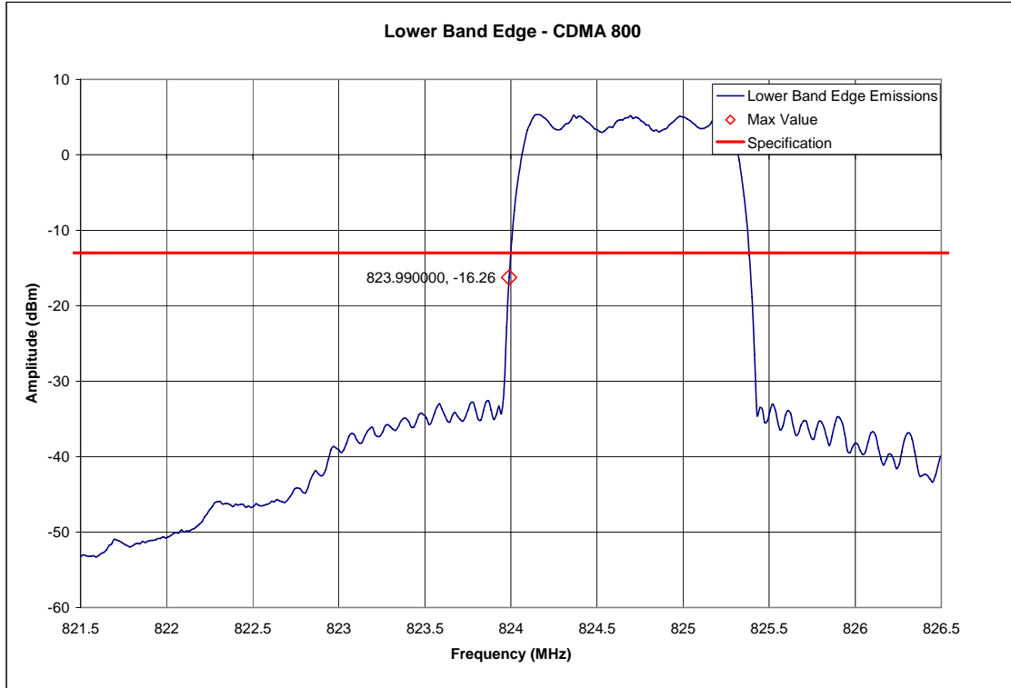
800 CDMA – Lower Band Edge – Channel 1013 (824.702MHz)
