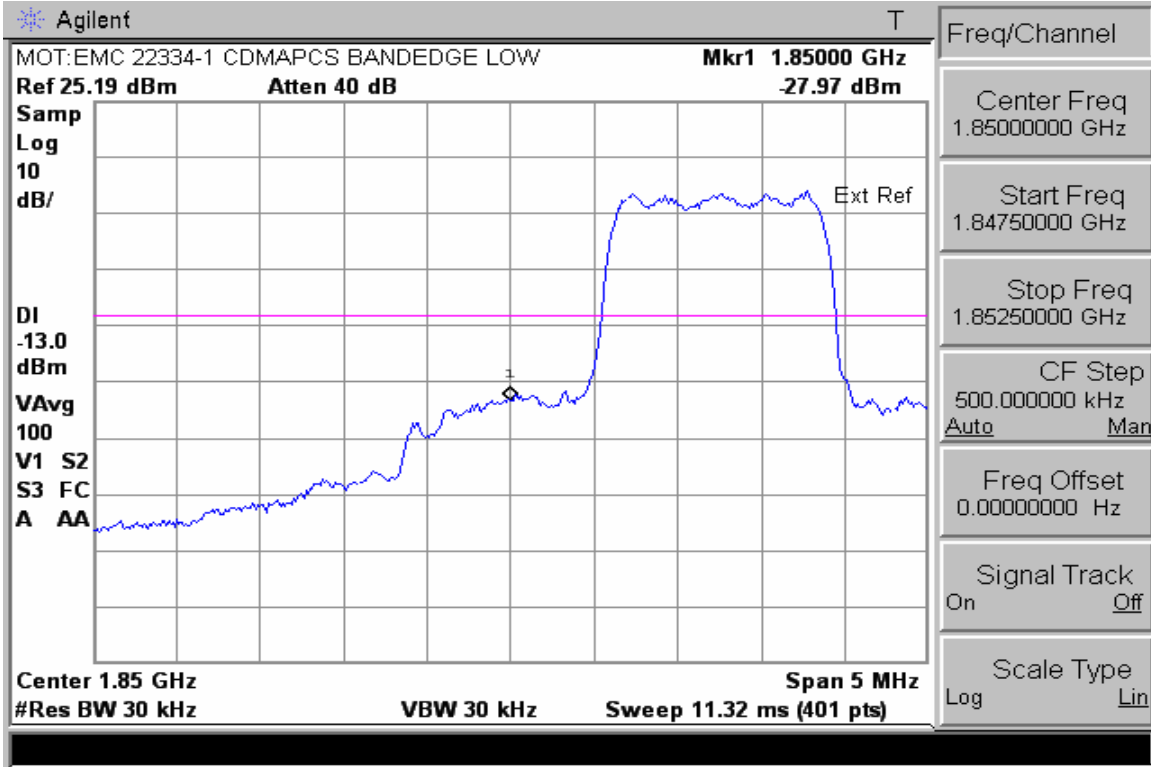
1900 CDMA – Lower Band Edge – Channel 25 (1851.25 MHz)
