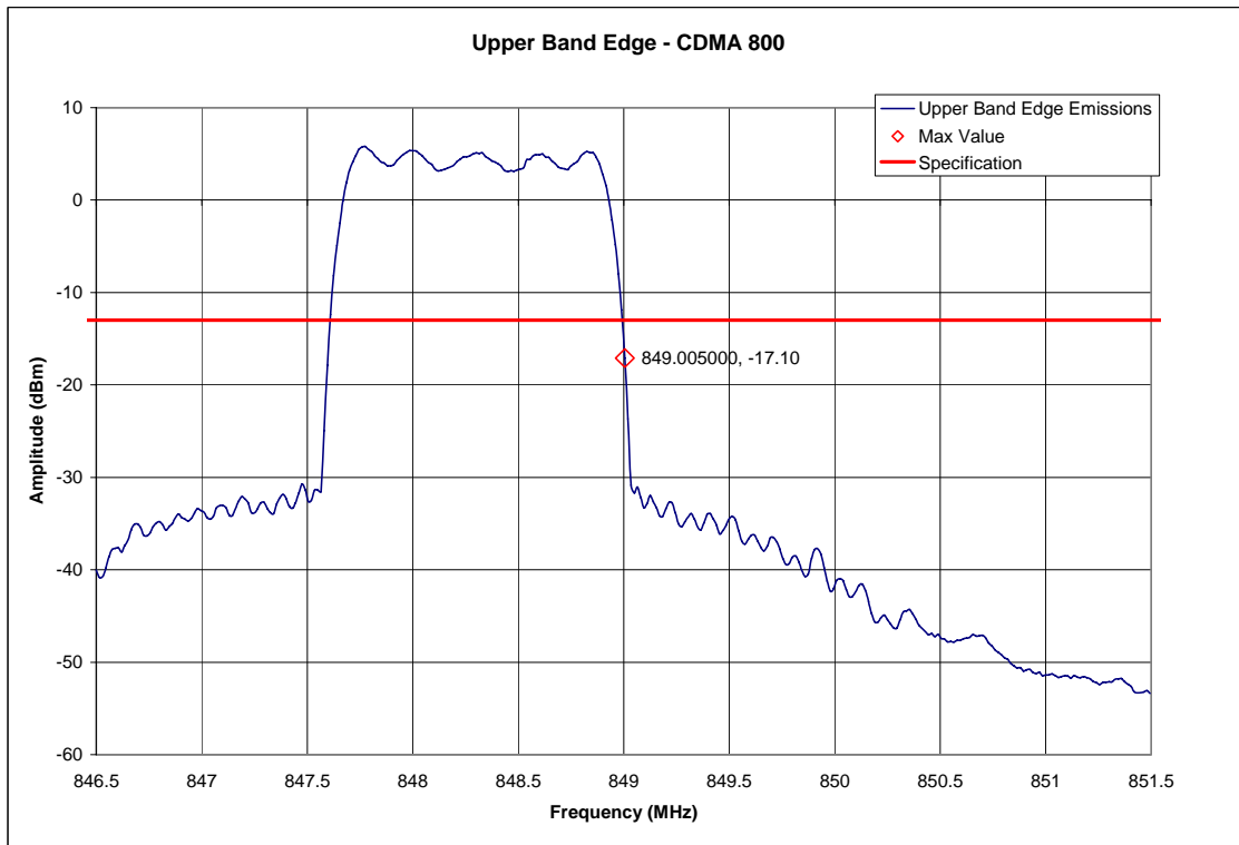
800 CDMA – Upper Band Edge – Channel 777 (848.31MHz)
