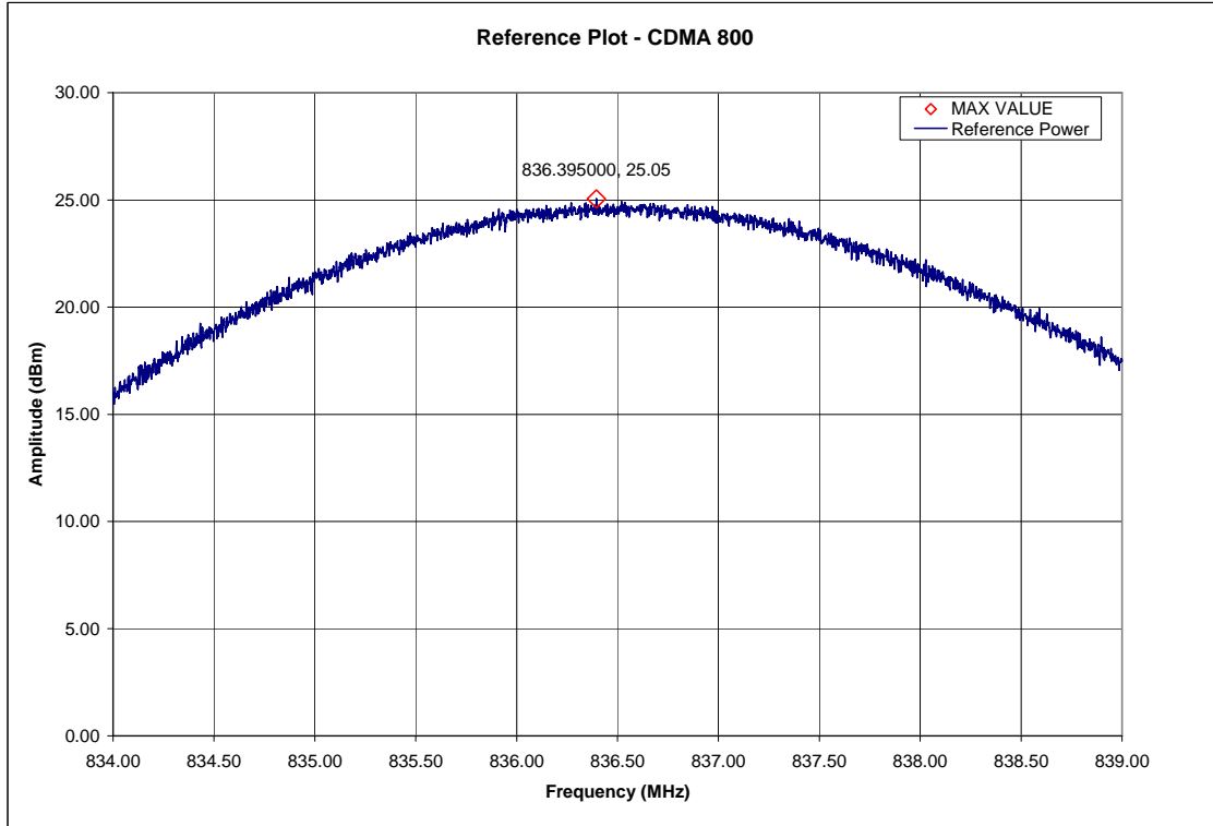
800 CDMA – Reference Level Plot – Channel 384 (836.52MHz)
