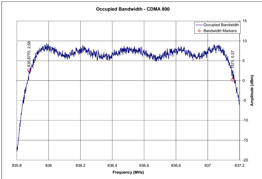
800 CDMA – Occupied Bandwidth – Channel 384 (836.52MHz)
