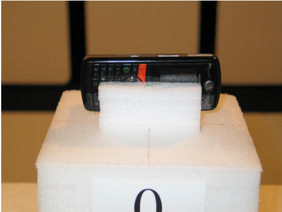
22136-1, IHDP56JS1 placed in test position Y
