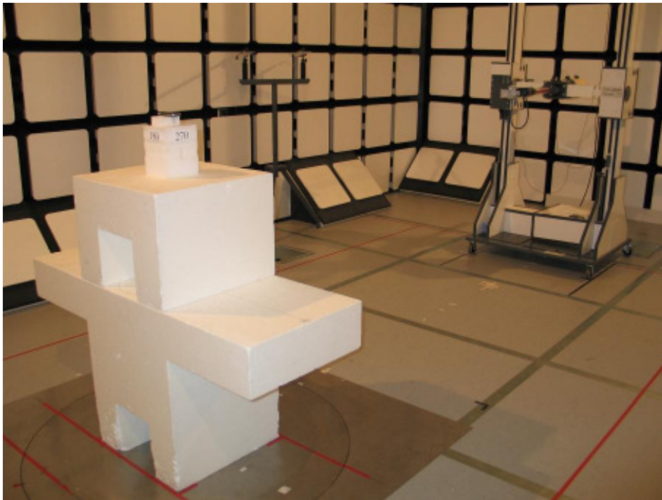
22136-1, IHDP56JS1 setup in semi-anechoic chamber – right side
