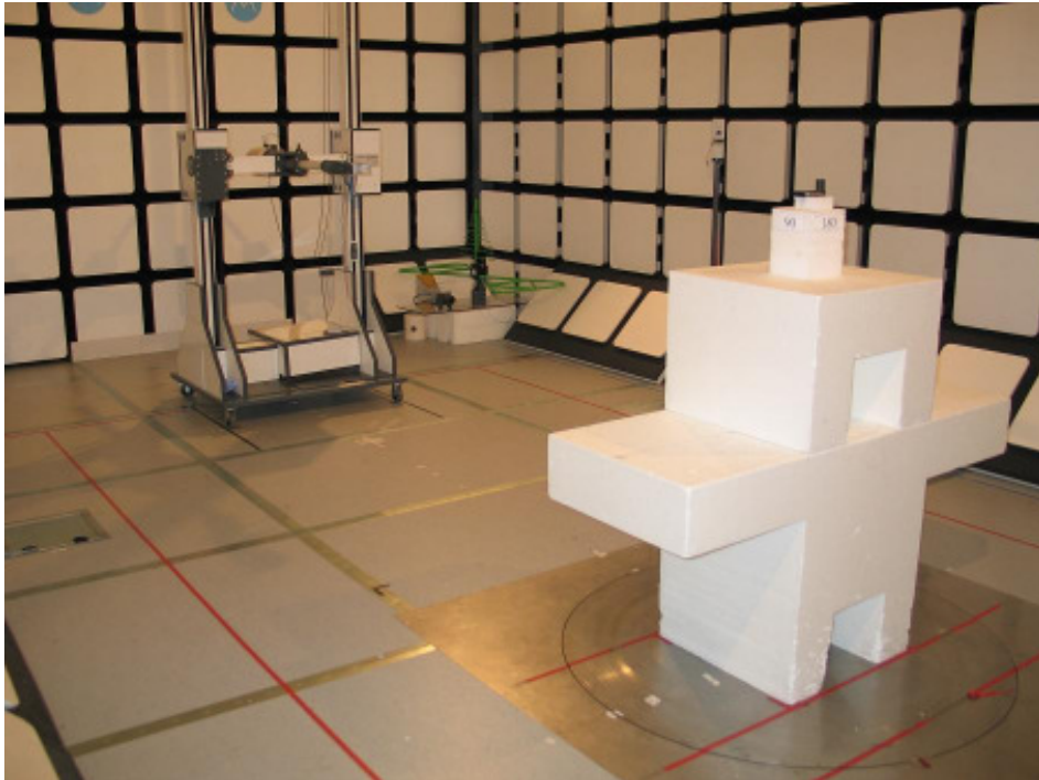
22136-1, IHDP56JS1 setup in semi-anechoic chamber – left side
