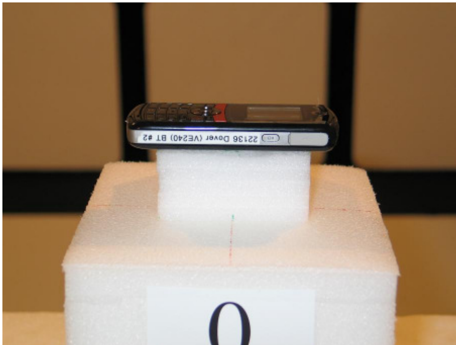
22136-1, IHDP56JS1 placed in test position X
