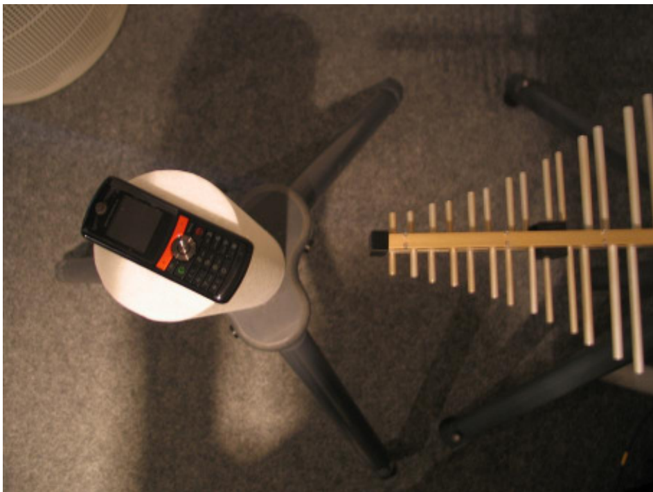
22136-1, IHDP56JS1 check for maximum radiation at position X
