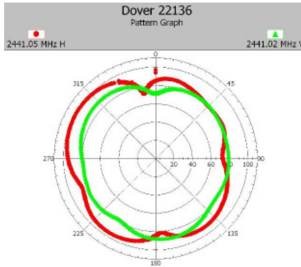
22136-1, IHDP56JS1 maximum radiation pattern position X
