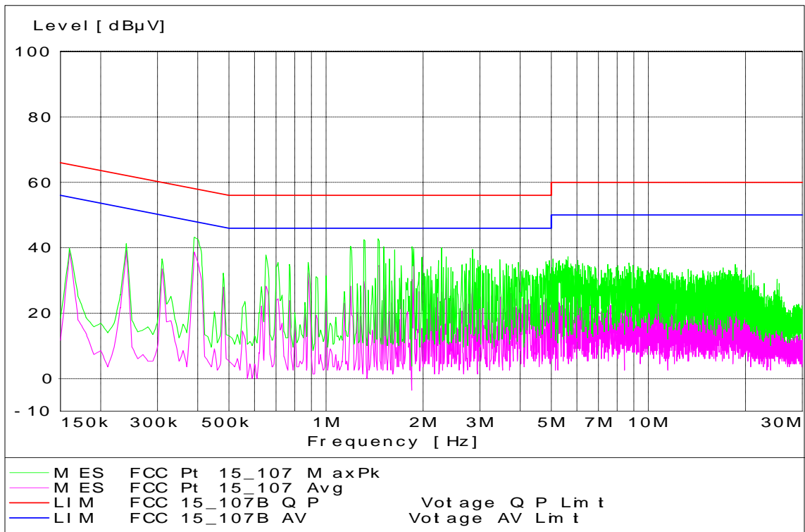
CDMA 1700 Channel 875 - Tx Mode - Neutral Coupling
