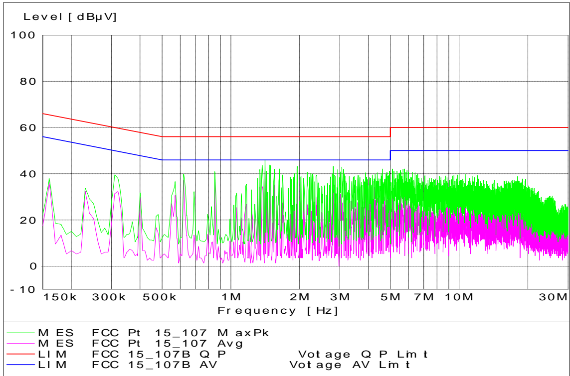
CDMA 1700 Channel 25 - Tx Mode - Line Coupling
