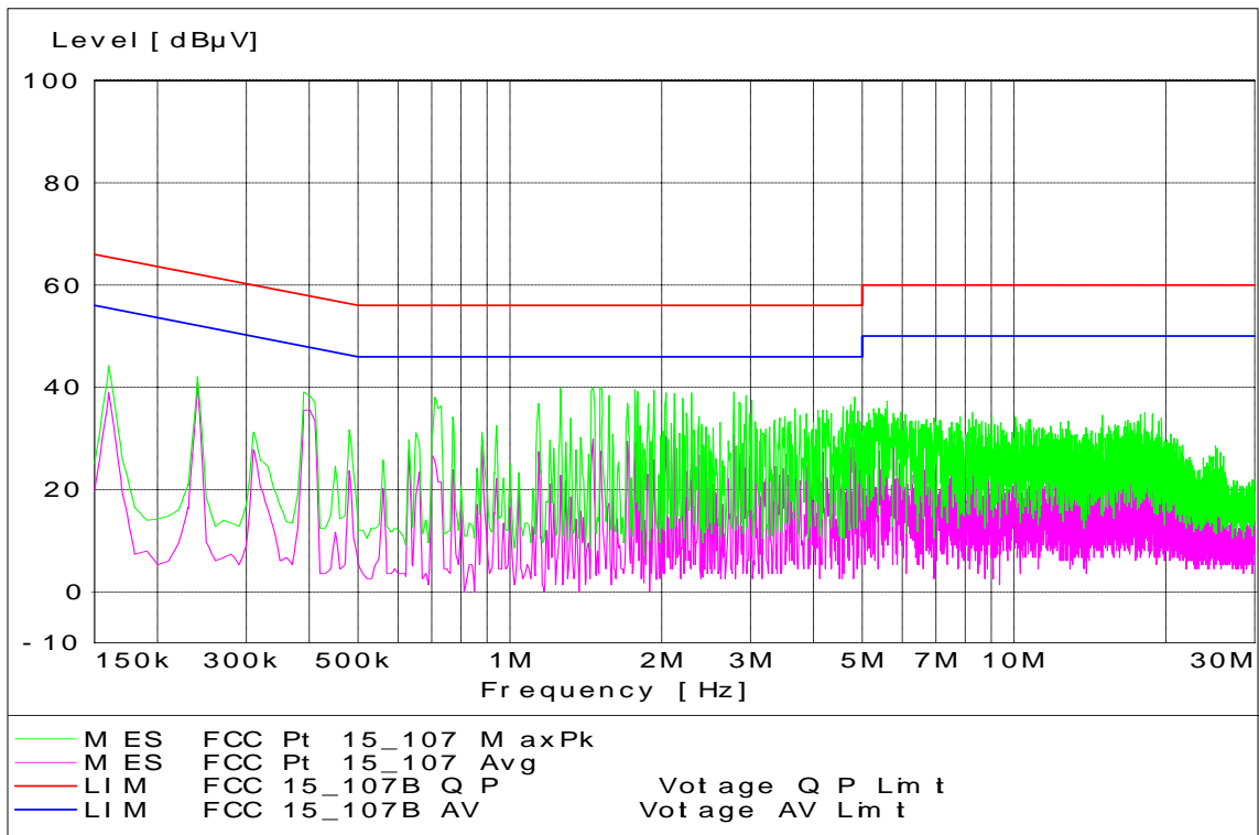
CDMA 1900 Channel 1175 - Tx Mode - Neutral Coupling
