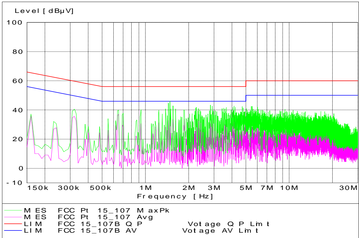
CDMA 1700 Channel 450 - Tx Mode - Line Coupling
