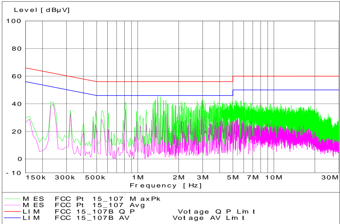
CDMA 1700 Channel 875 - Tx Mode - Line Coupling
