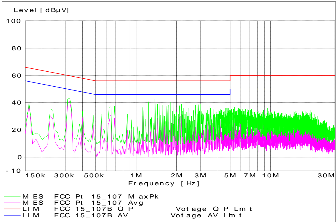
CDMA 1700 Channel 25 - Tx Mode - Neutral Coupling
