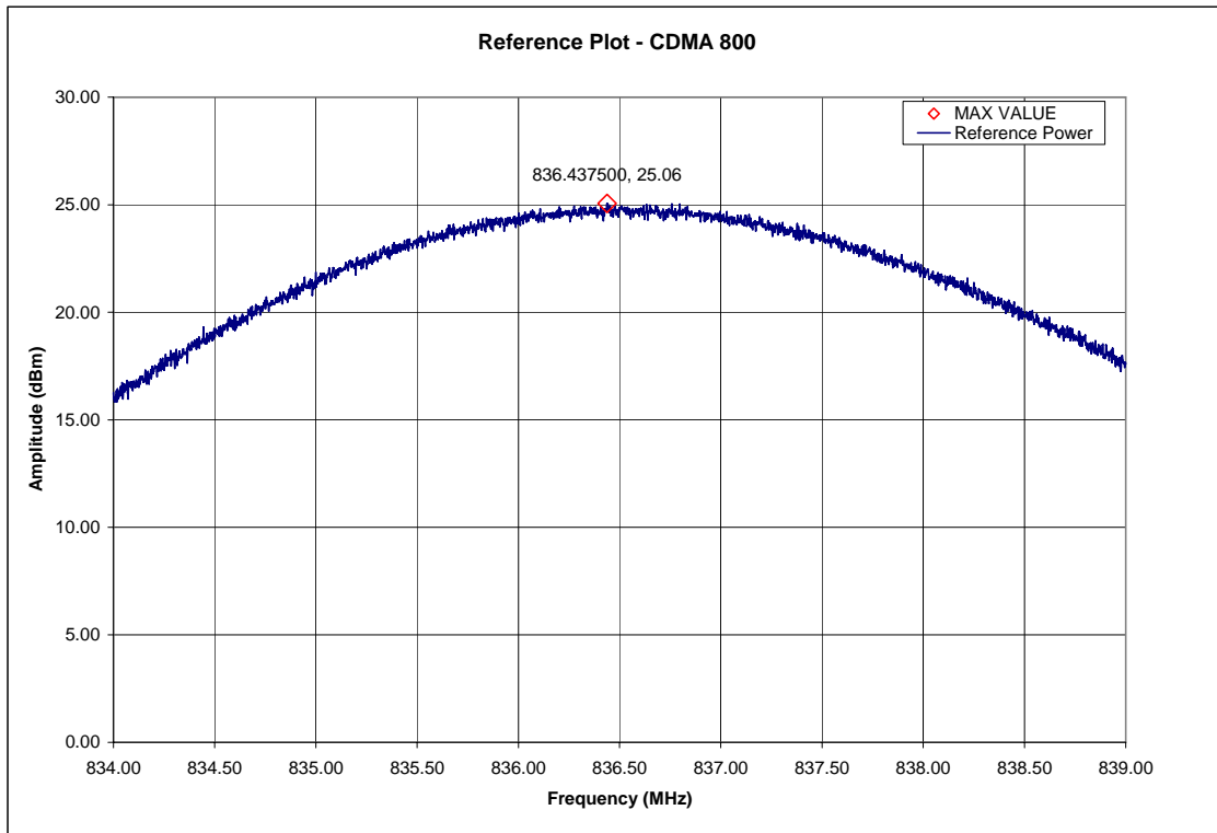
CDMA 800 – Reference Level Plot – Channel 384 (836.52MHz)
