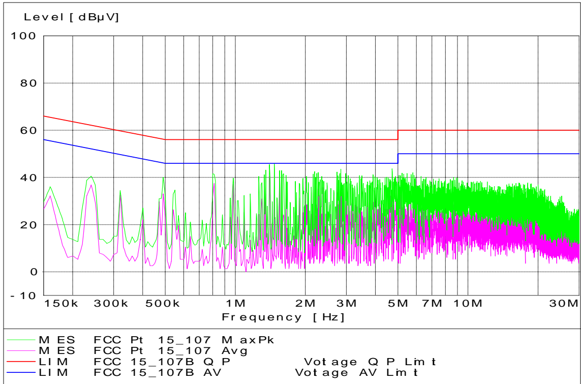
CDMA 1900 Channel 1175 - Tx Mode - Line Coupling
