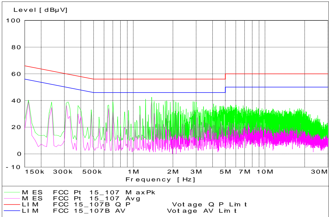
CDMA 1700 Channel 450 - Tx Mode - Neutral Coupling
