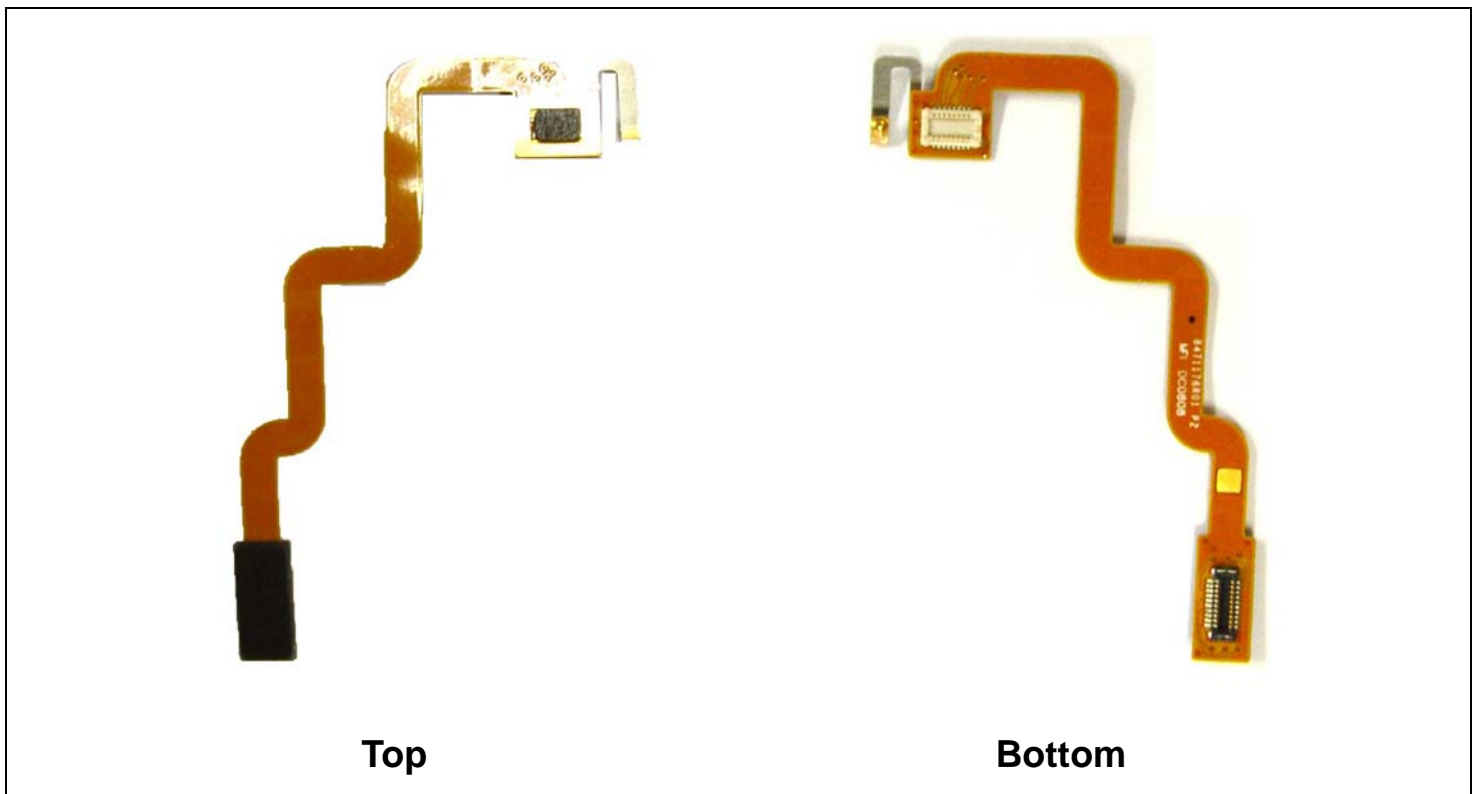
Hinge FPCB
