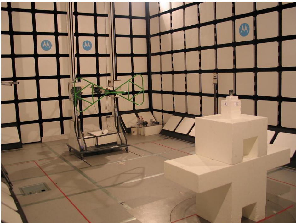
22140-2, IHDP56JL1 setup in semi-anechoic chamber – left view
