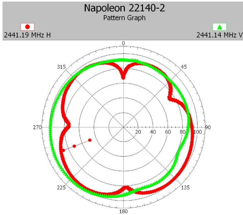
22140-2, IHDP56JL1 Maximum radiation pattern position Y – BT mode
