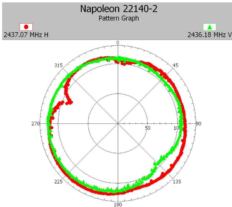
22140-2, IHDP56JL1 Maximum radiation pattern position Y – WiFi mode
