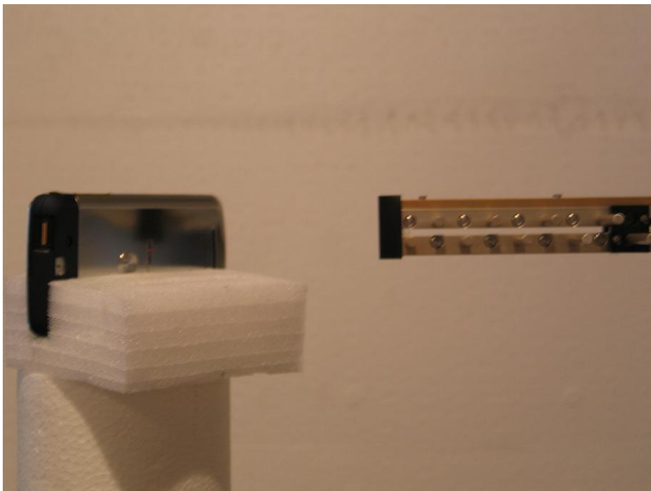
22140-2, IHDP56JL1 Check for maximum radiation at position Y – BT/WiFi mode
