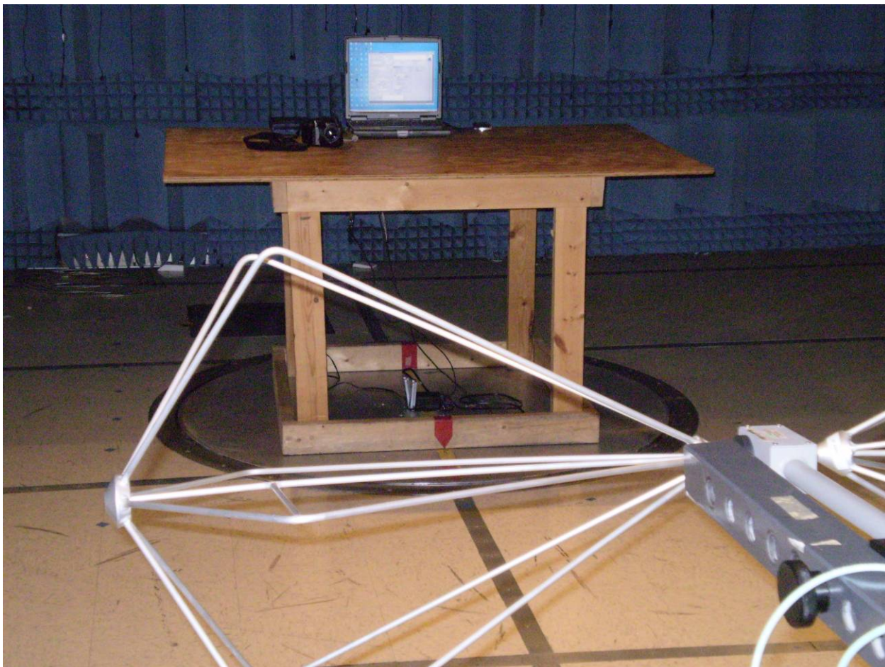
Radiated Emissions – Computer Peripheral
