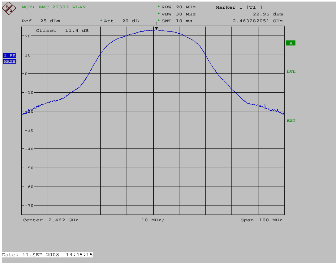
Max. Power Channel 11 @ 36 Mbps
