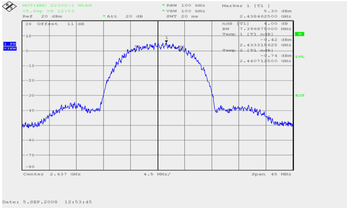
6dB Bandwidth Channel 6 @ 11 Mbps
