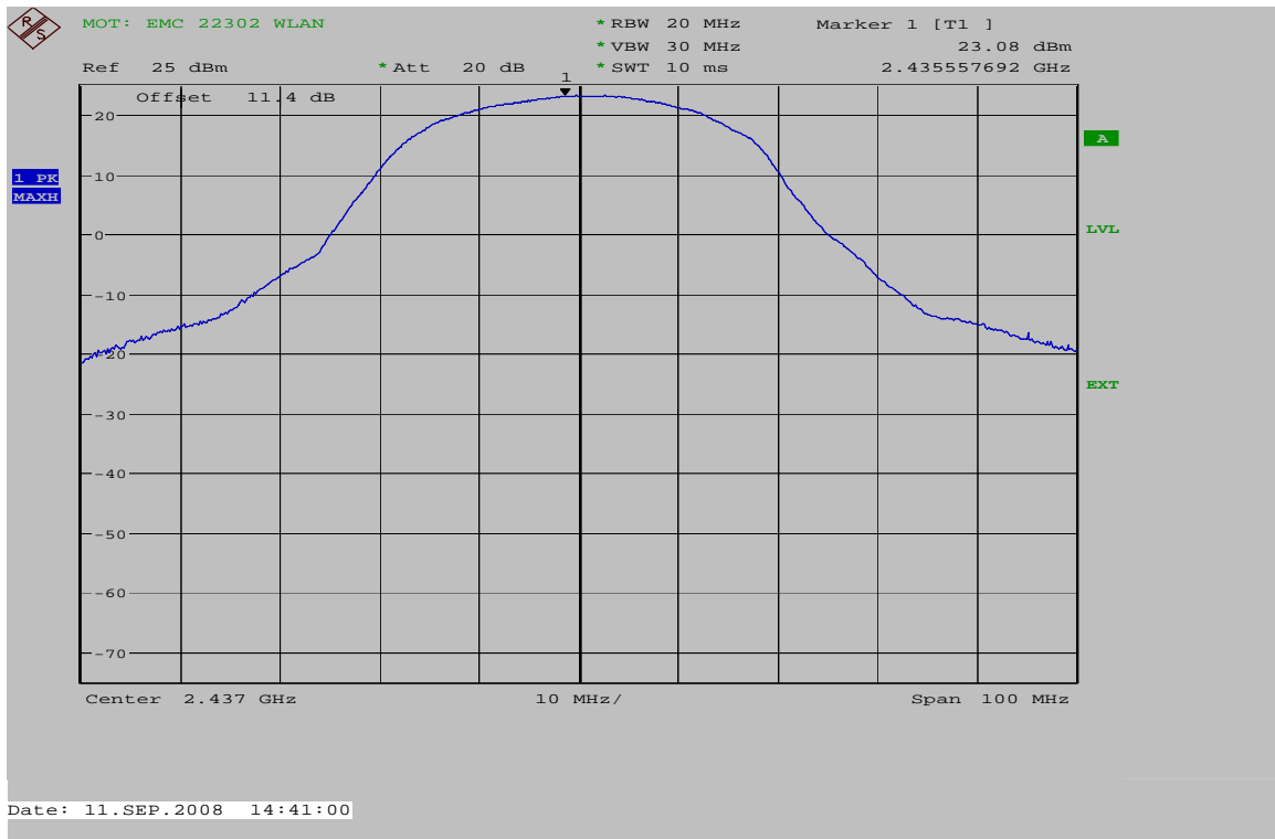
Max. Power Channel 6 @ 36 Mbps
