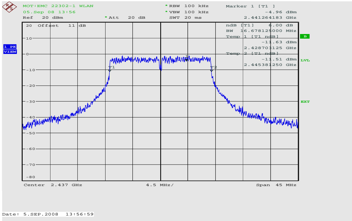
6dB Bandwidth Channel 6 @ 36 Mbps
