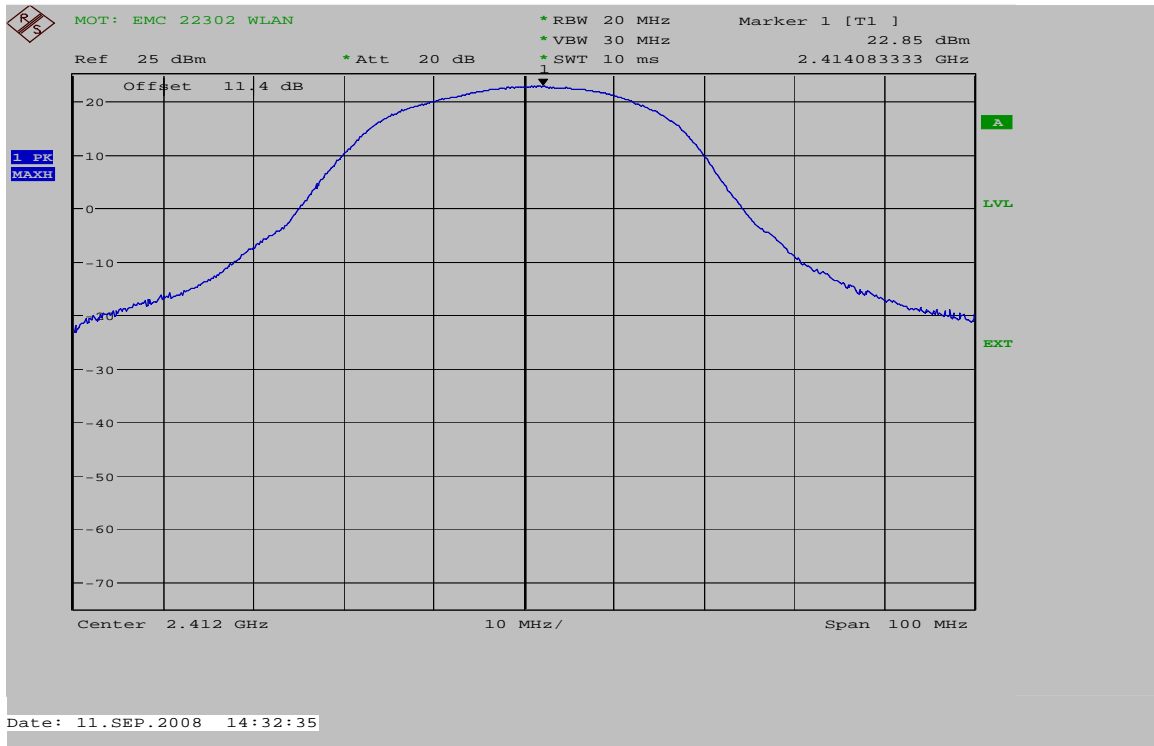
Max. Power Channel 1 @ 36 Mbps
