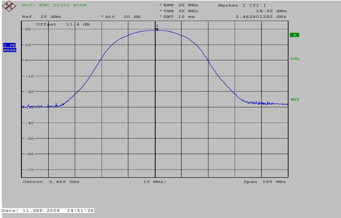
Max. Power Channel 11 @ 11 Mbps
