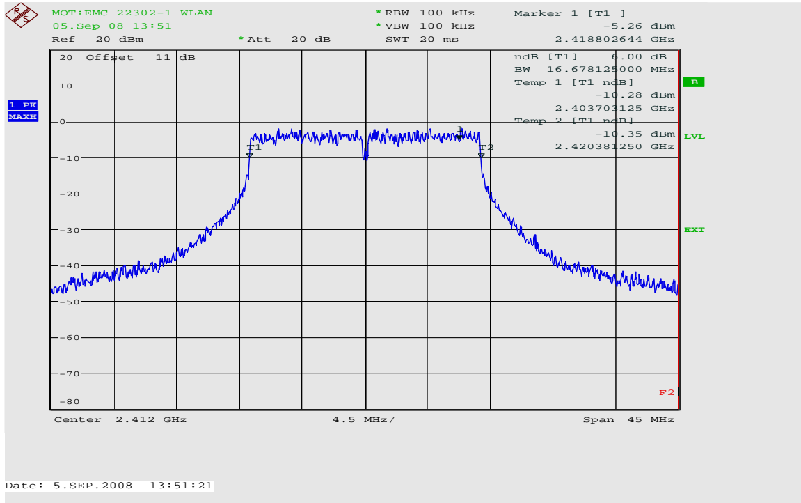
6dB Bandwidth Channel 1 @ 36 Mbps
