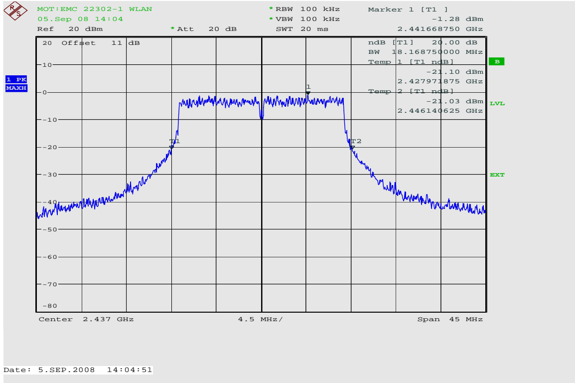
20dB Bandwidth Channel 6 @ 36 Mbps
