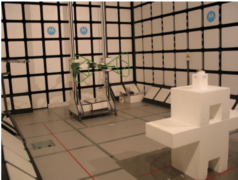
22302-1, IHDP56JK1 setup in semi-anechoic chamber – left view
