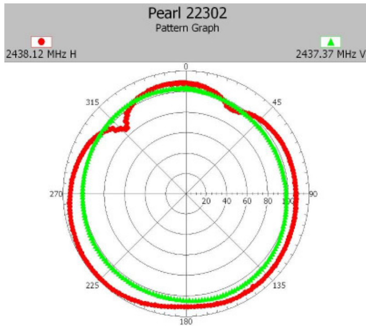
22302-1, IHDP56JK1 Maximum radiation pattern position Y – WiFi mode
