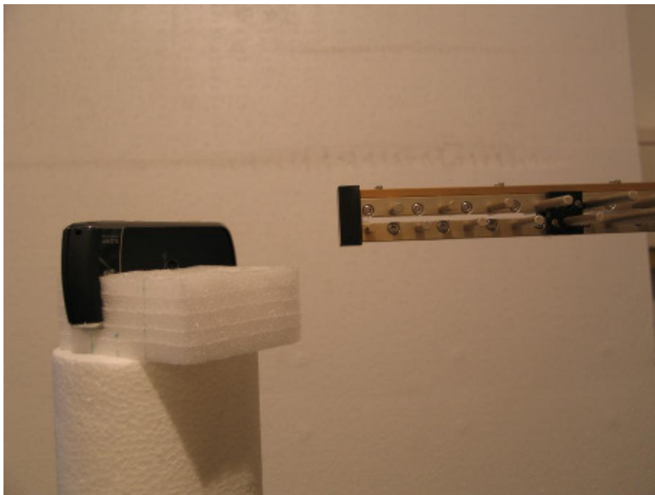
22302-1, IHDP56JK1 Check for maximum radiation at position Y – Closed – BT/WiFi mode
