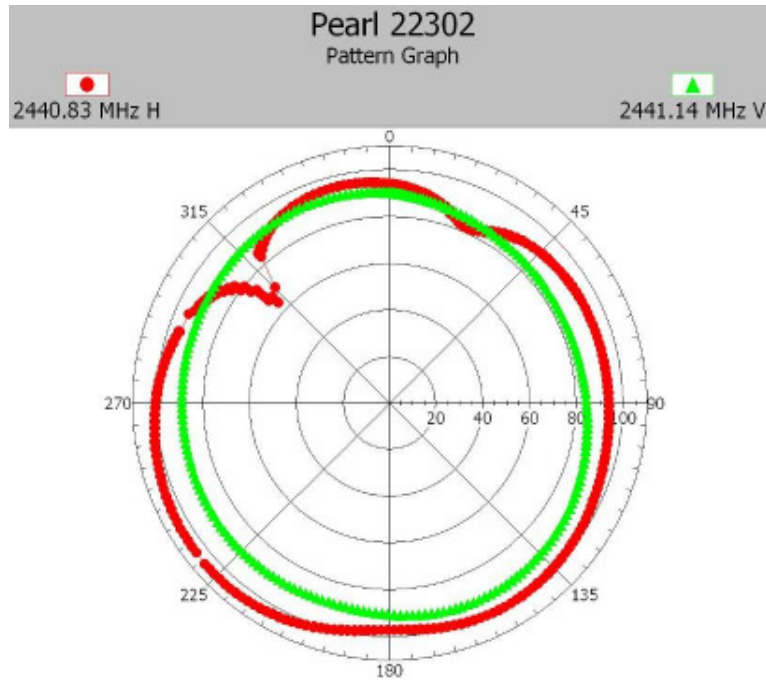
22302-1, IHDP56JK1 Maximum radiation pattern position Y – BT mode
