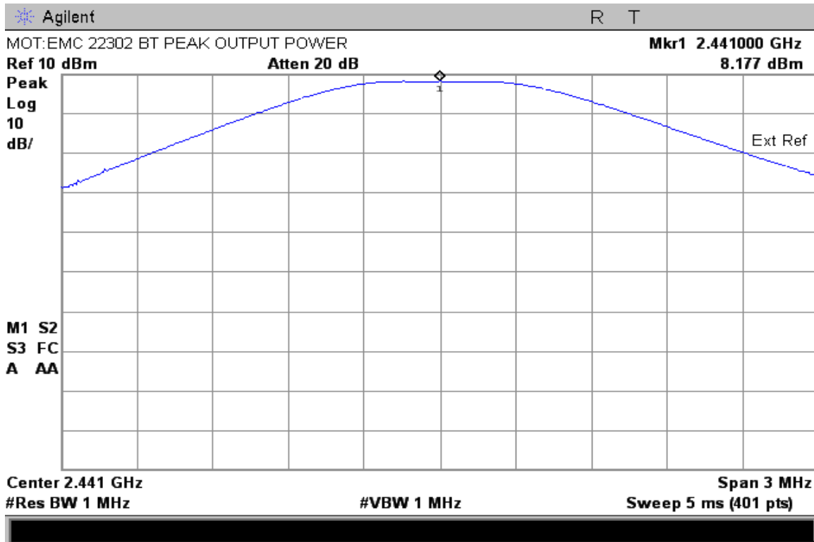
Peak Output Power Non EDR Mode
