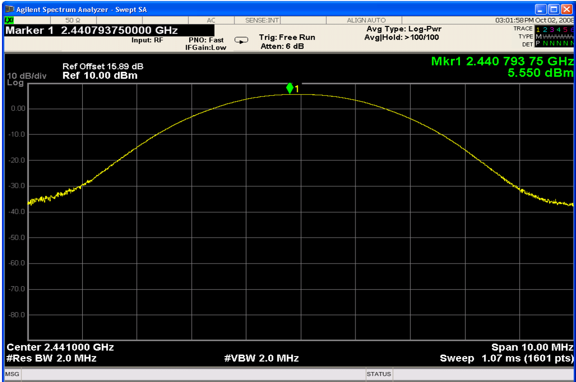
Peak Output Power EDR Mode
