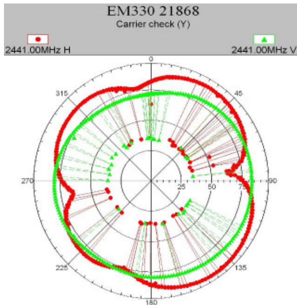
21868-1, IHDP56JJ1 Maximum radiation pattern position Y - Closed
