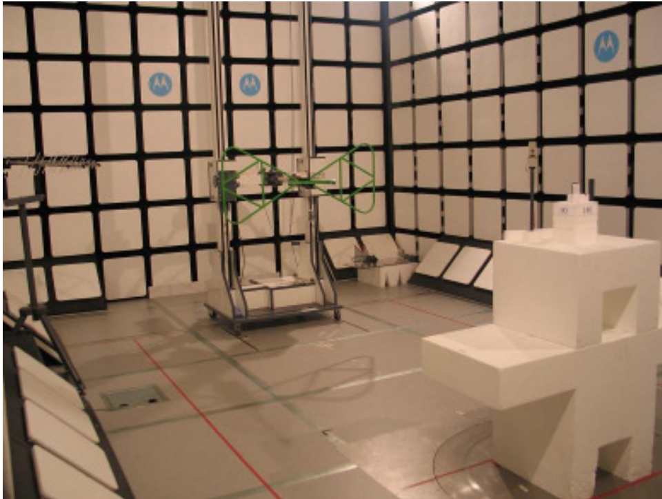
21868-1, IHDP56JJ1 setup in semi-anechoic chamber – front view
