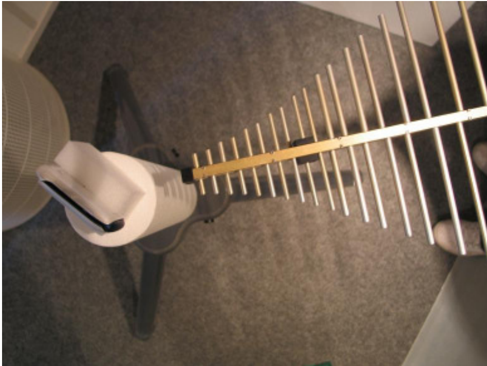
21868-1, IHDP56JJ1 Check for maximum radiation at position Y - Closed
