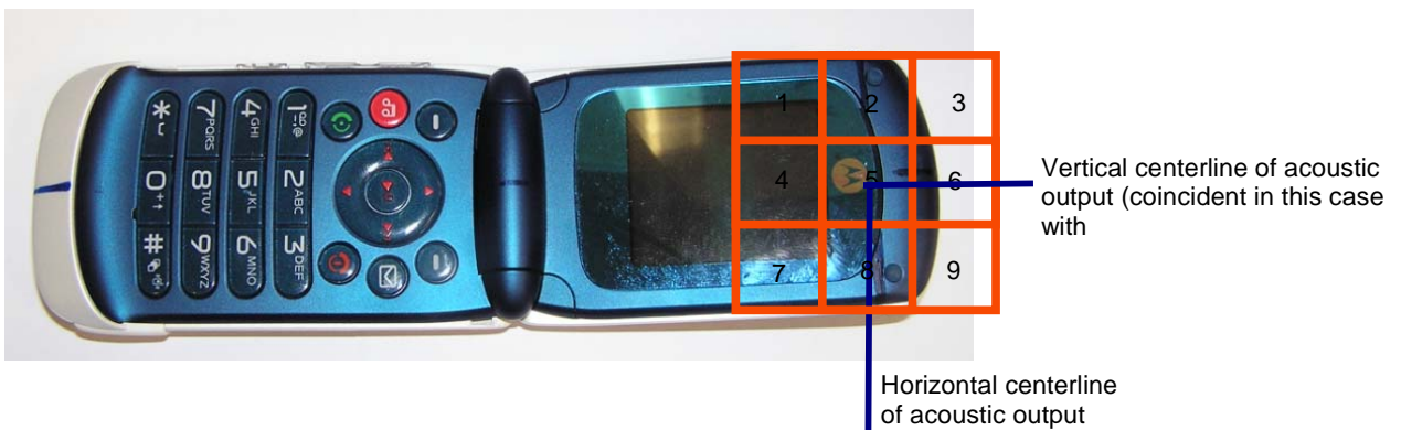
Figure 3. Phone Open – Orientation and Measurement Plane for RF Emission Testing
