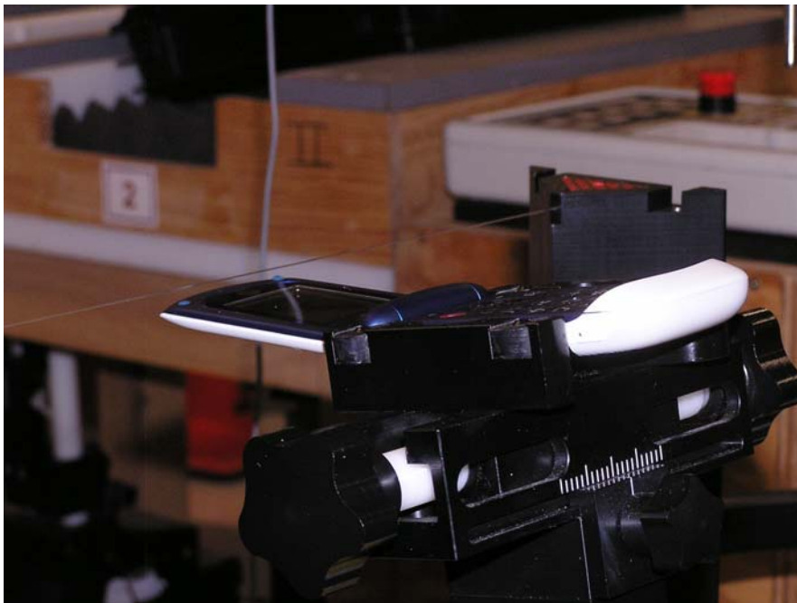
Figure 5. Measurement for RF Emissions
