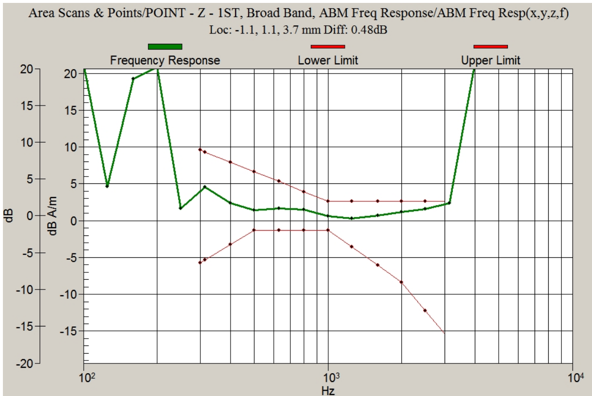
Graph 2: GSM 850 Frequency Response with Battery 1
