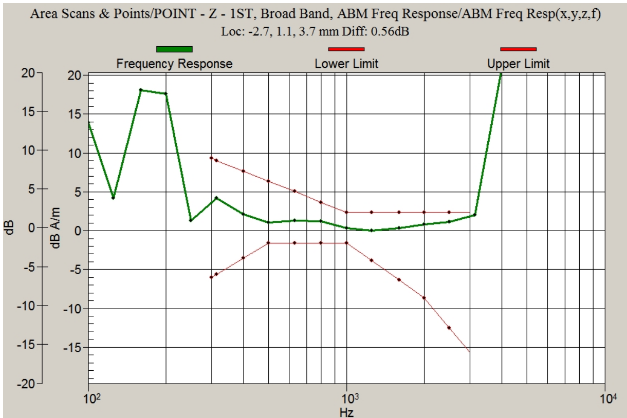
Graph 3: GSM 1900 Frequency Response with Battery 1
