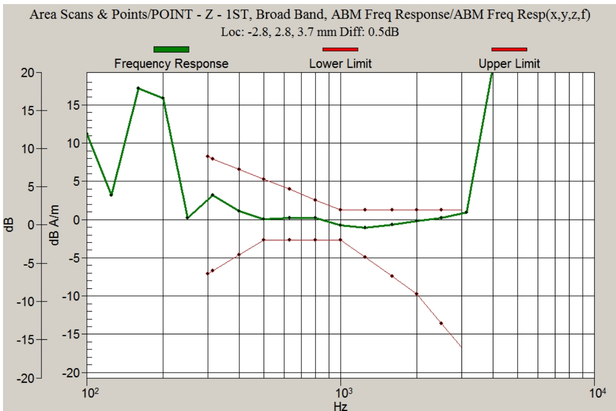
Graph 4: GSM 1900 Frequency Response with Battery 2
