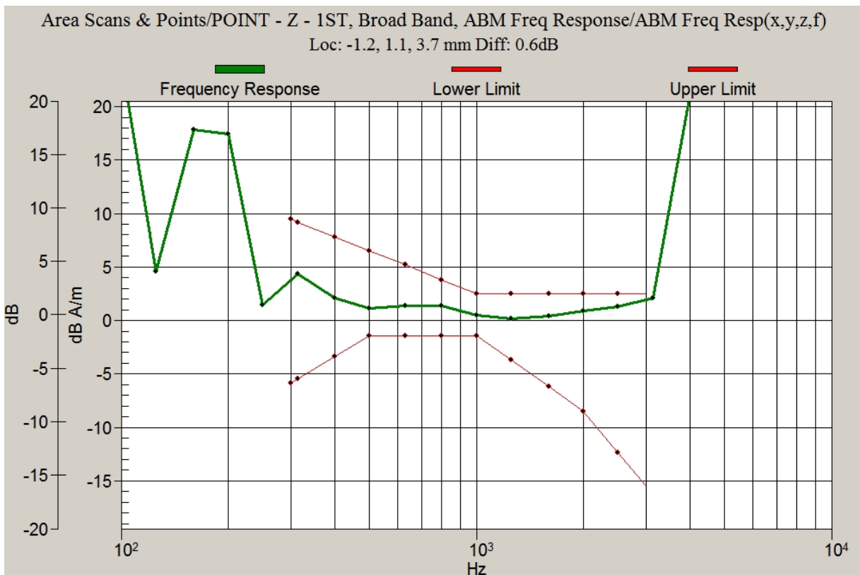
Graph 3: GSM 850 Frequency Response with Battery 2
