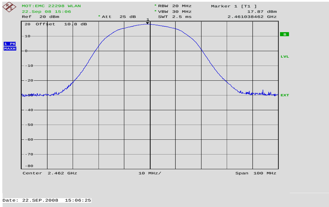
Max. Power Channel 11 @ 11 Mbps
