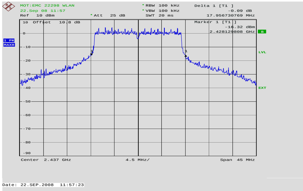
20dB Bandwidth Channel 6 @ 36 Mbps
