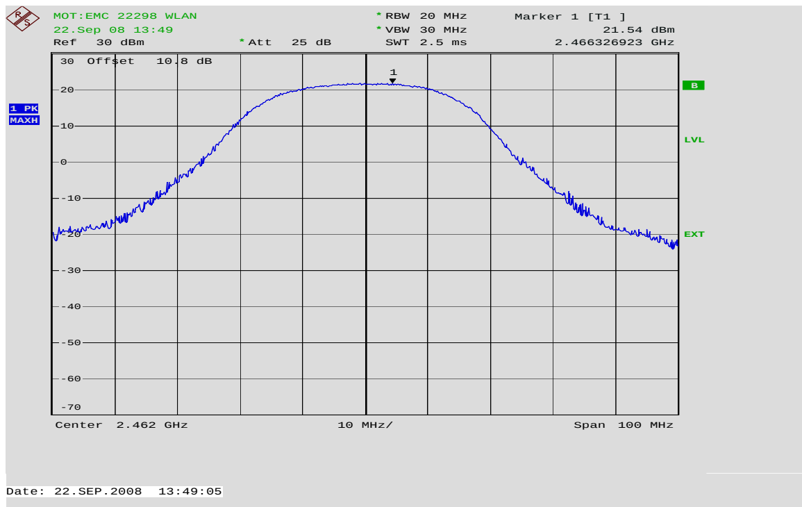
Max. Power Channel 11 @ 36 Mbps
