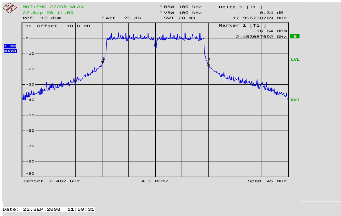
20dB Bandwidth Channel 11 @ 36 Mbps
