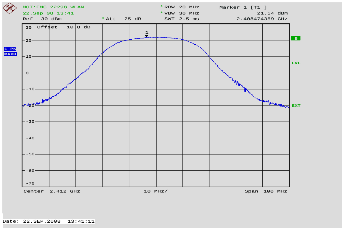
Max. Power Channel 1 @ 36 Mbps
