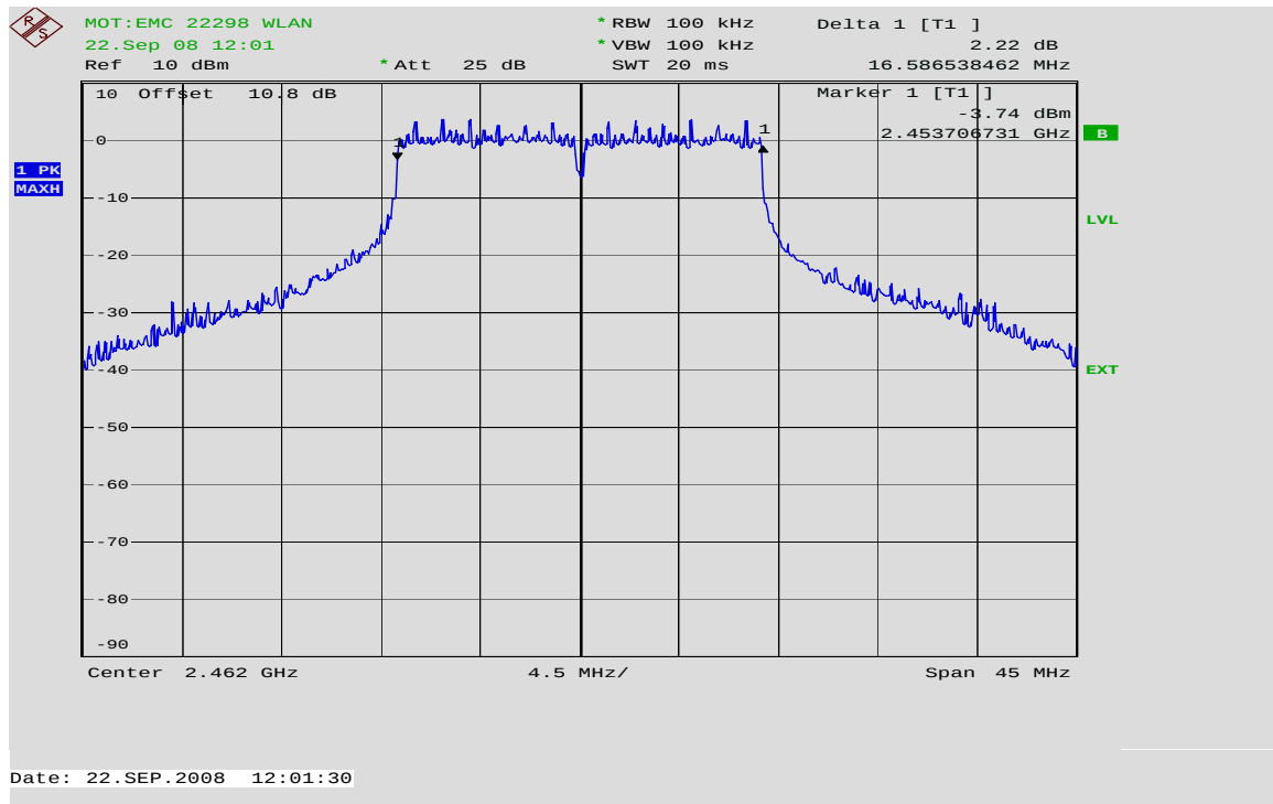
6dB Bandwidth Channel 11 @ 36 Mbps
