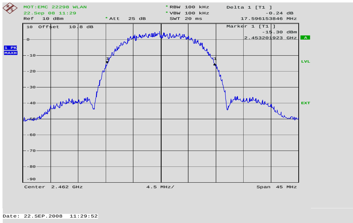
20dB Bandwidth Channel 11 @ 11 Mbps
