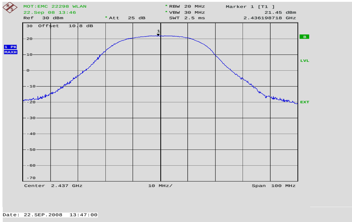
Max. Power Channel 6 @ 36 Mbps
