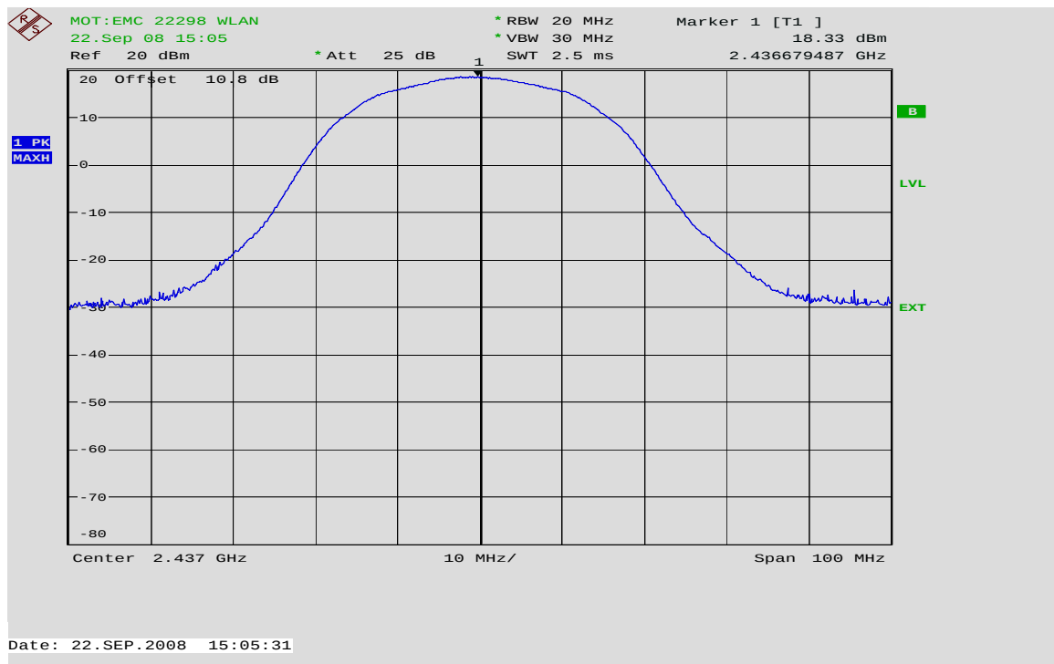
Max. Power Channel 6 @ 11 Mbps
