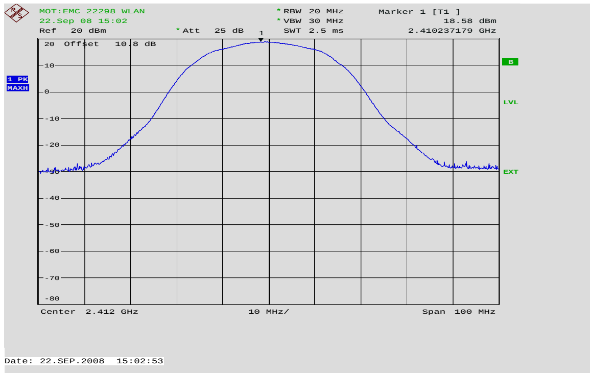
Max. Power Channel 1 @ 11 Mbps
