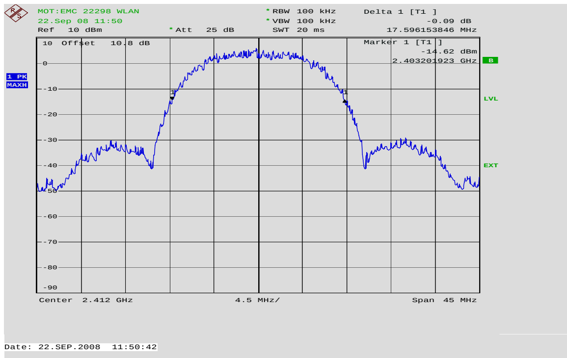
20dB Bandwidth Channel 1 @ 11 Mbps
