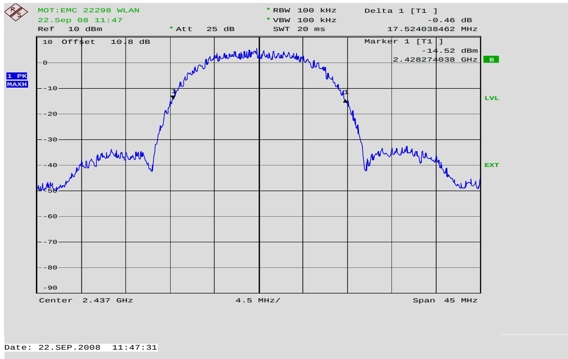
20dB Bandwidth Channel 6 @ 11 Mbps
