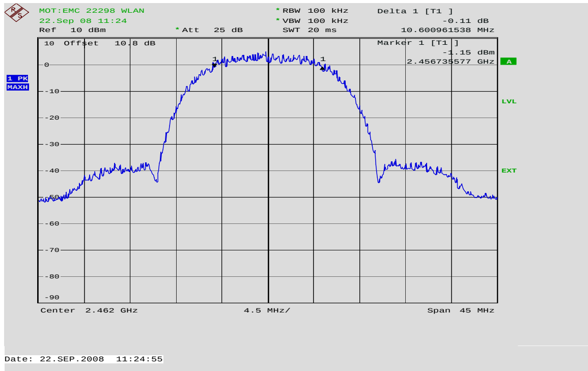
6dB Bandwidth Channel 11 @ 11 Mbps
