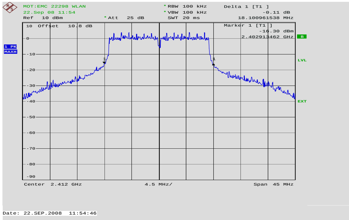
20dB Bandwidth Channel 1 @ 36 Mbps
