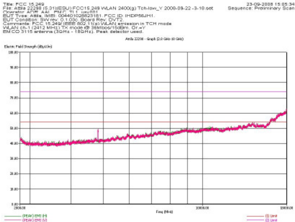
3-18GHz Low Channel, Dual Polarization, Y-Orientation
