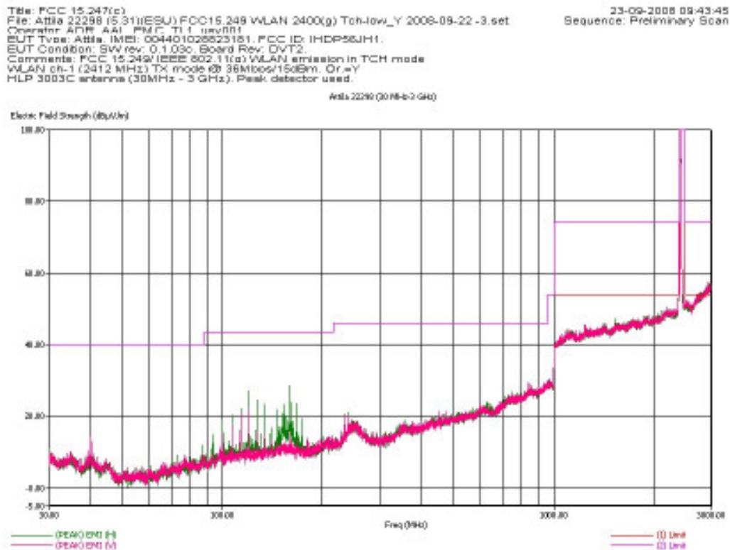
30 - 3000MHz Low Channel, Dual Polarization, Y
