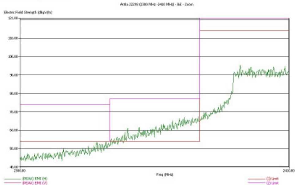
Band Edge Low Channel, X-Orientation, RBW = 100 kHz (6 dB)
