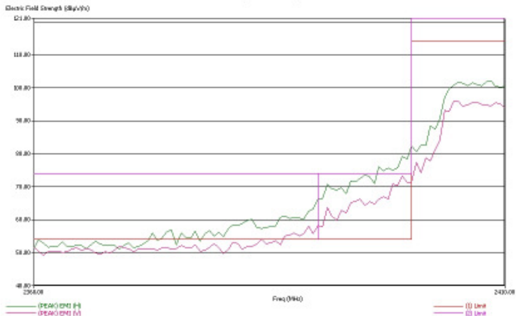
Low Band Edge Z-Orientation – Restricted band performance, PK (Peak detector and vertical limit line at 2390 MHz)
