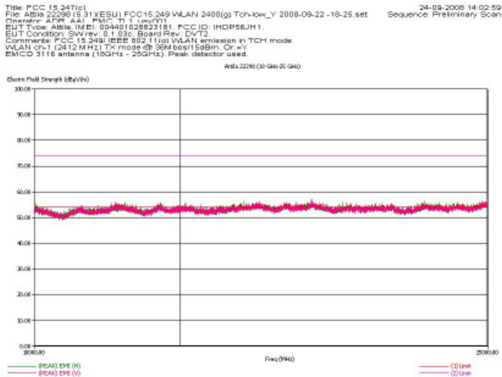
18-25 GHz Low Channel, Dual Polarization, Y-Orientation
