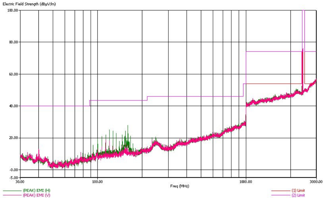
30-3000 MHz Low Channel, Dual Polarization, X
