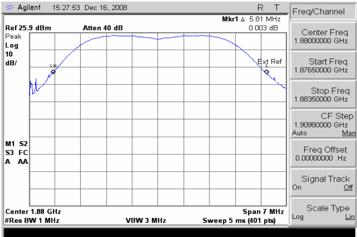
WCDMA 1900 – Channel 9400 (1880.00 MHz) – Occupied Bandwidth
