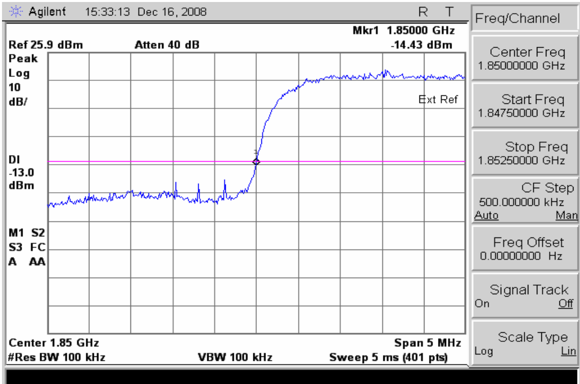
WCDMA 1900 – Lower Band Edge – Channel 9262 (1852.4 MHz)
