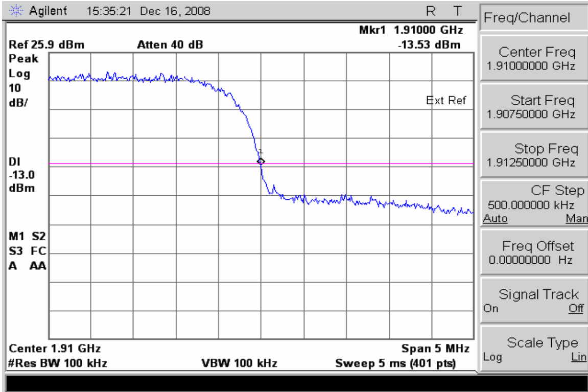
CDMA 1900 – Upper Band Edge – Channel 9538 (1907.6 MHz)
