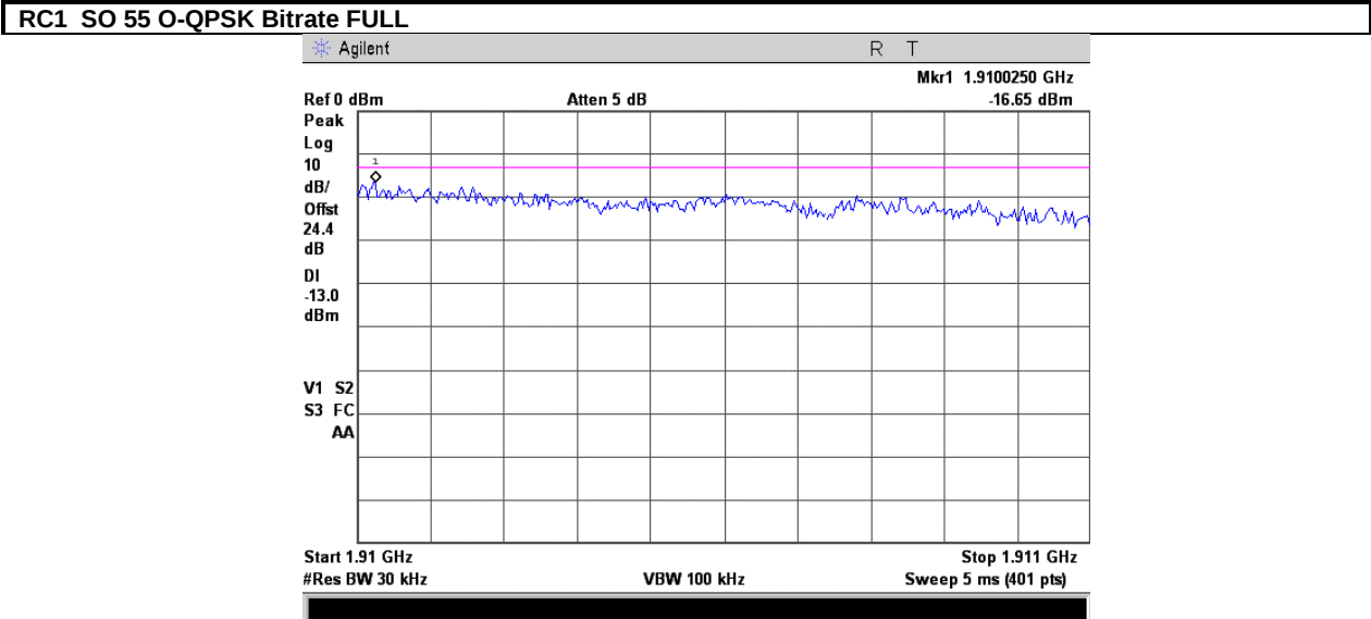
Plot 7.3.25 Spurious emission measurements in 1910 – 1911 MHz range at high carrier frequency
