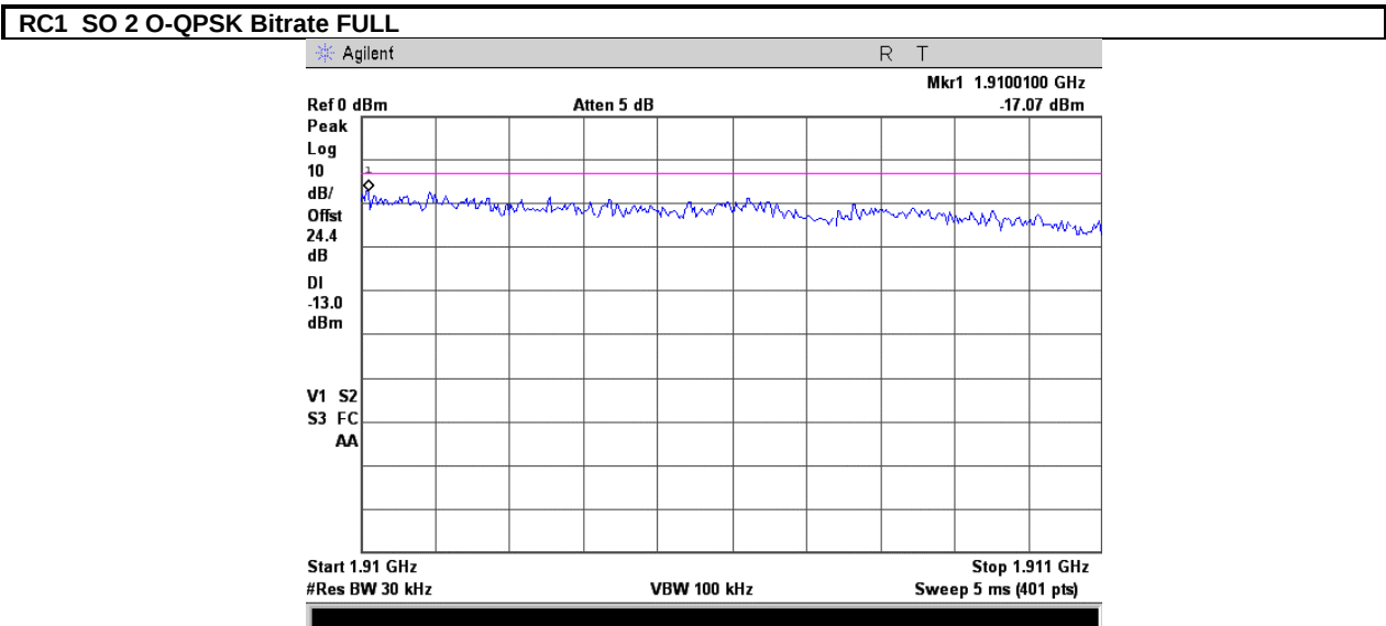
Plot 7.3.26 Spurious emission measurements in 1910 – 1911 MHz range at high carrier frequency
