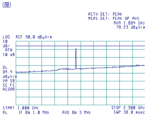
Plot 7.4.12 Radiated emission measurements in 1000 – 2900 MHz range
