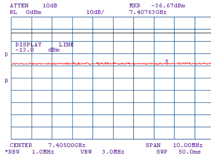
Plot 7.3.37 Conducted spurious emission measurements at the 4 th harmonic of low carrier frequency
