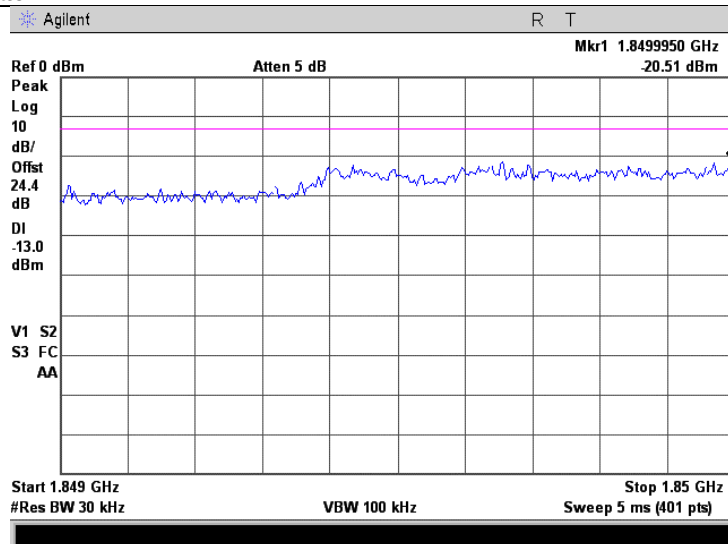
Plot 7.3.13 Spurious emission measurements in 1849 -1850 MHz range at low carrier frequency
