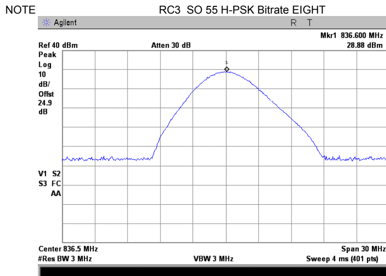
Plot 7.1.8 RF power output test results at mid frequency
