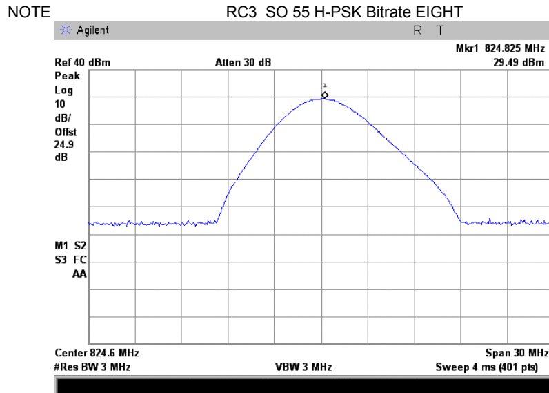
Plot 7.1.7 RF power output test results at low frequency
