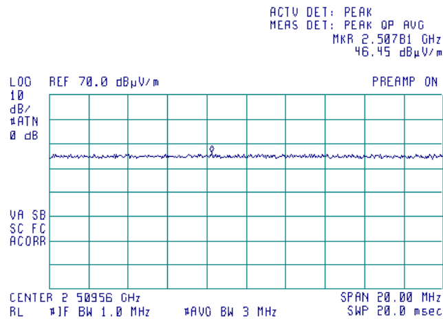
Plot 7.4.21 Radiated emission measurements at the 3 rd harmonic
