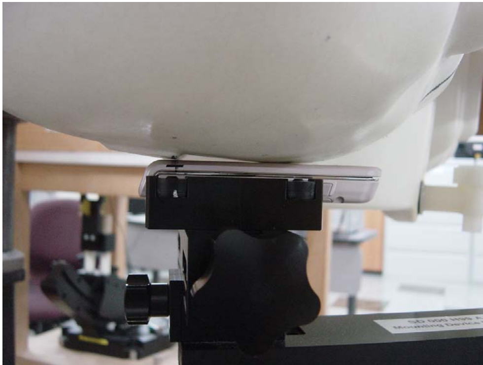
Figure5: Phone Against the Head Phantom (Cheek Touch – Slider Closed)
