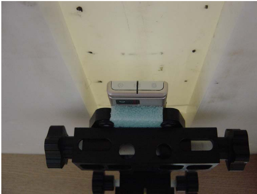
Figure9: Phone Against the Flat Phantom
