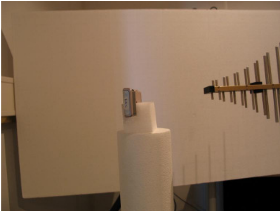
21780-1, IHDP56JD1 Maximum radiation position Y - Open
