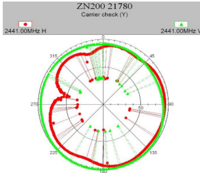
21780-1, IHDP56JD1 Maximum radiation pattern position Y - Open
