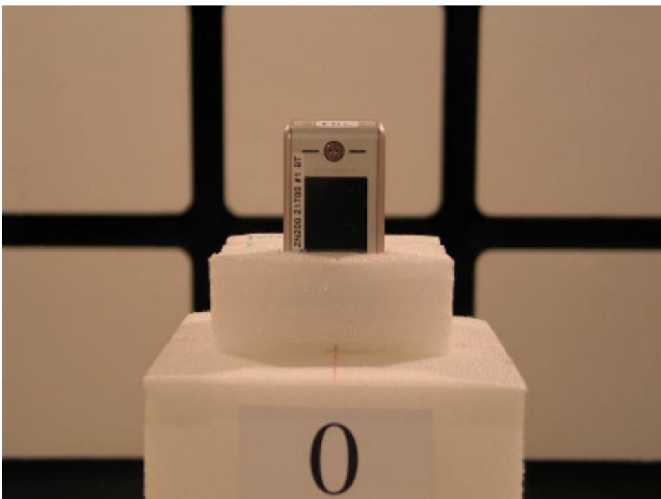
21780-1, IHDP56JD1 placed in test position Z - Closed
