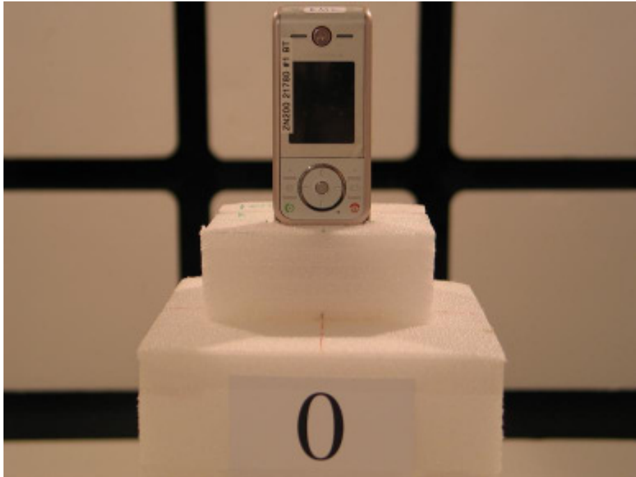
21780-1, IHDP56JD1 placed in test position Z - Open
