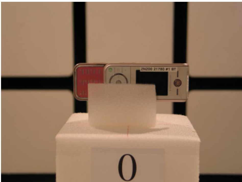
21780-1, IHDP56JD1 placed in test position Y - Open
