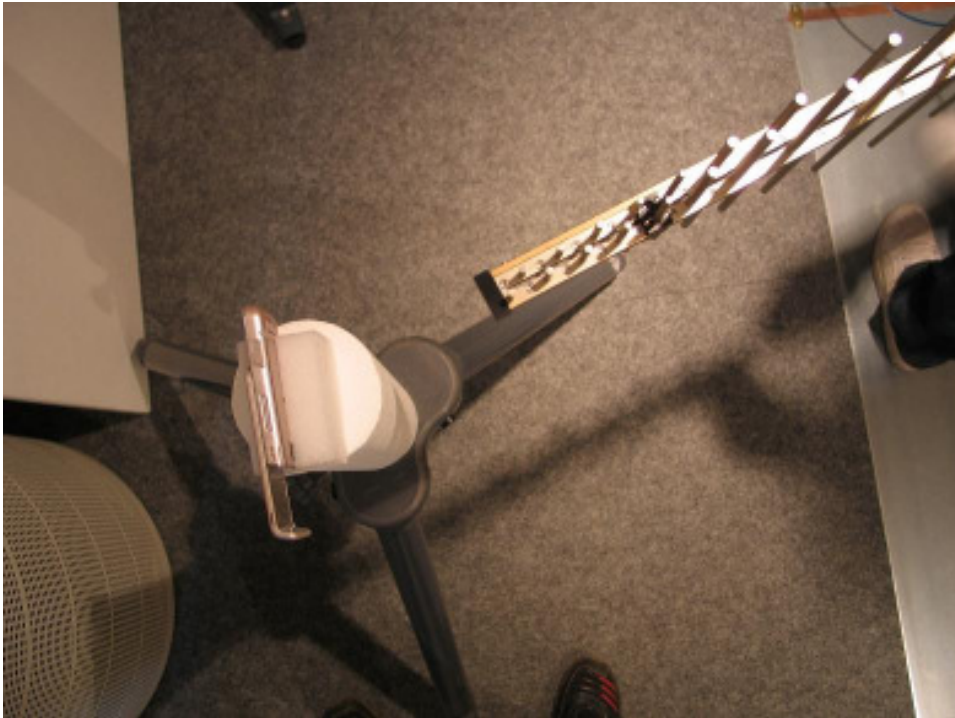
21780-1, IHDP56JD1 Check for maximum radiation at position Y - Open
