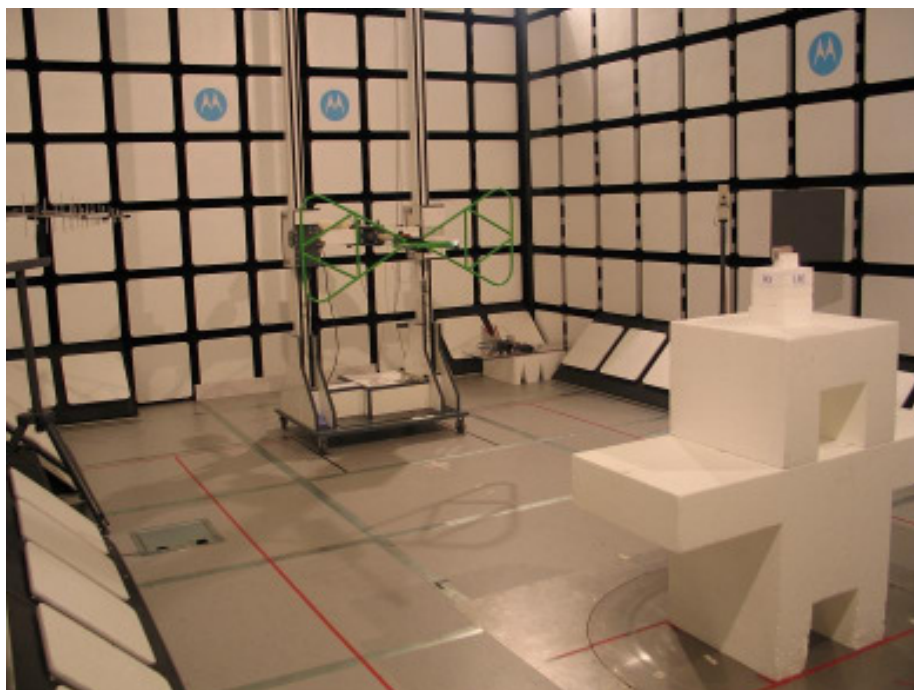
21780-1, IHDP56JD1 setup in semi-anechoic chamber – front view
