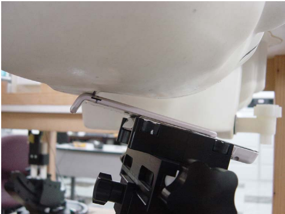
Figure8: Phone Against the Head Phantom (15° Tilt - Slider Open)
