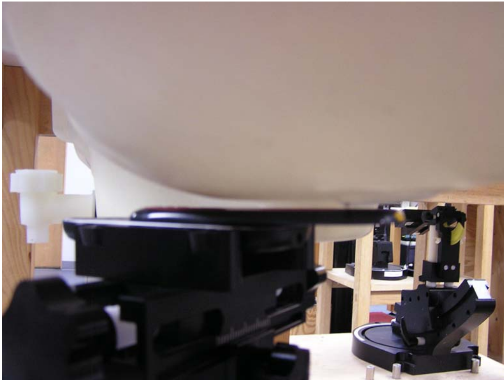
Figure 5 - Transceiver against head, Cheek Touch position – Slider Open
