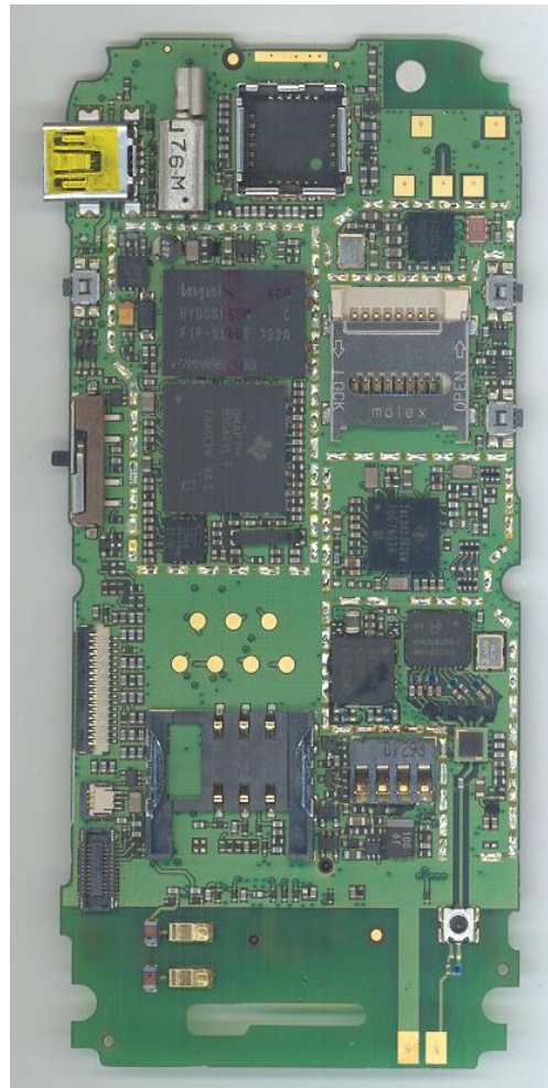
Main Board Top Without Shields
