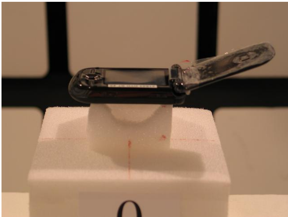
21624-1, IHDP56HT1 placed in test position X - Open
