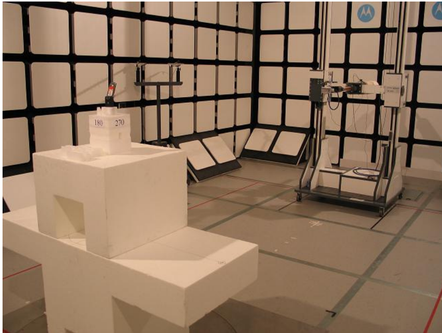
21624-1, IHDP56HT1 setup in semi-anechoic chamber – front view
