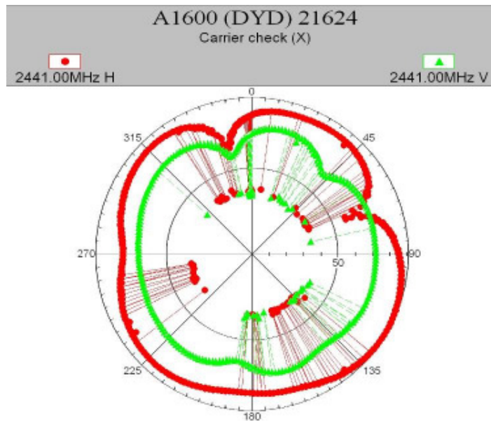
21624-1, IHDP56HT1 maximum radiation pattern position X - Open
