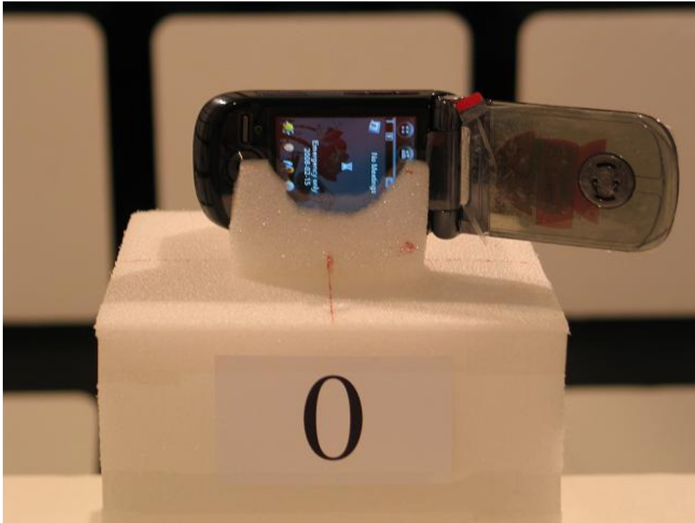
21624-1, IHDP56HT1 placed in test position Y - Open
