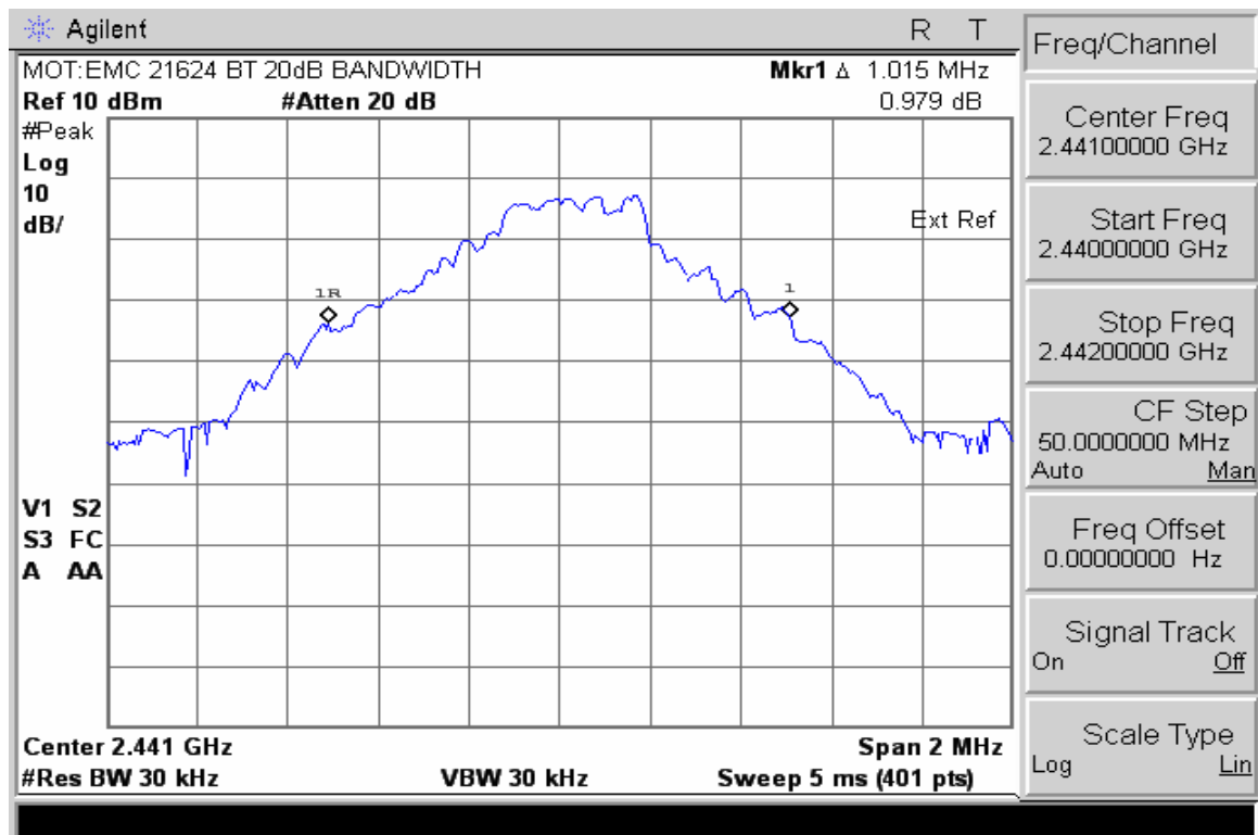
20dB Bandwidth
