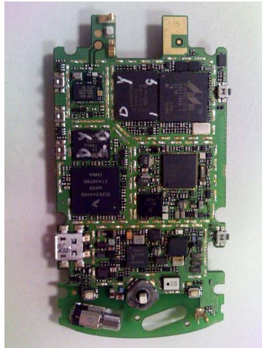
Main Board Bottom Without Shields
