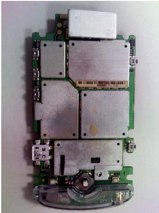
Main Board Bottom With Shields
