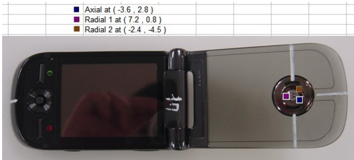
Figure 5. Location of Measured Points for T-coil measurements
