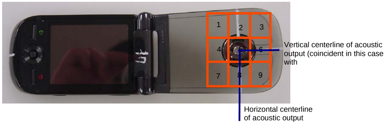
Figure 3. Phone Open - Orientation and Measurement Plane for RF Emissions Testing
