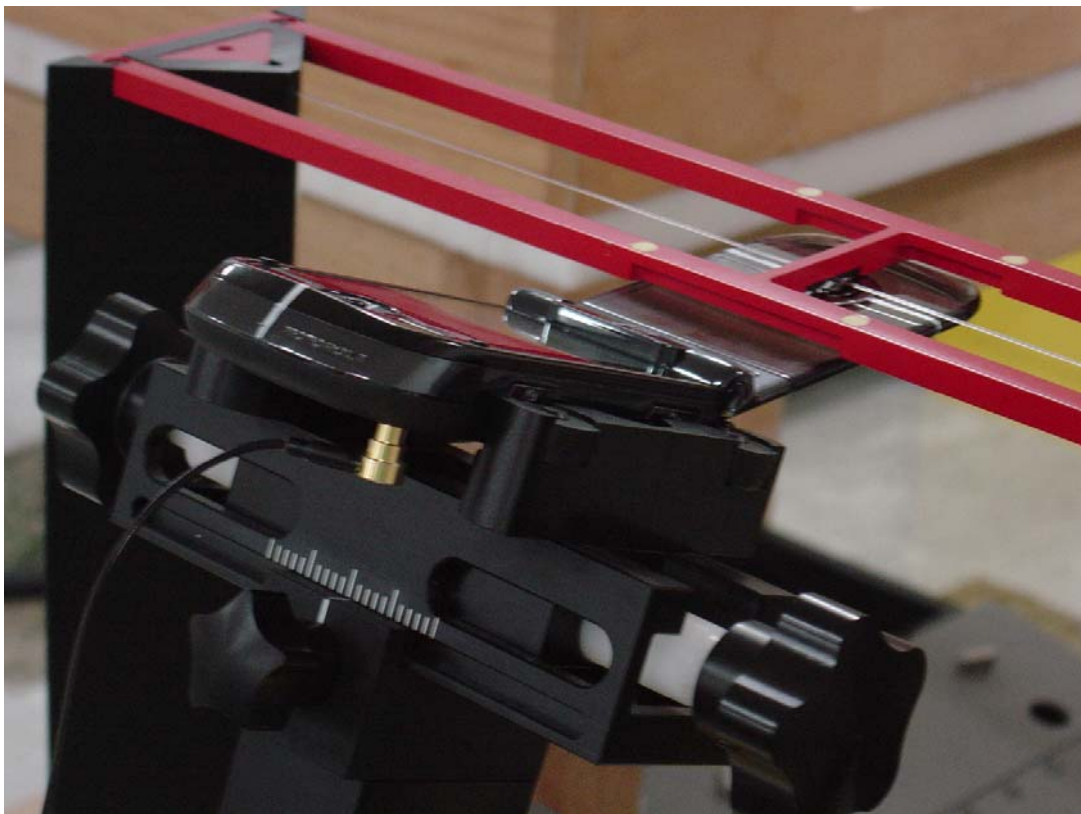
Figure 6. Positioning and Measurement for T-coil
