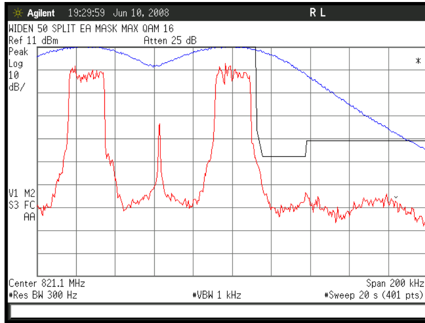
Figure 6a-2.7.3. WiDEN50 Split 800 MHz Band, QAM16, Maximum Power, EA Emission Mask
