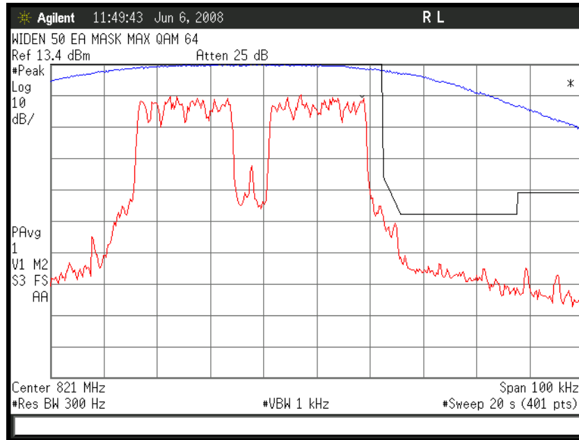
Figure 6a-2.4.5. WiDEN50 800 MHz Band, Continuous QAM64, Maximum Power, EA Emission Mask
