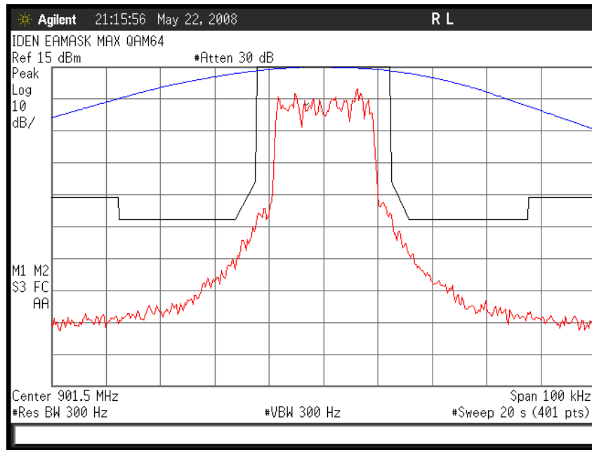
Figure 6b.2.1.3. iDEN NBPCS Band, Quad- 64QAM; Occupied Bandwidth
