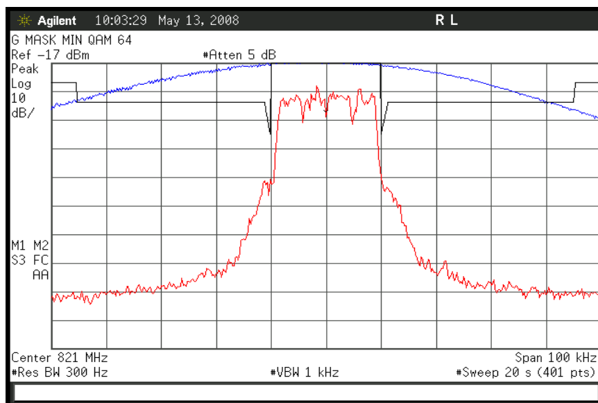
Figure 6a-2.1.10. iDEN 800 MHz Band, QAM64, Minimum Power, Emission Mask G
