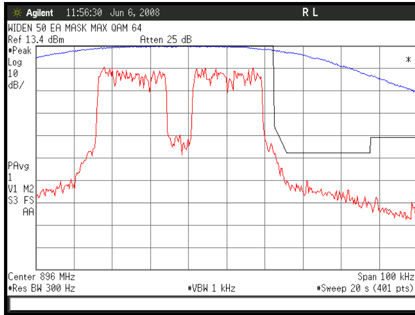
Figure 6a-2.9.5. WiDEN50 900 MHz Band, Continuous QAM64, Maximum Power, EA Emission Mask
