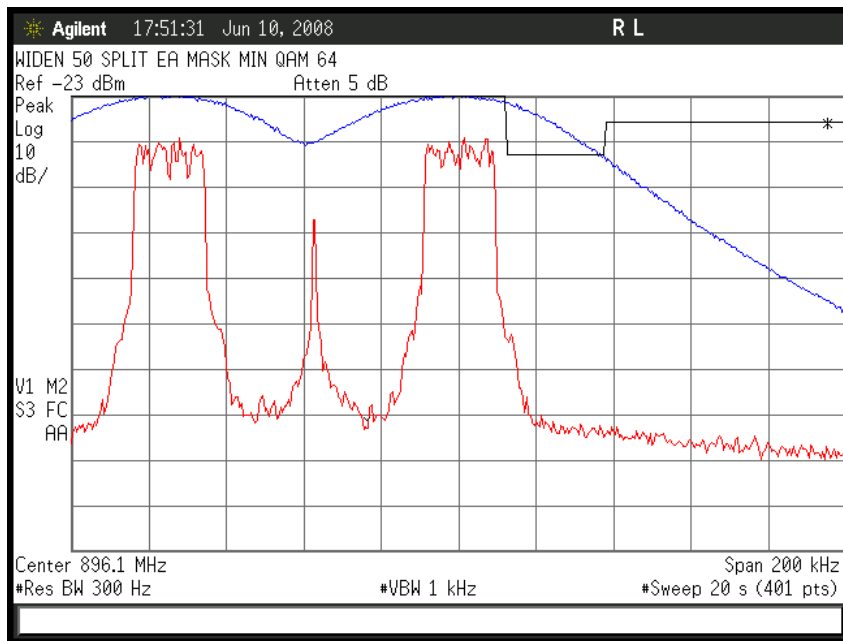
Figure 6a-2.12.6. WiDEN50 Split 900 MHz Band, QAM64, Minimum Power, EA Emission Mask
