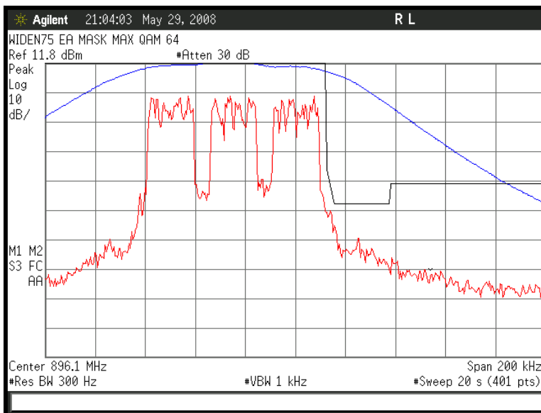
Figure 6a-2.10.5. WiDEN75 900 MHz Band, QAM64, Maximum Power, EA Emission Mask
