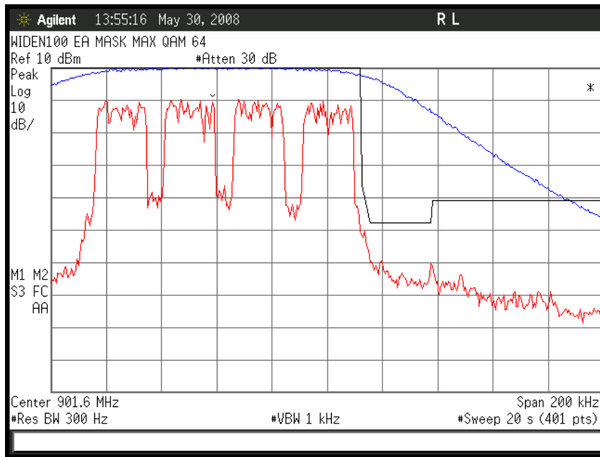
Figure 6b.2.5.3.15. WiDEN 100 NBPCS Band, Quad- 64 QAM; Occupied Bandwidth
