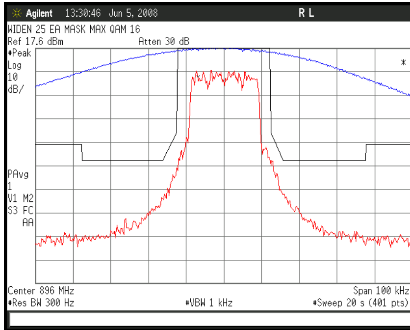
Figure 6a-2.8.7. WiDEN25 900 MHz Band, QAM16, Maximum Power, EA Emission Mask
