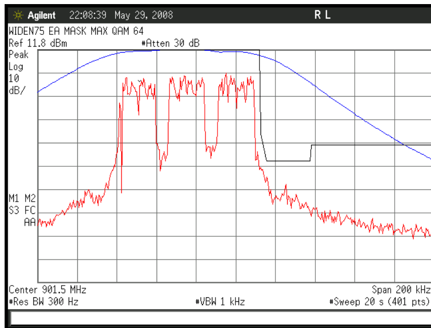
Figure 6b.2.4.3. WiDEN 75 NBPCS Band, Quad- 64 QAM; Occupied Bandwidth
