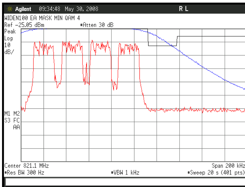
Figure 6a-2.6.2. WiDEN100 800 MHz Band, Quad-QPSK, Minimum Power, EA Emission Mask
