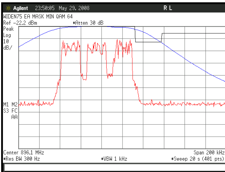
Figure 6a-2.10.6. WiDEN75 900 MHz Band, QAM64, Minimum Power, EA Emission Mask
