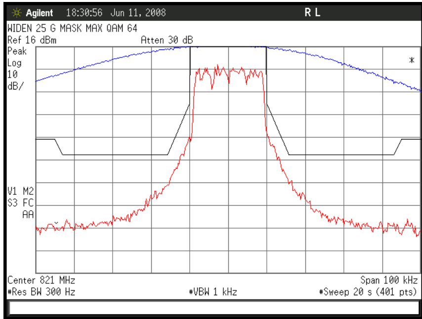
Figure 6a-2.3.9. WiDEN25 800 MHz Band, QAM64, Maximum Power, Emission Mask G
