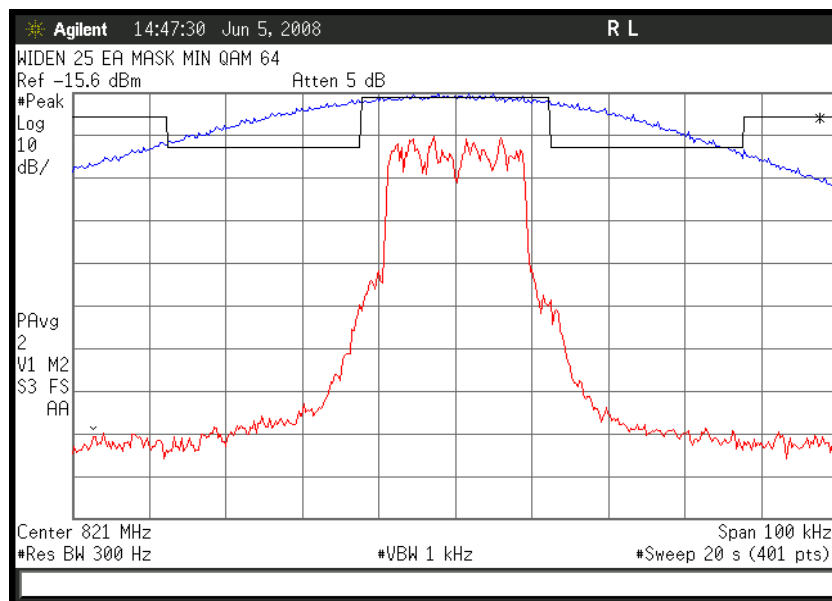
Figure 6a-2.3.12. WiDEN25 800 MHz Band, QAM64, Minimum Power, EA Emission Mask
