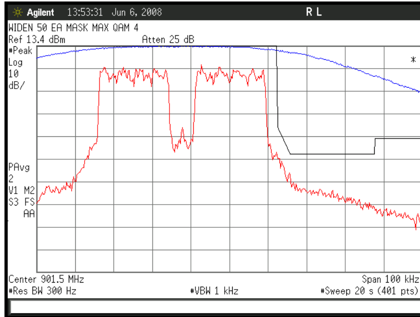
Figure 6b.2.3.1. WiDEN 50 NBPCS Band, QPSK; Occupied Bandwidth
