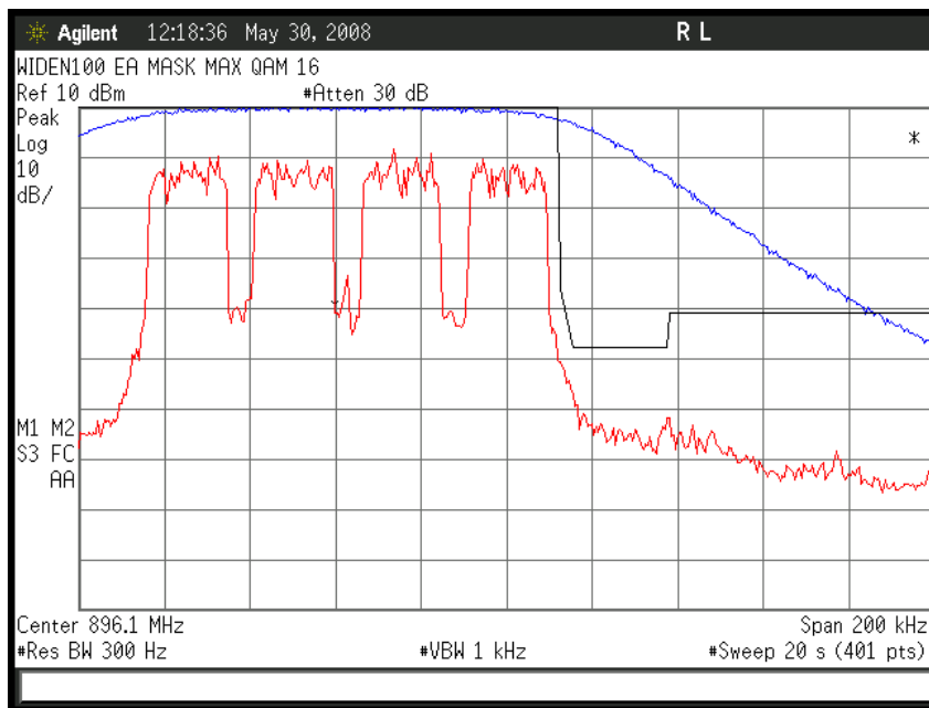
Figure 6a-2.11.3. WiDEN100 900 MHz Band, QAM16, Maximum Power, EA Emission Mask
