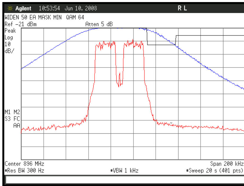
Figure 6a-2.9.6. WiDEN50 900 MHz Band, Continuous QAM64, Minimum Power, EA Emission Mask
