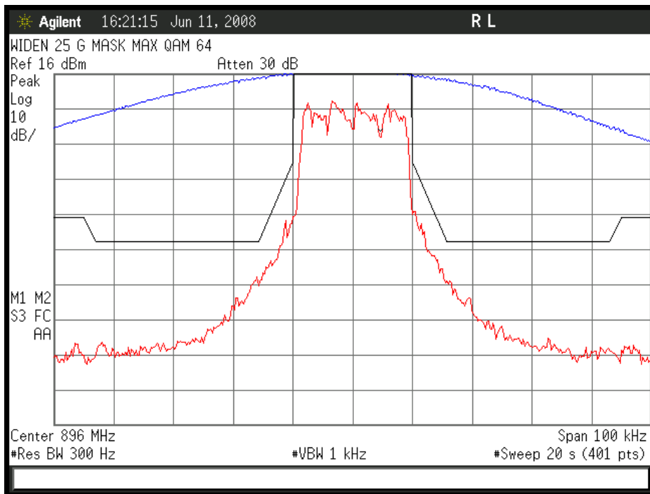
Figure 6a-2.8.9. WiDEN25 900 MHz Band, QAM64, Maximum Power, Emission Mask G
