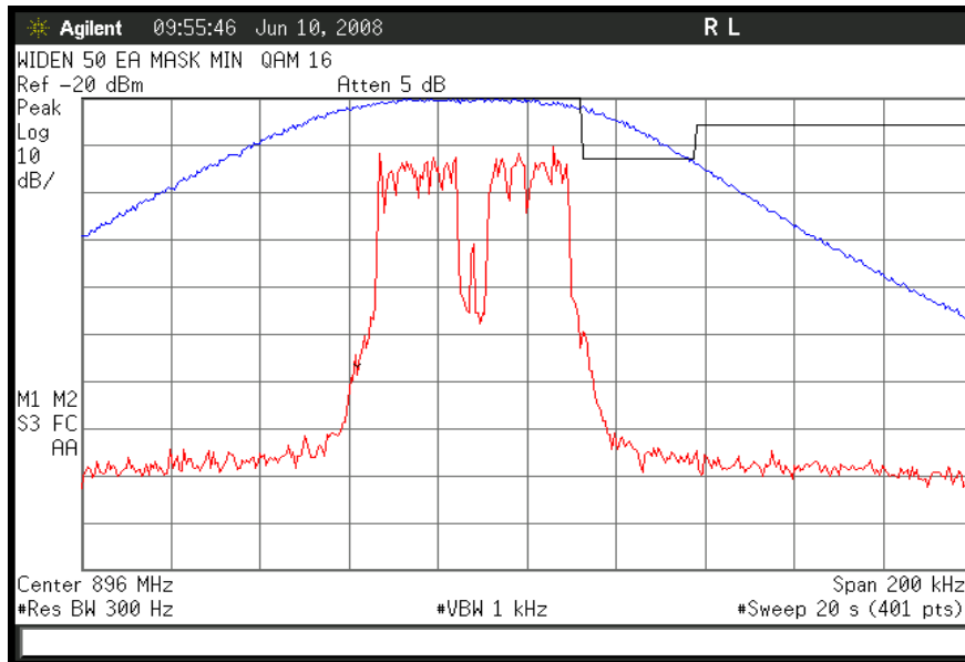
Figure 6a-2.9.4. WIDEN50 900 MHz Band, Continuous QAM16, Minimum Power, EA Emission Mask
