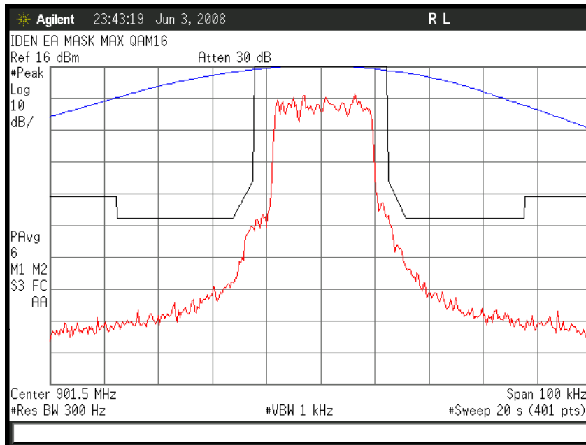
Figure 6b.2.1.2. iDEN NBPCS Band, Quad-16QAM; Occupied Bandwidth
