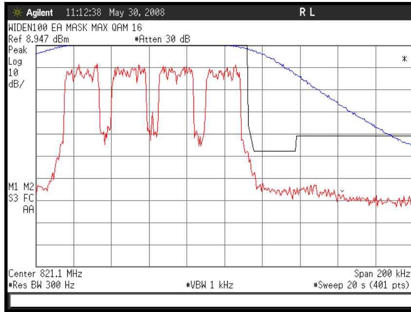
Figure 6a-2.6.3. WiDEN100 800 MHz Band, QAM16, Maximum Power, EA Emission Mask
