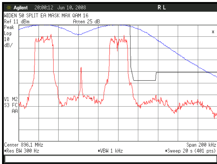
Figure 6a-2.12.3. WiDEN50 Split 900 MHz Band, QAM16, Maximum Power, EA Emission Mask
