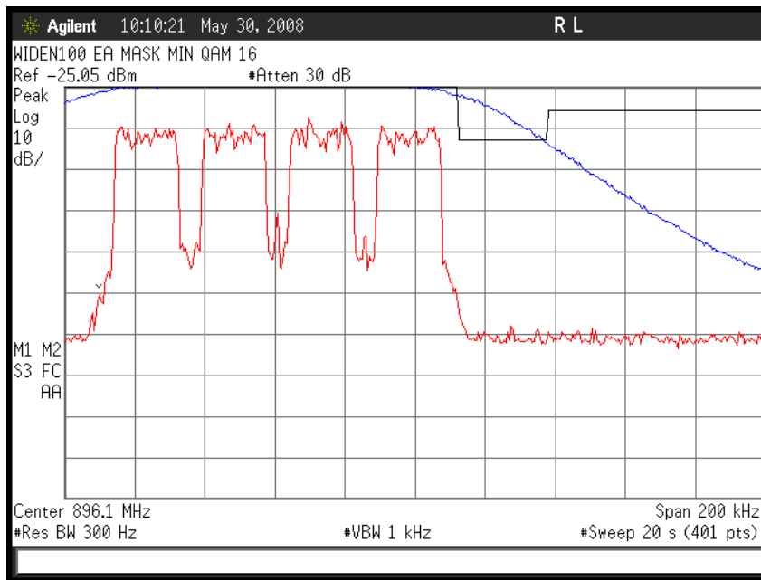
Figure 6a-2.11.4. WiDEN100 900 MHz Band, QAM16, Minimum Power, EA Emission Mask
