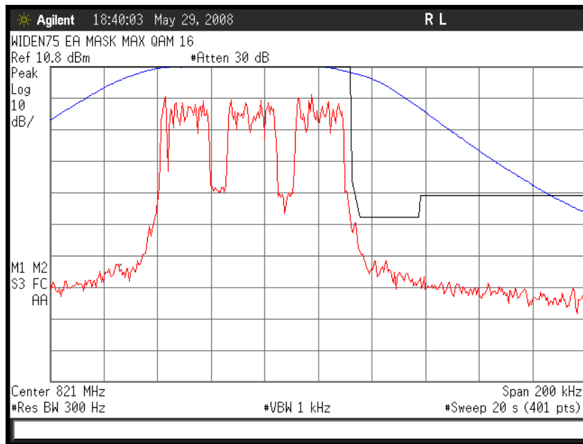
Figure 6a-2.5.3. WIDEN75 800 MHz Band, QAM16, Maximum Power, EA Emission Mask
