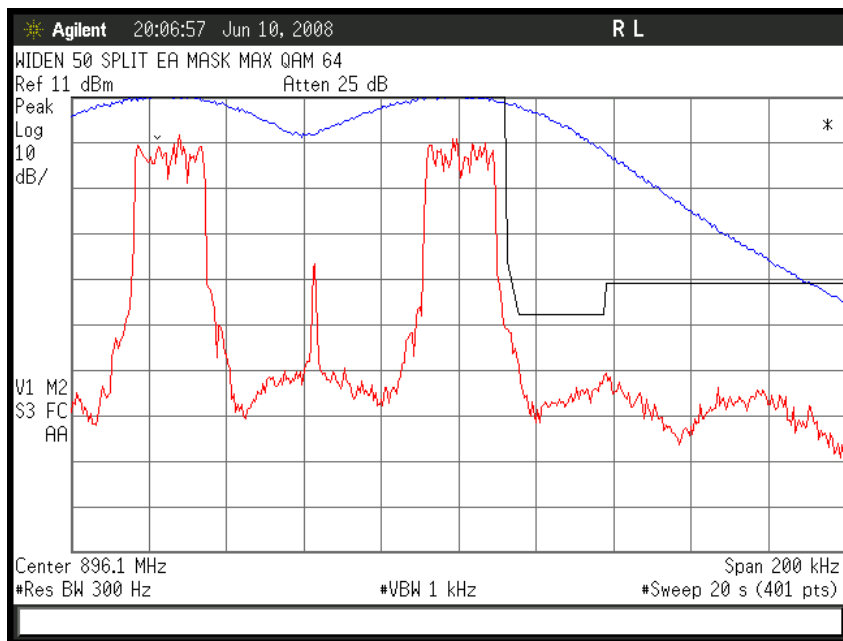
Figure 6a-2.12.5. WiDEN50 Split 900 MHz Band, QAM64, Maximum Power, EA Emission Mask
