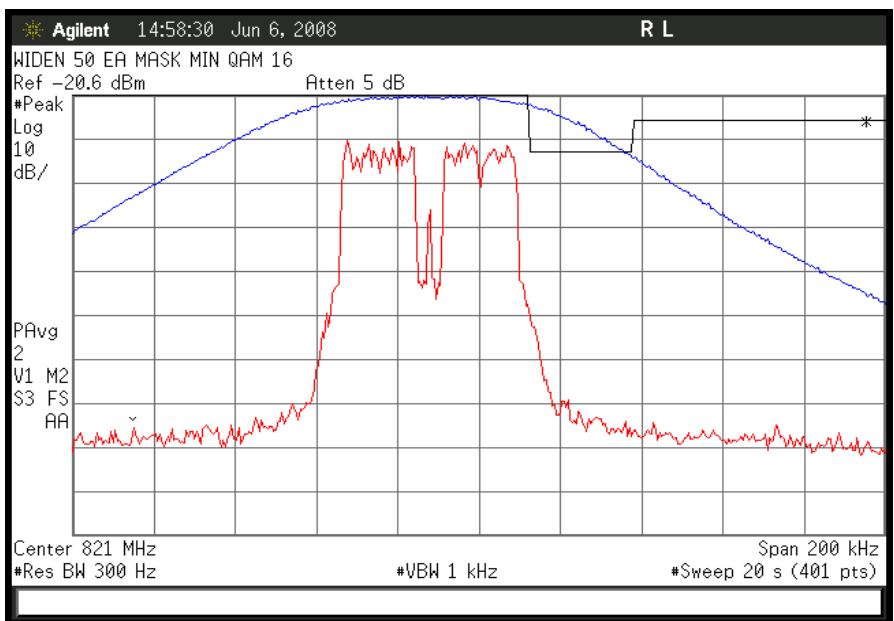
Figure 6a-2.4.4. WiDEN50 800 MHz Band, Continuous QAM16, Minimum Power, EA Emission Mask
