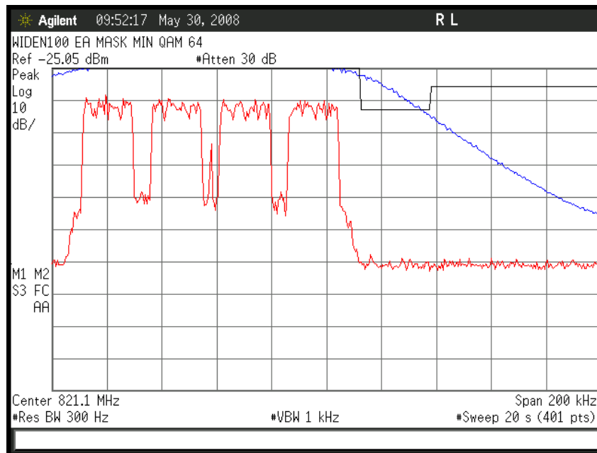
Figure 6a-2.6.6. WiDEN100 800 MHz Band, QAM64, Minimum Power, EA Emission Mask
