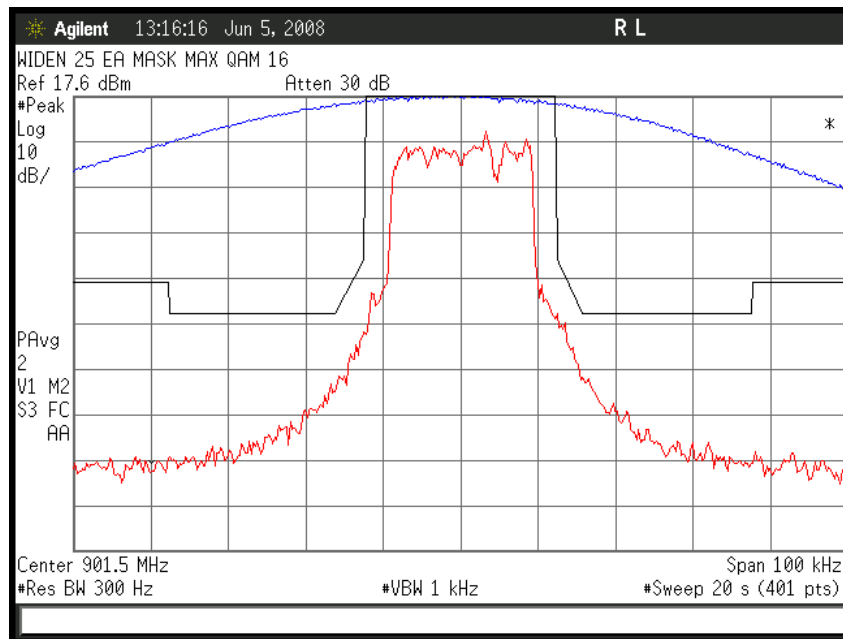
Figure 6b.2.2.2. WIDEN 25 NBPCS Band, Quad- 16 QAM; Occupied Bandwidth
