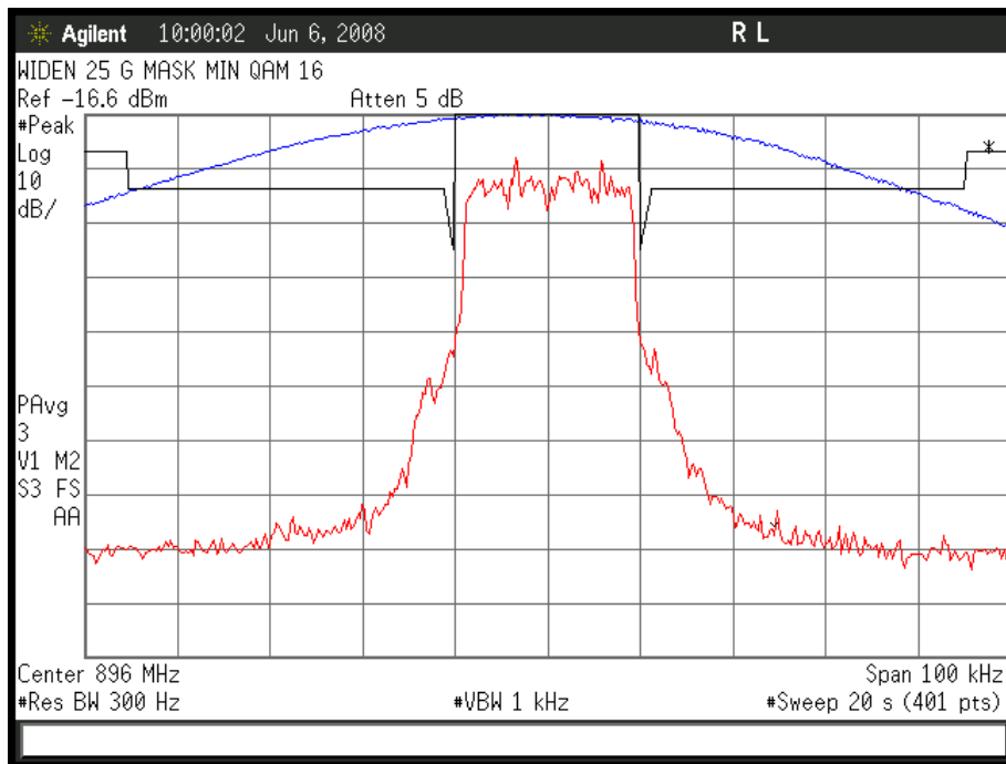
Figure 6a-2.8.6. WiDEN25 900 MHz Band, QAM16, Minimum Power, Emission Mask G
