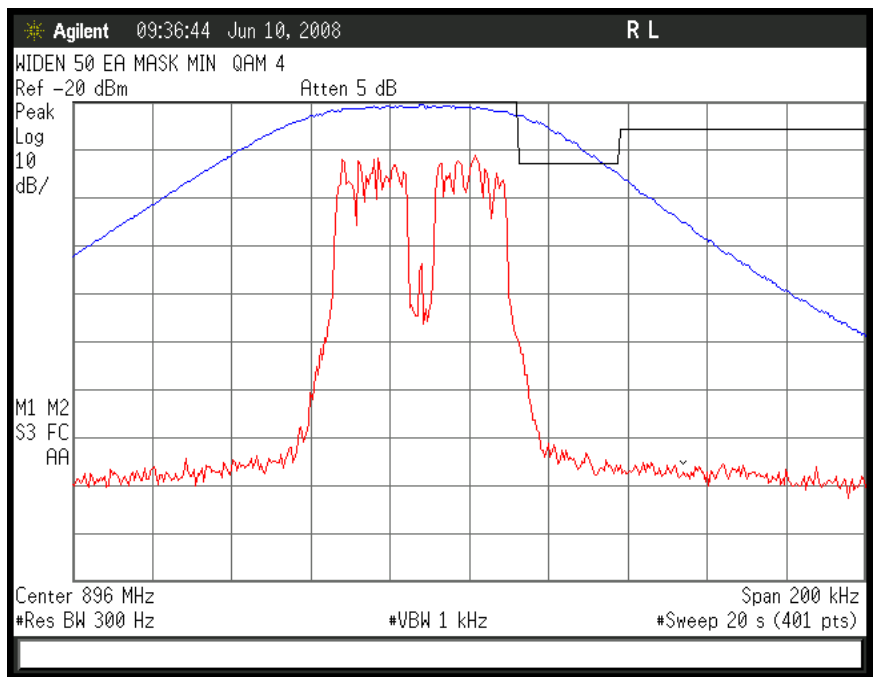
Figure 6a-2.9.2. WiDEN50 900 MHz Band, Continuous Quad-QPSK, Minimum Power, EA Emission Mask
