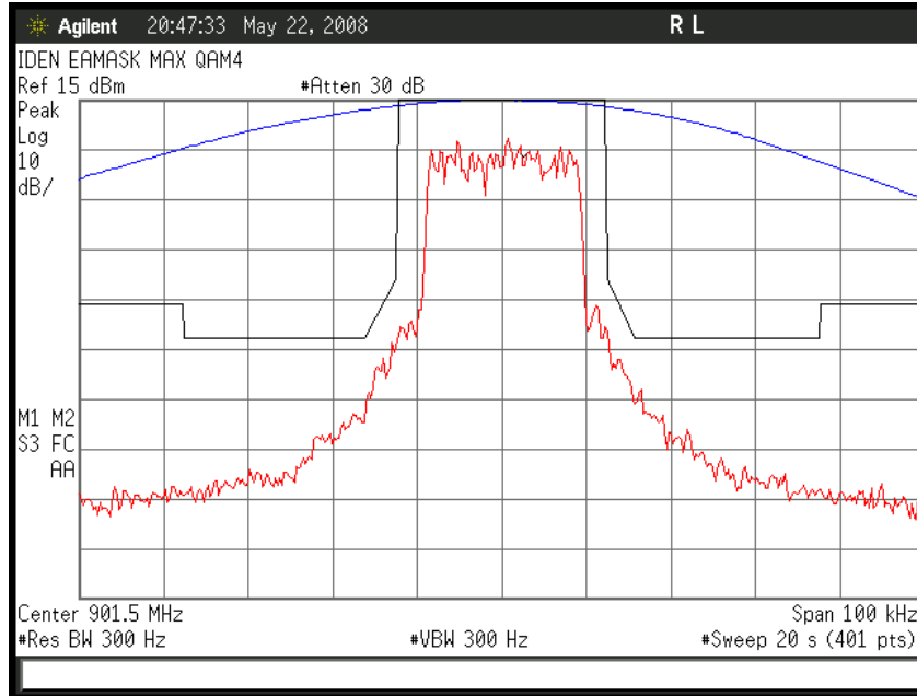
Figure 6b.2.1.1 iDEN NBPCS Band, QPSK; Occupied Bandwidth.
