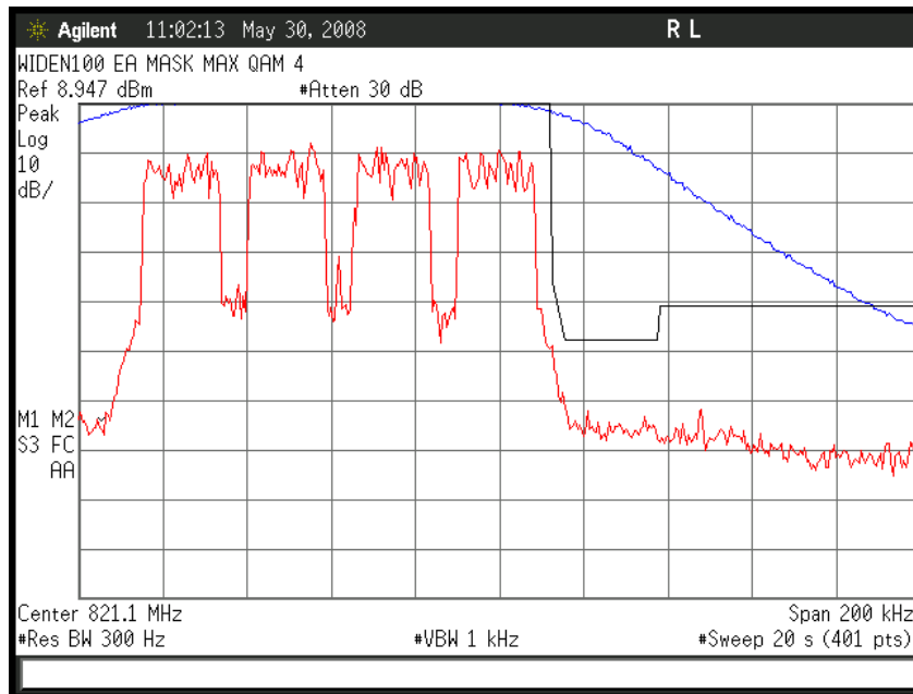
Figure 6a-2.6.1. WiDEN100 800 MHz Band, Quad-QPSK, Maximum Power, EA Emission Mask
