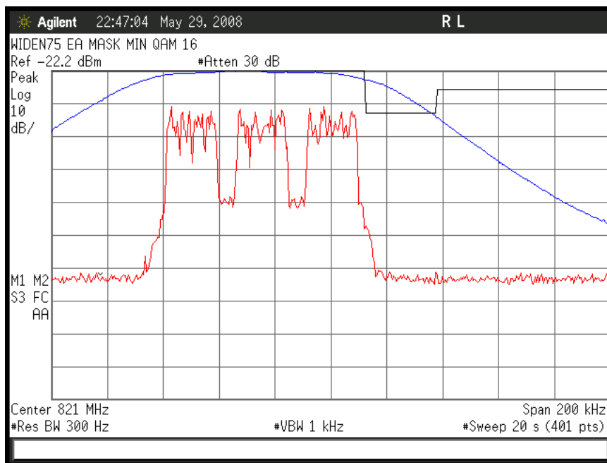
Figure 6a-2.5.4. WIDEN75 800 MHz Band, QAM16, Minimum Power, EA Emission Mask
