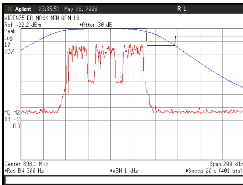
Figure 6a-2.10.4. WIDEN75 900 MHz Band, QAM16, Minimum Power, EA Emission Mask
