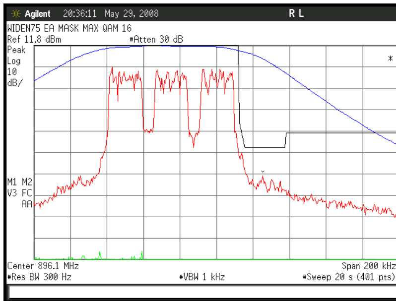
Figure 6a-2.10.3. WIDEN75 900 MHz Band, QAM16, Maximum Power, EA Emission Mask
