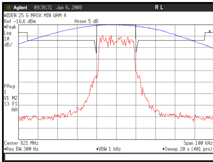
Figure 6a-2.3.2. WiDEN25 800 MHz Band, Quad-QPSK, Minimum Power, Emission Mask G
