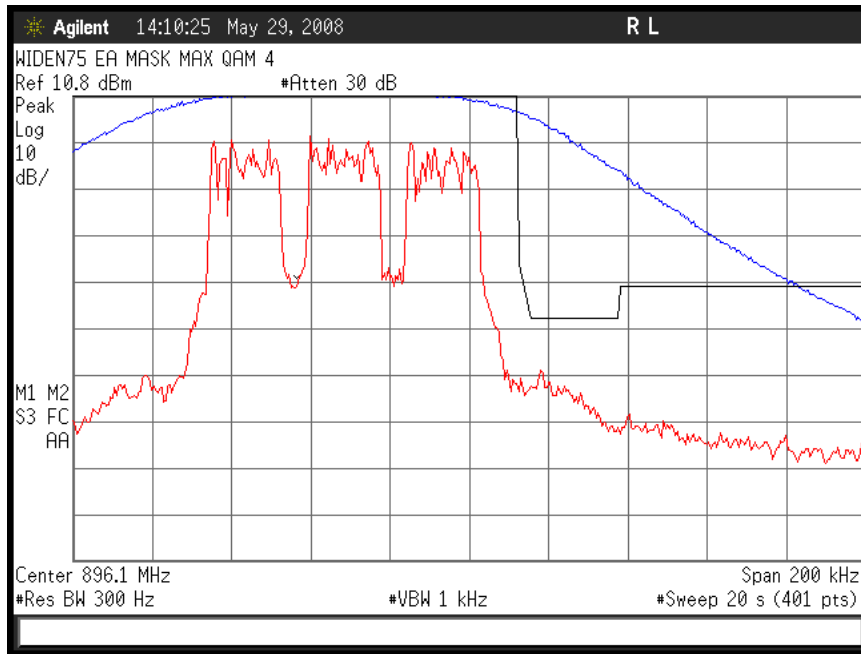
Figure 6a-2.10.1. WiDEN75 900 MHz Band, Quad-QPSK, Maximum Power, EA Emission Mask
