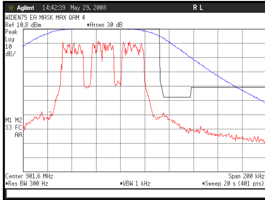
Figure 6b.2.4.1. WiDEN 75 NBPCS MHz Band, QPSK; Occupied Bandwidth
