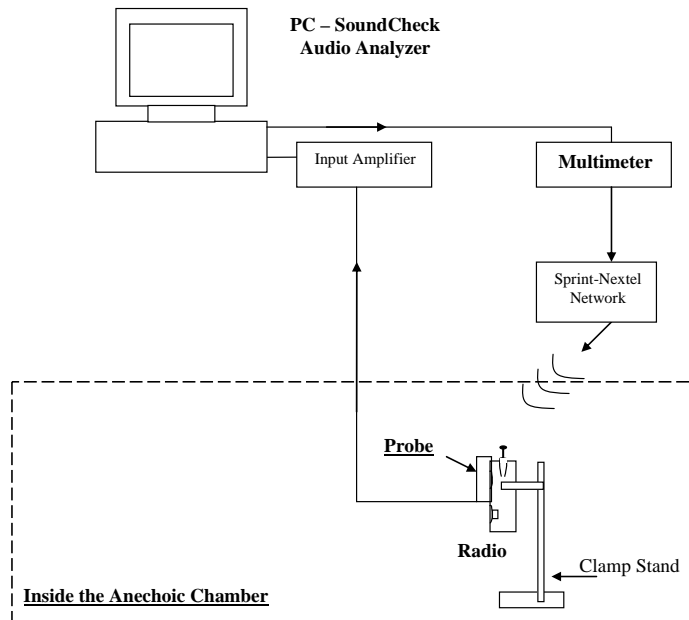
Figure 5-1 – Test setup
