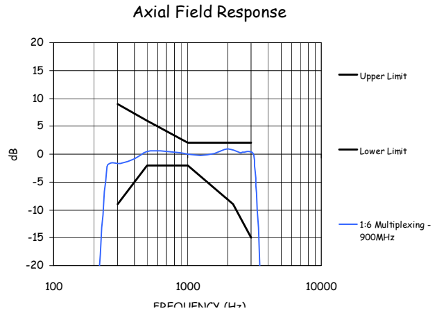
Figure 9-1-4: 900 MHz Measured Frequency Response (1:6).
