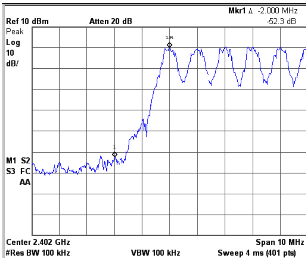
Figure 6c.6-3: Plot of lower band-edge conducted emissions with hopping enabled.
