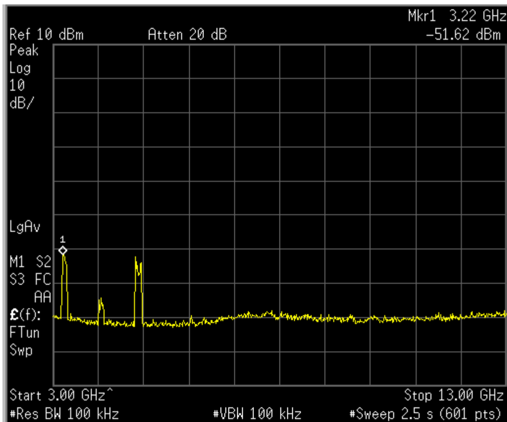
Figure 6c.7-2: Plot of spurious conducted emissions 3 GHz – 13 GHz.
