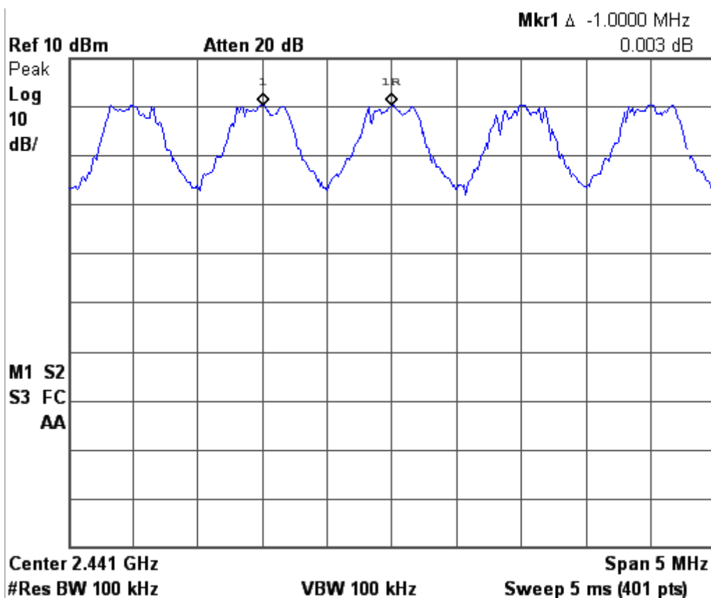
Figure 6c.1-1: Plot of Bluetooth carrier frequency separation
