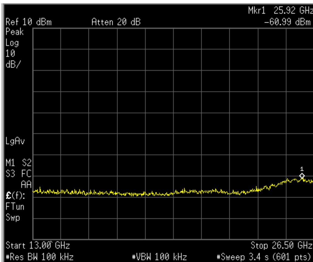
Figure 6c.7-3: Plot of spurious conducted emissions 13 GHz – 26.5 GHz.
