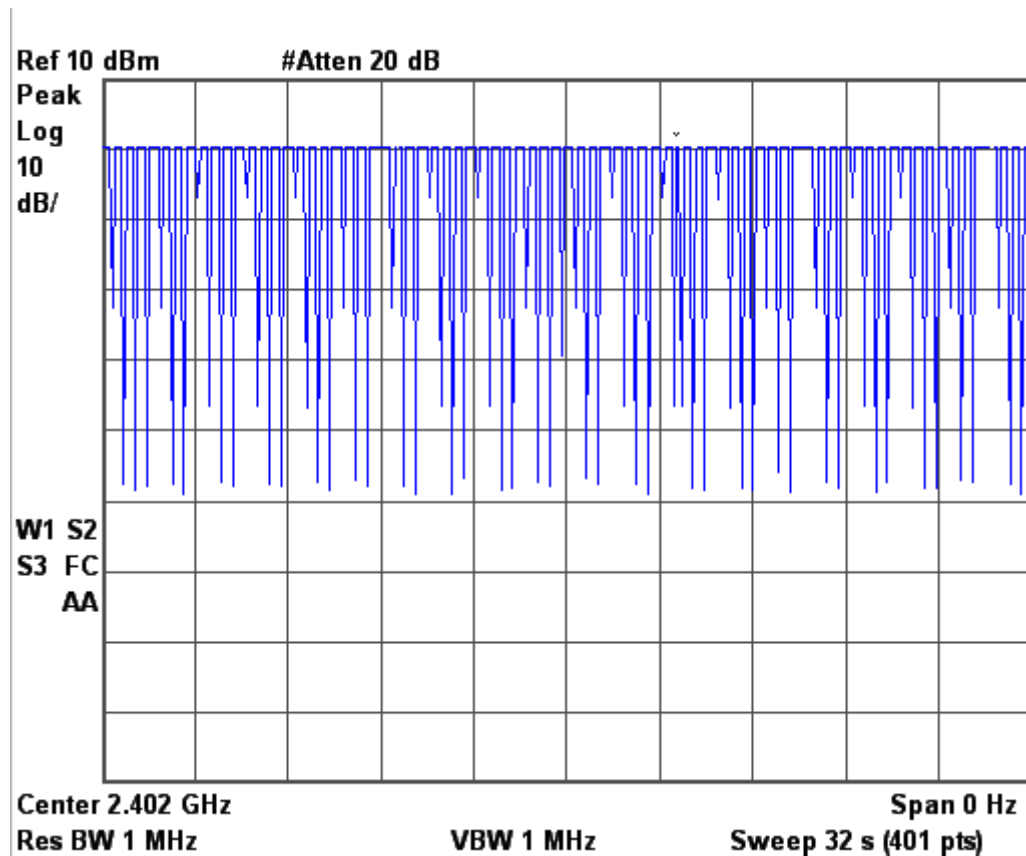
Figure 6c.4-1: Plot of dwell time over 32 second period
