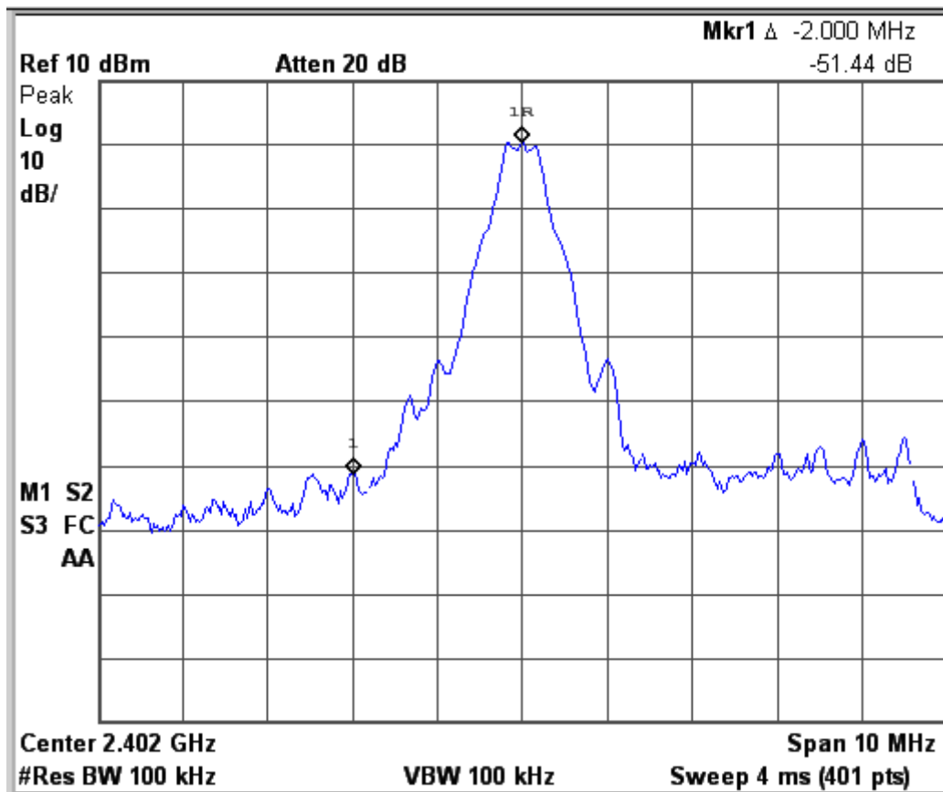
Figure 6c.6-1: Plot of lower band-edge conducted emissions with hopping disabled
