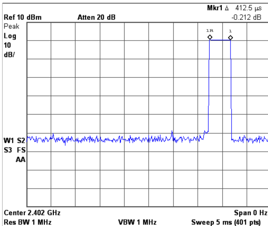
Figure 6c.4-3: Plot of dwell time over 5 ms period.
