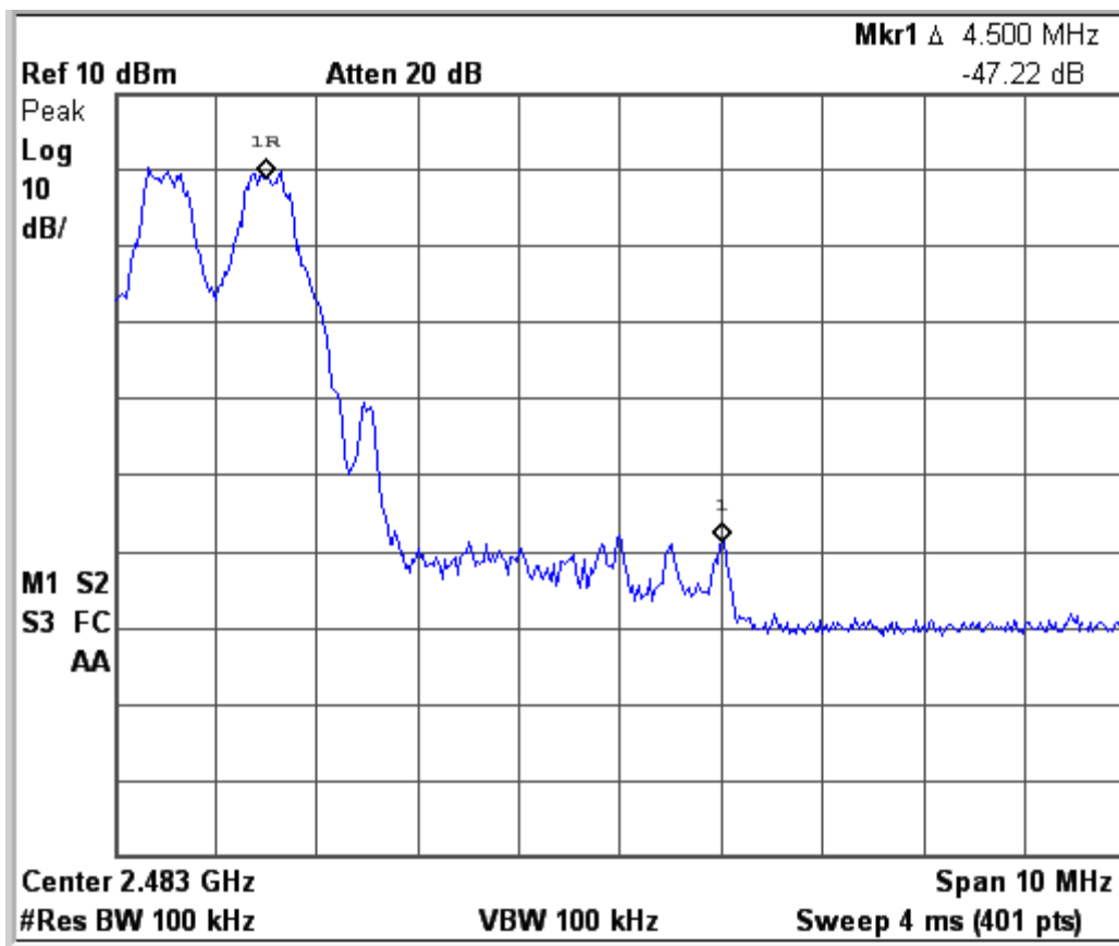
Figure 6c.6-4: Plot of upper band-edge conducted emissions with hopping enabled.
