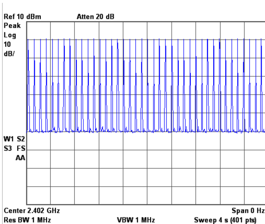
Figure 6c.4-2: Plot of dwell time over 4 second period.
