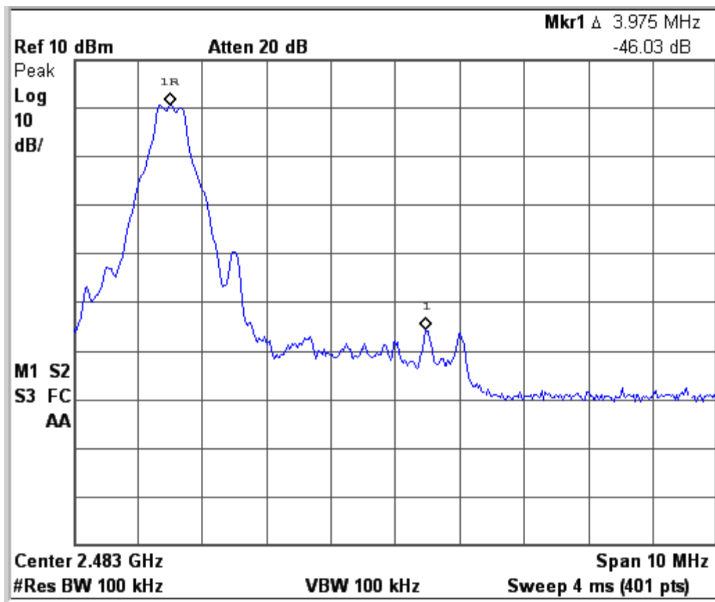
Figure 6c.6-2: Plot of upper band-edge conducted emissions with hopping disabled.
