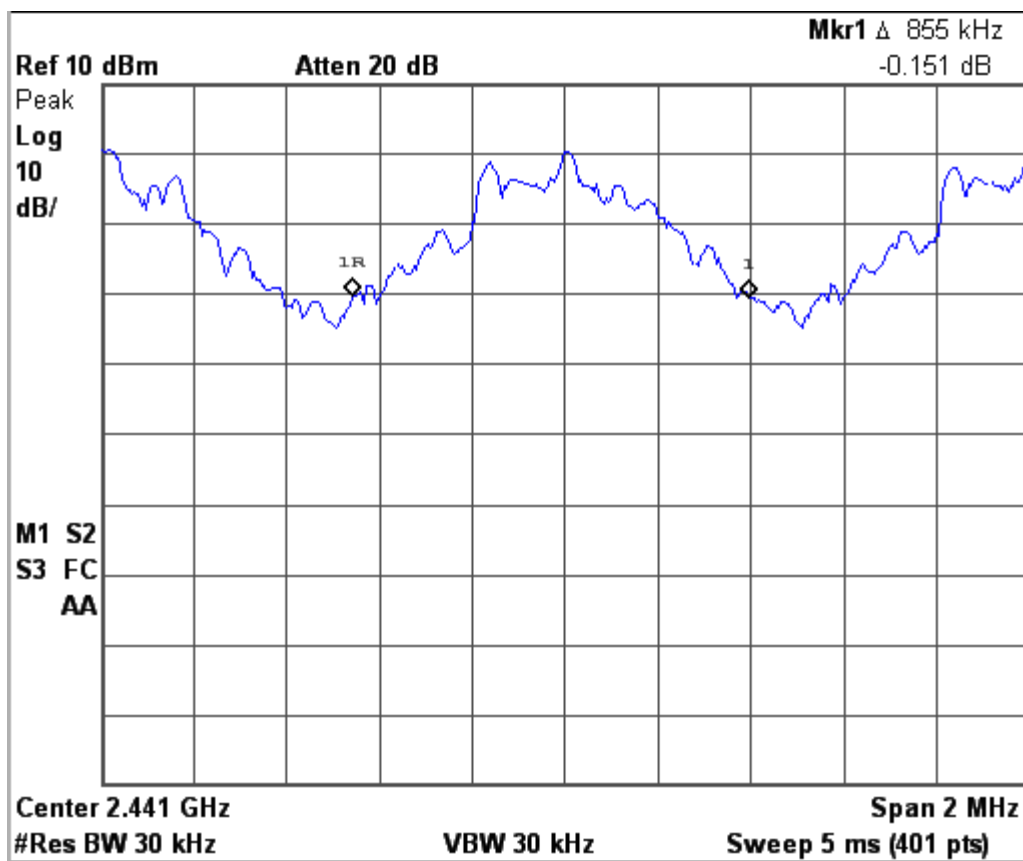
Figure 6c.2-1: Plot of 20 – dB bandwidth
