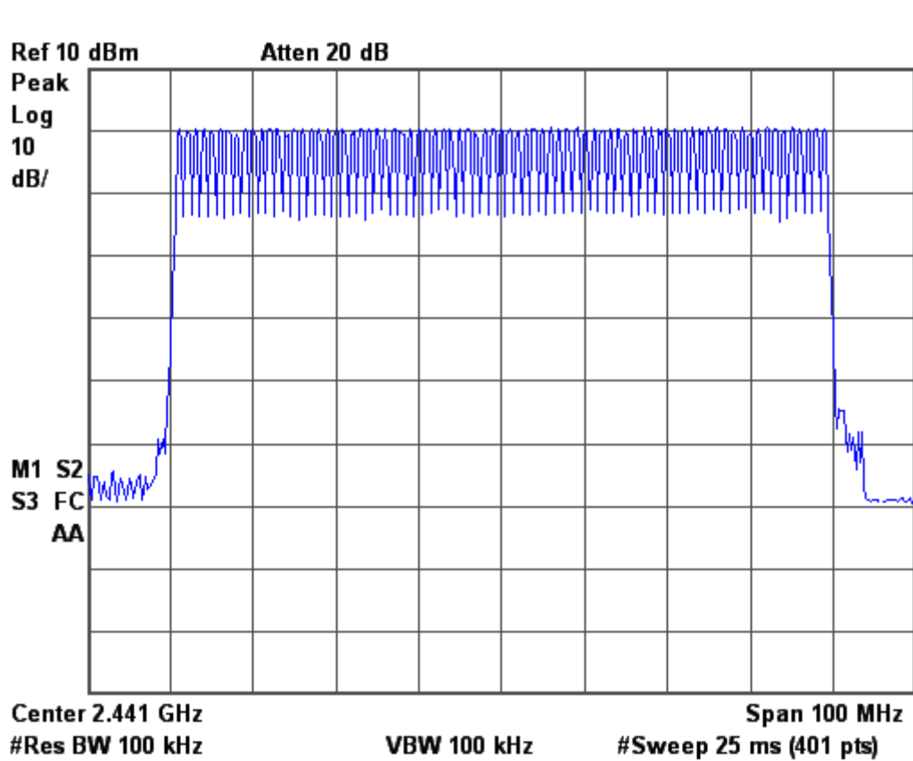
Figure 6c.3-1: Plot of number of Bluetooth hopping frequencies
