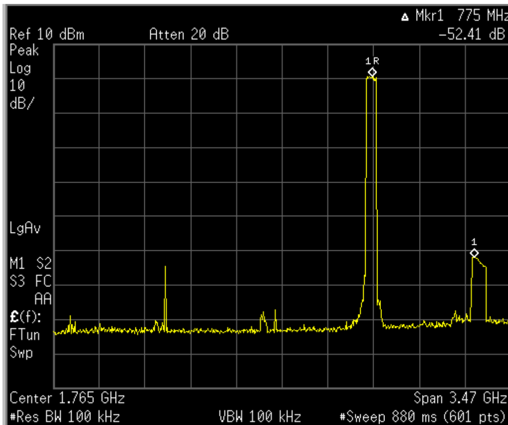
Figure 6c.7-1: Plot of spurious conducted emissions 30 MHz – 3.5 GHz.
