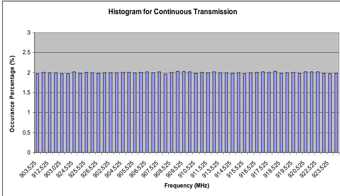
Figure 6b.2.6.1. Histogram of MOTotalk ISM Band Continuous Transmission.
