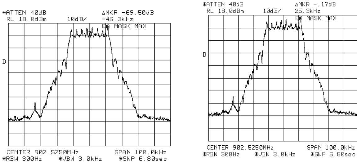
Figure 6b.2.2.1 Spectrum analyzer plot of MOTotalk ISM Band 8-FSK traffic channel signal’s 99% bandwidth at center frequency 902.525 MHz, with hopping function disabled.
