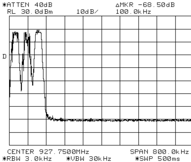
Figure 6b.2.2.8. Out-of-band transmitter spurious emissions high band edge, with hopping function enabled.
