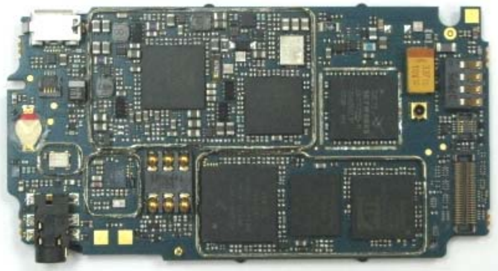
Photograph 9-2: Component side of radio product PC Board, Shields removed.
