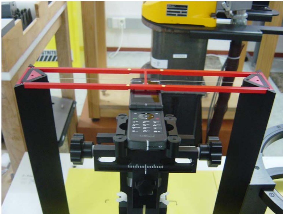
Figure A4-6. Positioning and Measurement for T-coil (Front)
