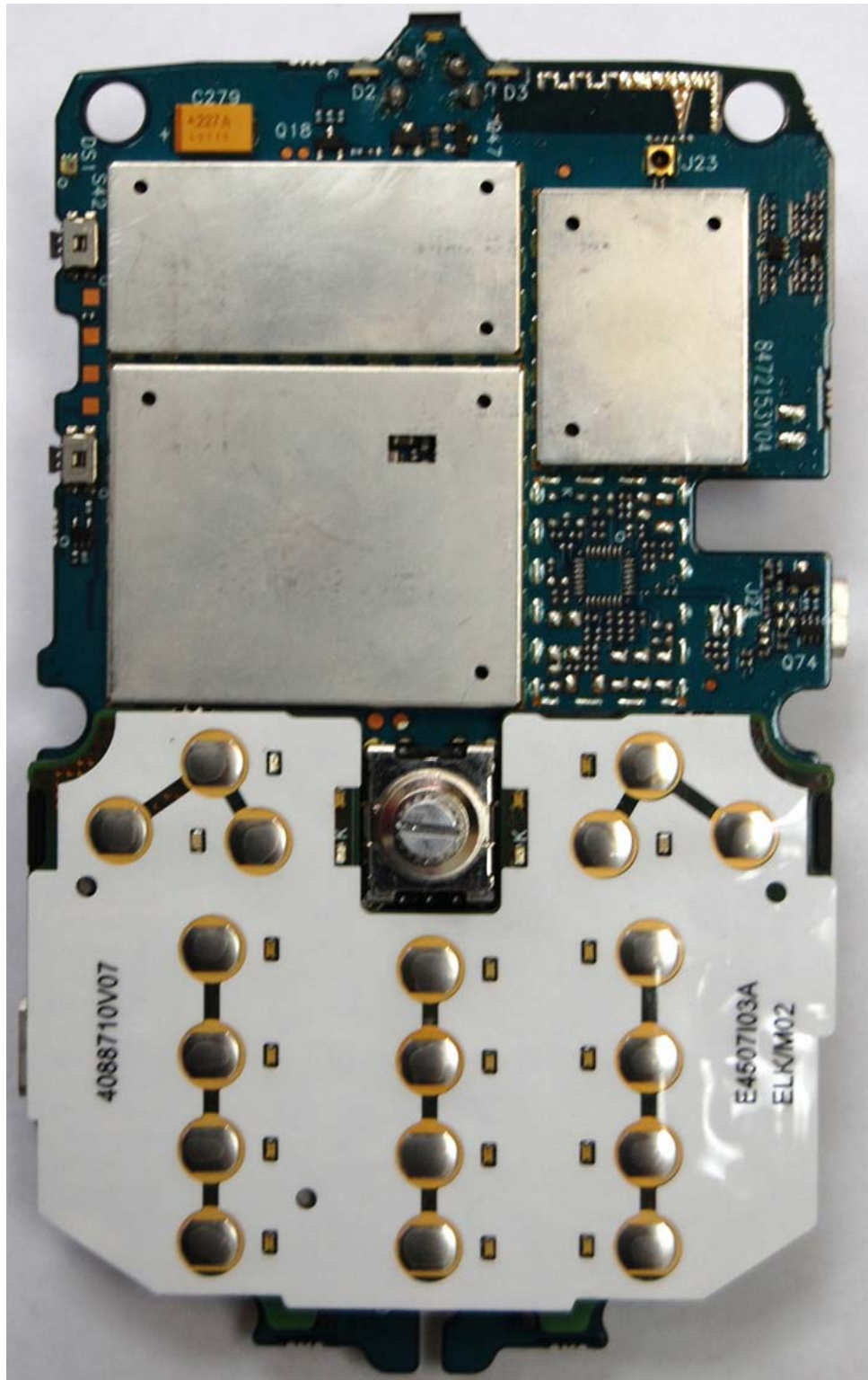
M 990 PI - Internal view
