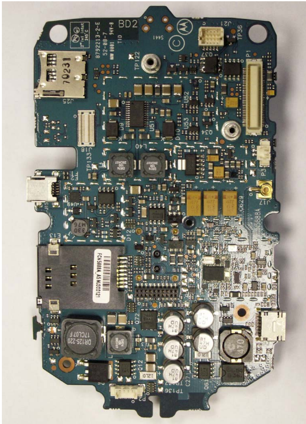
M 990 PI - Internal view with shields removed
