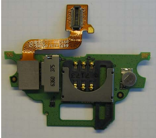
Daughter Board Top
