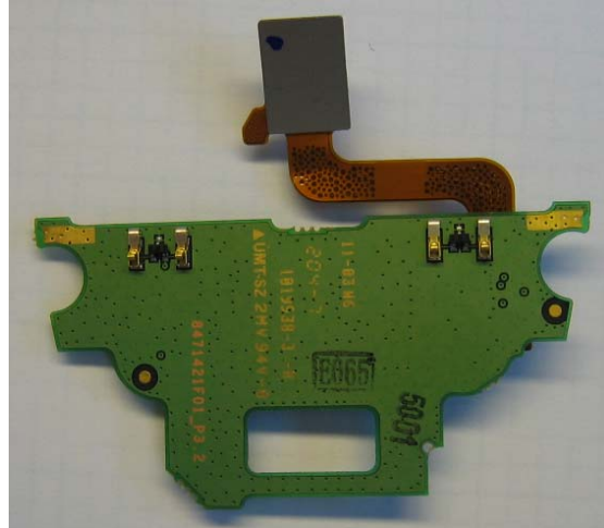
Daughter Board Bottom
