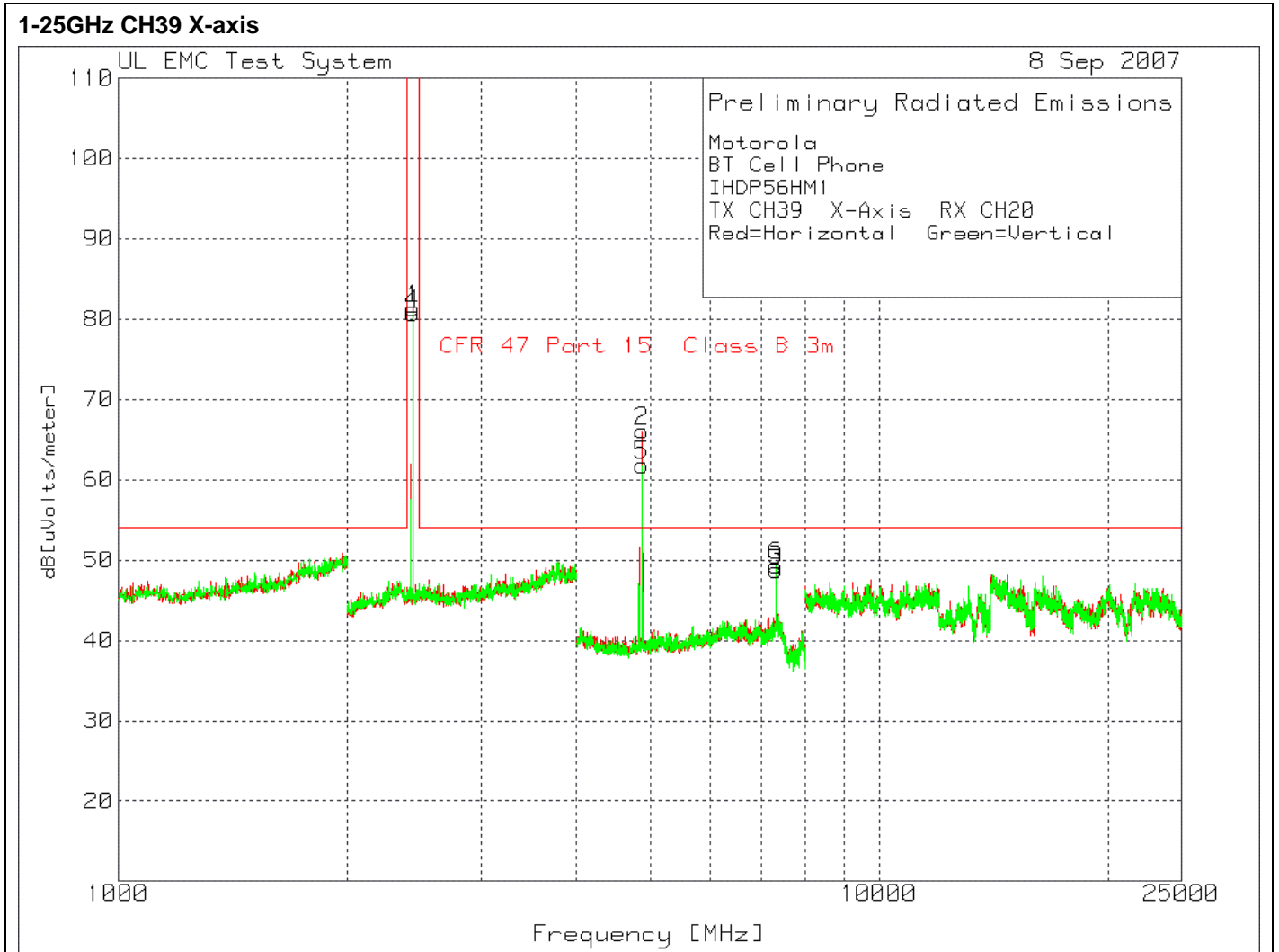
Figure 14 Radiated Emissions Graph
