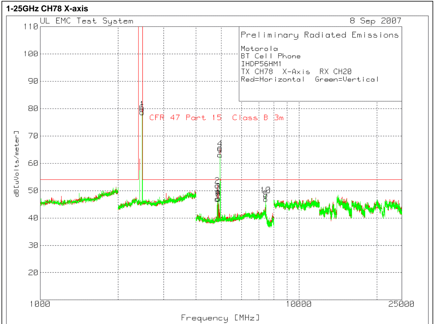
Figure 17 Radiated Emissions Graph
