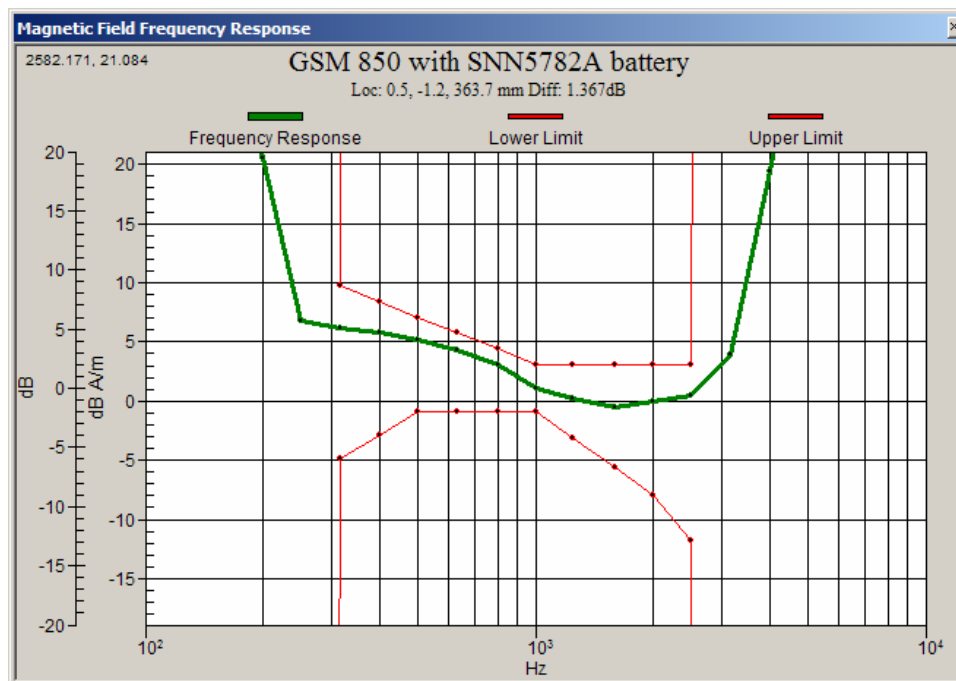
Graph 2: Frequency Response Plots
