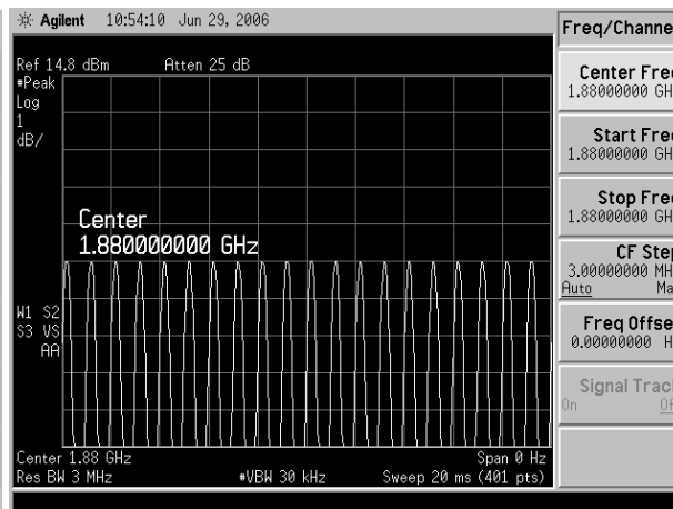
80% AM 1880 MHz
