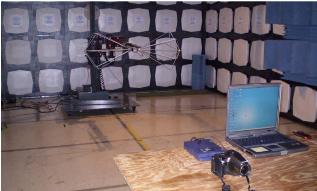
Figure 2. Radiated Emissions
