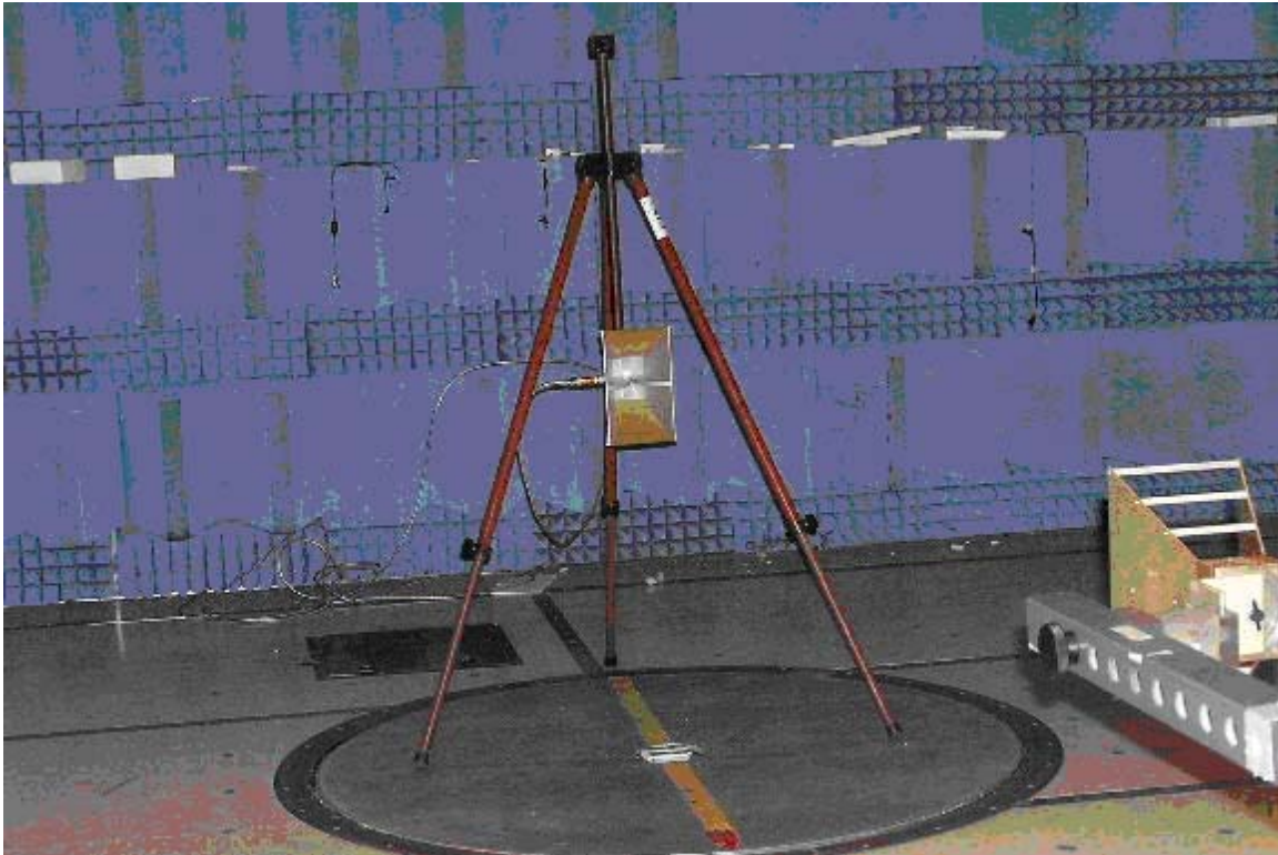
Figure 3. Antenna - Substitution
