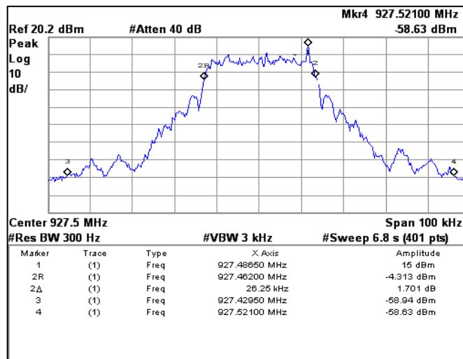
Figure 6b.2.2.5 Spectrum analyzer plot of MOTotalk ISM Band 8-FSK traffic channel signal's 99% bandwidth with hopping function disabled, at center frequency 927.475 MHz.
