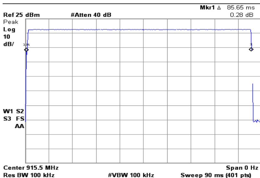
Figure 6b.2.5.1. MOTotalk ISM Band Average Measured Time of Occupancy.
