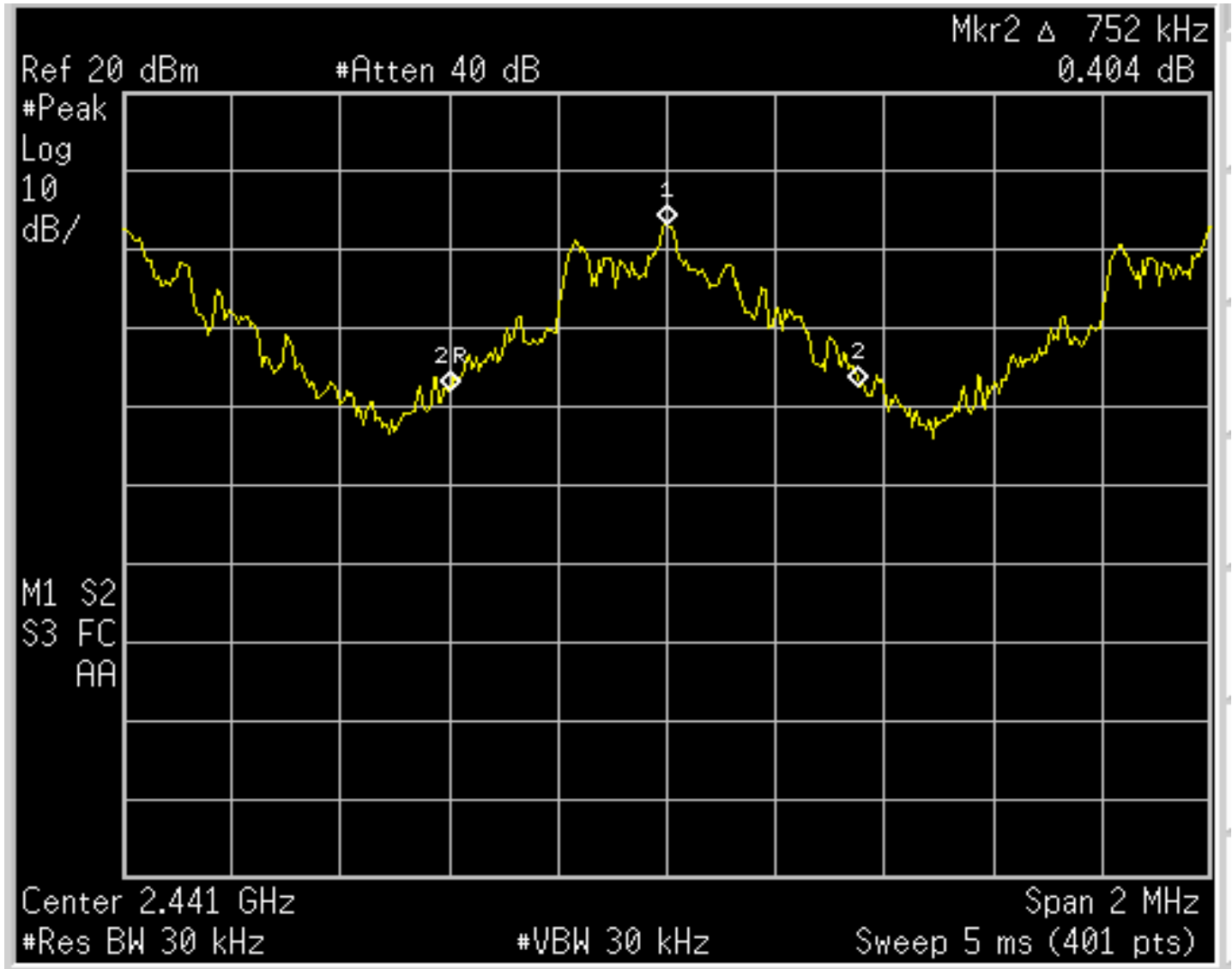
Figure 6c.2-1: Plot of 20 – dB bandwidth
