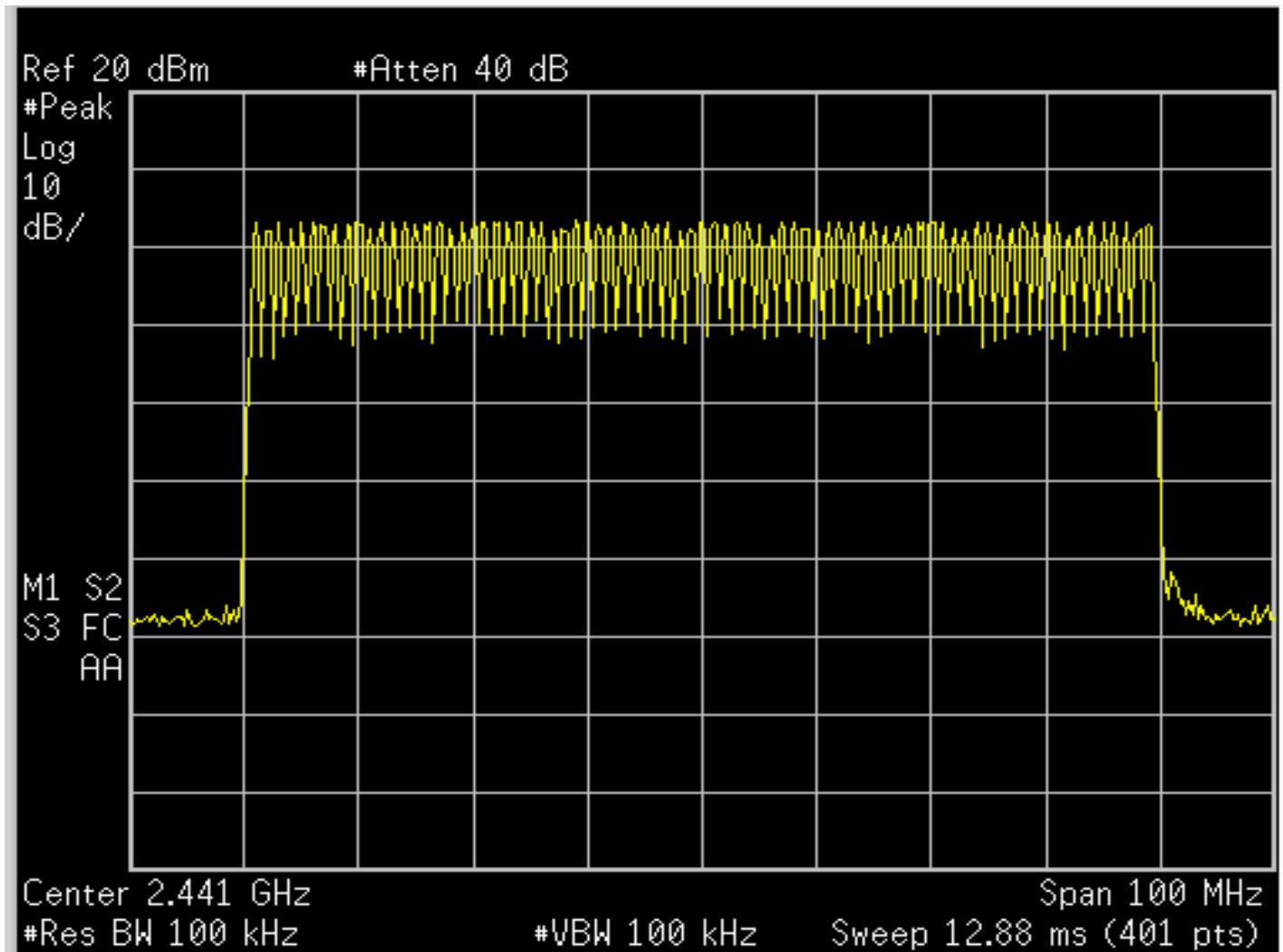
Figure 6c.3-1: Plot of number of Bluetooth hopping frequencies
