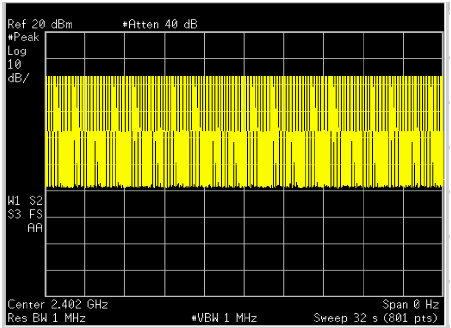
Figure 6c.4-1: Plot of dwell time over 32 second period
