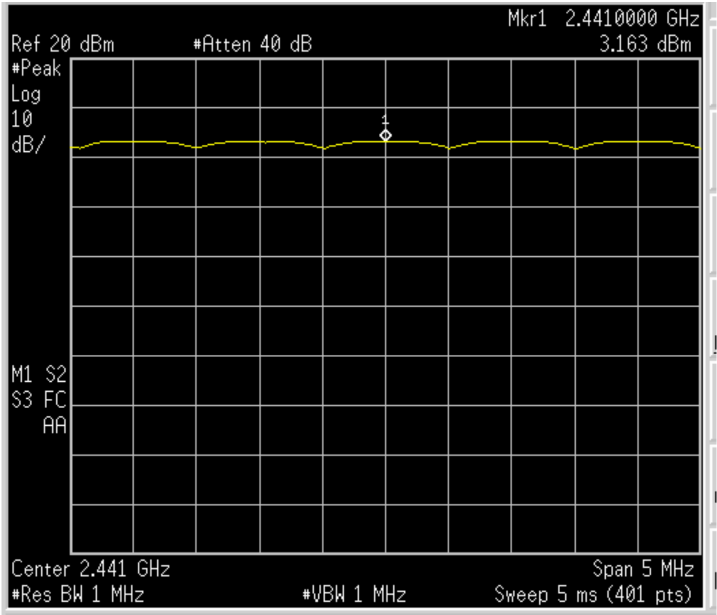
Figure 6c.5-1: Plot of peak output power
