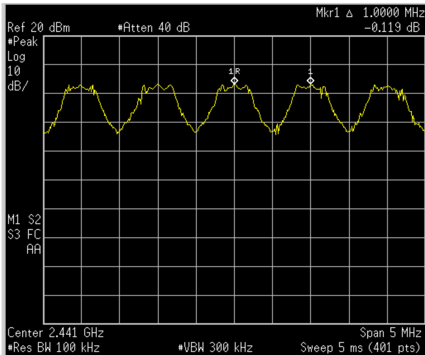
Figure 6c.1-1: Plot of Bluetooth carrier frequency separation
