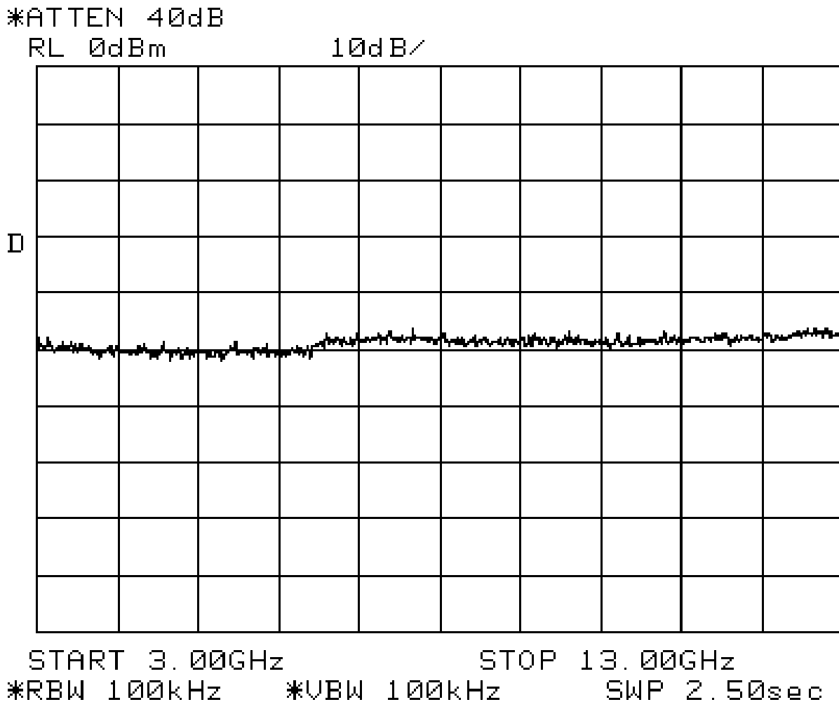
Figure 6c.7-2: Plot of spurious conducted emissions 3 GHz – 13 GHz.
