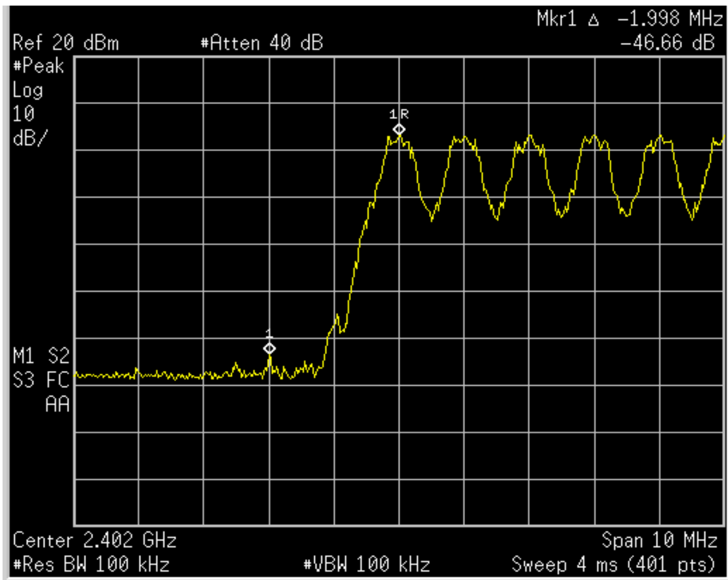
Figure 6c.6-3: Plot of lower band-edge conducted emissions with hopping enabled.
