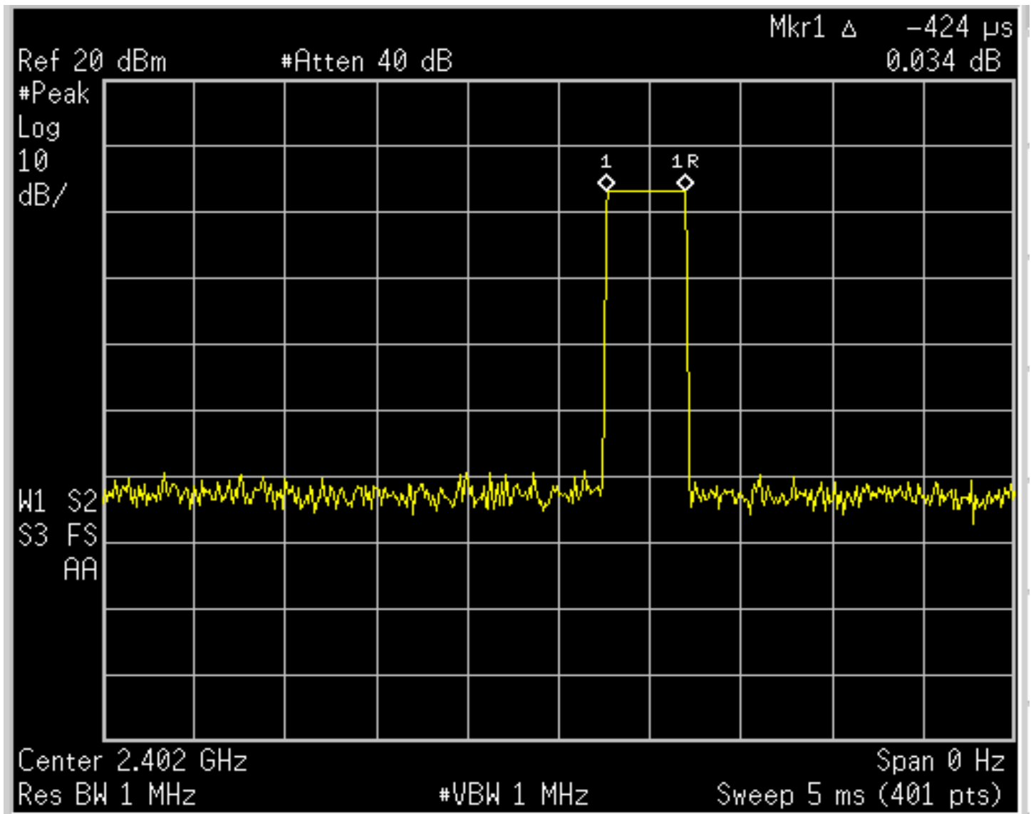
Figure 6c.4-3: Plot of dwell time over 5 ms period.
