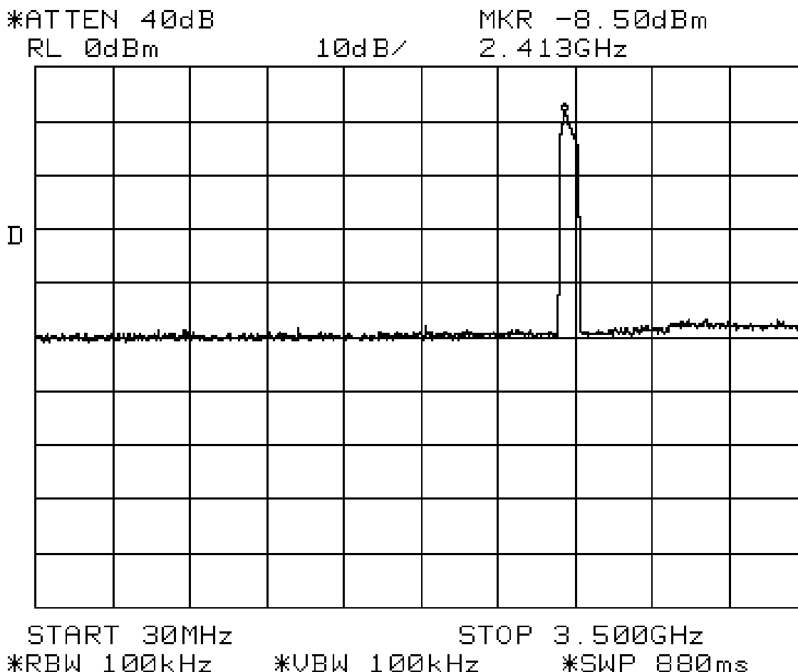
Figure 6c.7-1: Plot of spurious conducted emissions 30 MHz – 3.5 GHz.
