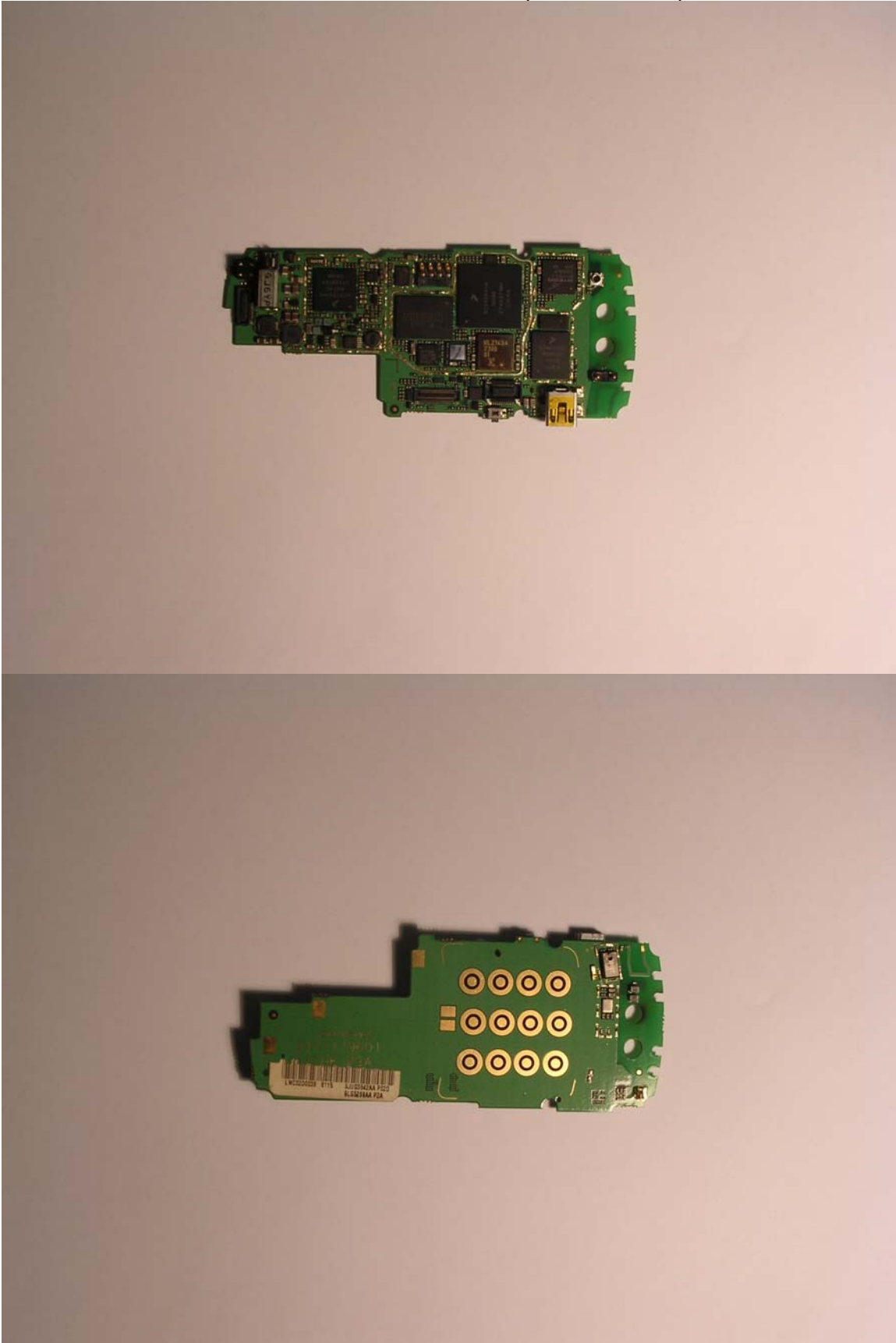
Main Board without Shields (Front & Back)
