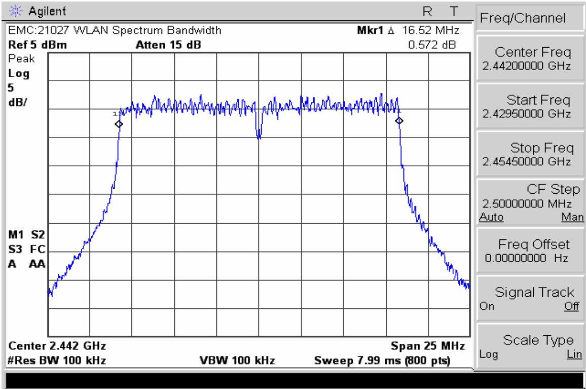
6dB Bandwidth Channel 7 @ 36 Mbps
