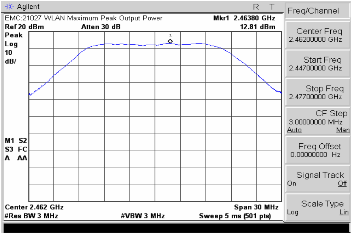
Max. Power Channel 11 @ 36 Mbps
