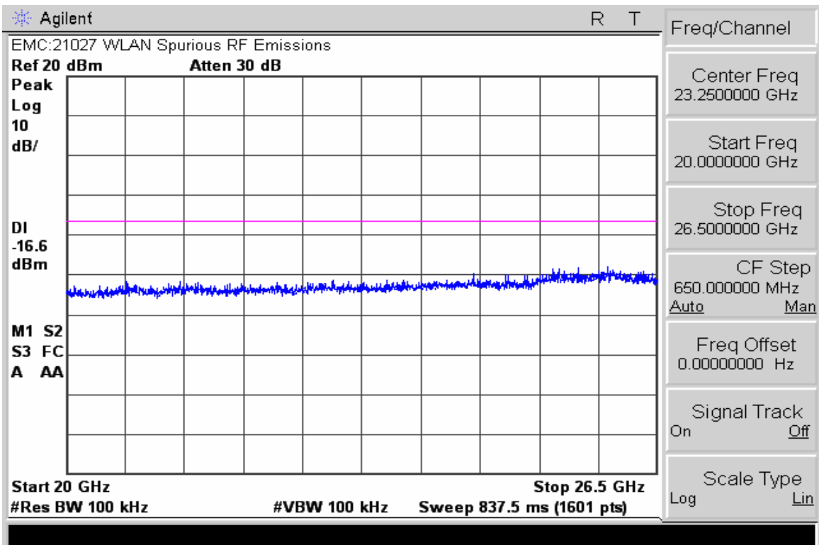
Conducted Spurious Emissions 20-26.5GHz (Mid Channel Enabled)
