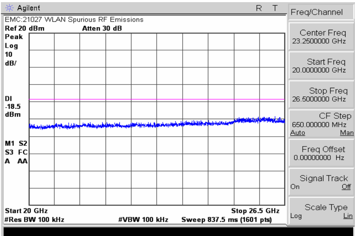
Conducted Spurious Emissions 20-26.5GHz (High Channel Enabled)
