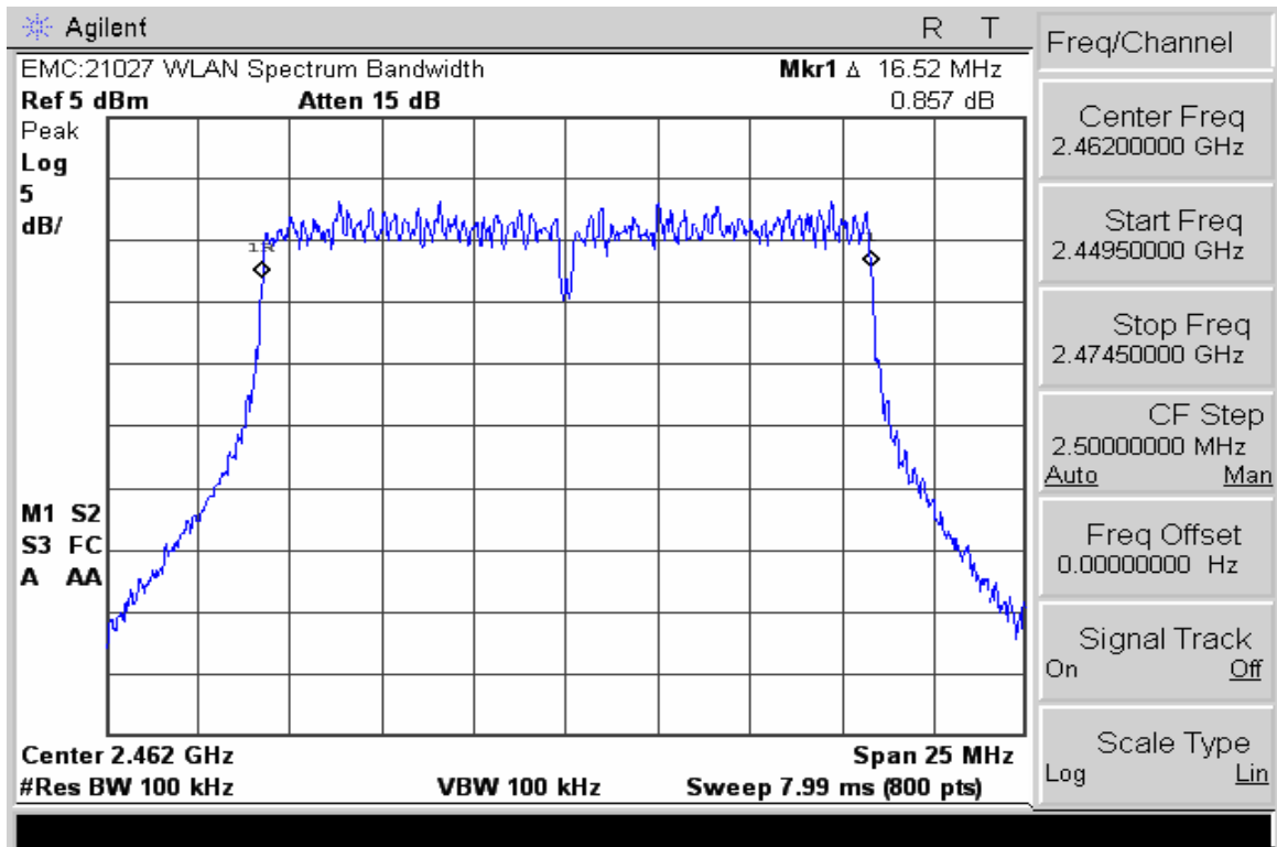
6dB Bandwidth Channel 11 @ 36 Mbps
