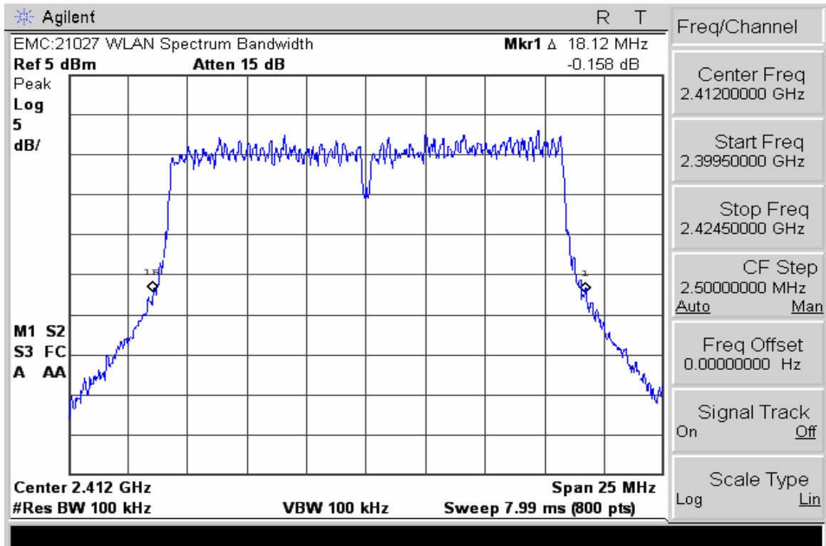
20dB Bandwidth Channel 1 @ 36 Mbps
