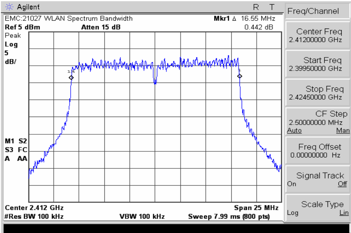
6dB Bandwidth Channel 1 @ 36 Mbps
