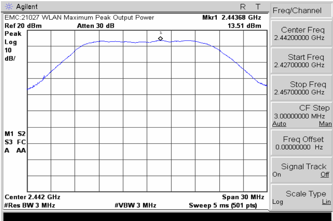
Max. Power Channel 7 @ 36 Mbps
