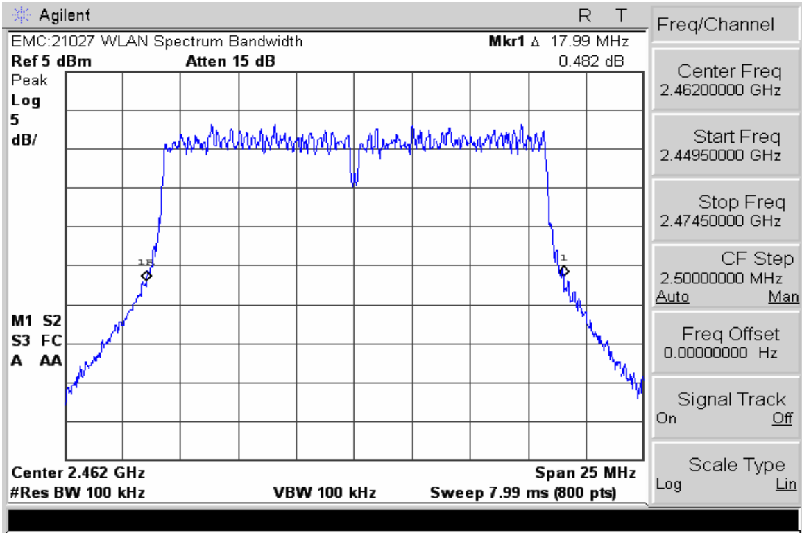
20dB Bandwidth Channel 11 @ 36 Mbps
