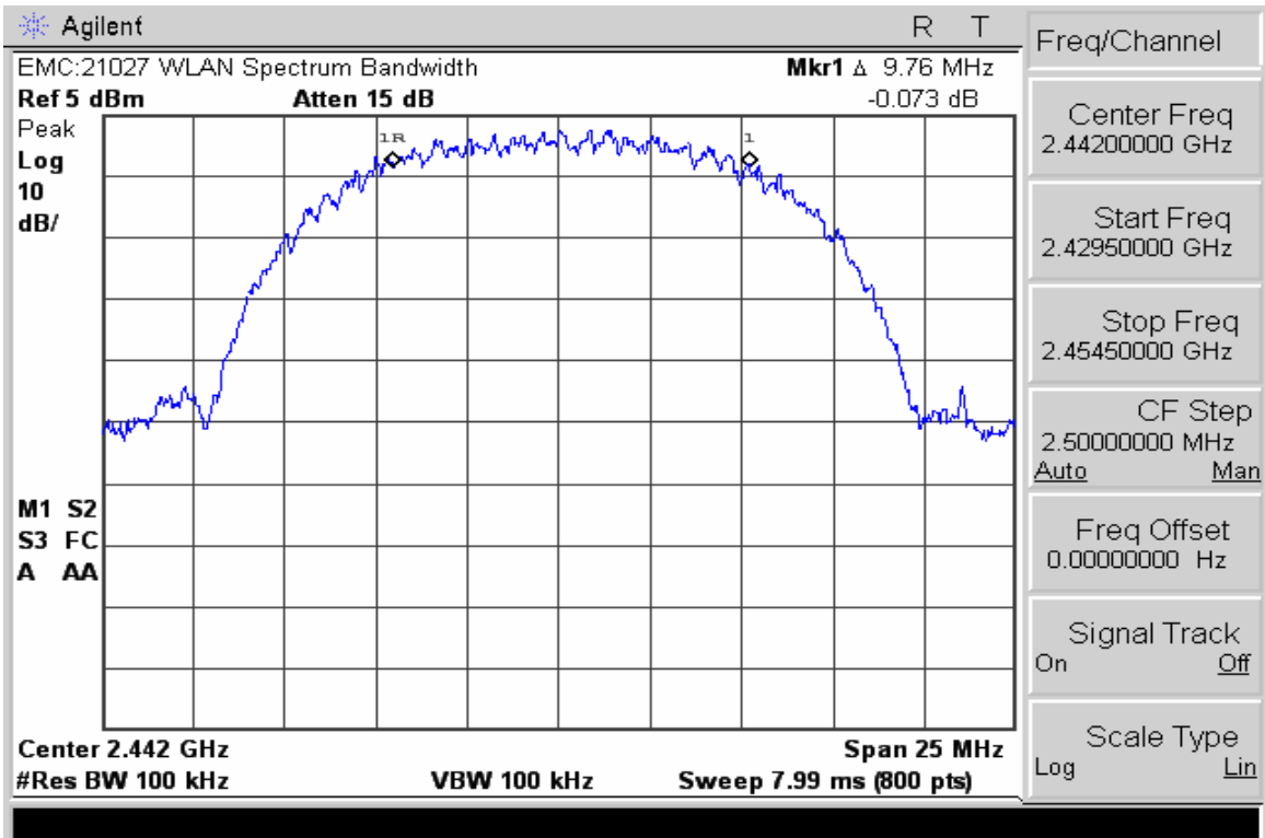
6dB Bandwidth Channel 7 @ 11 Mbps
