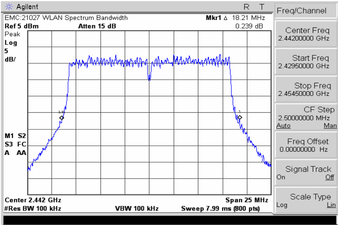
20dB Bandwidth Channel 7 @ 36 Mbps
