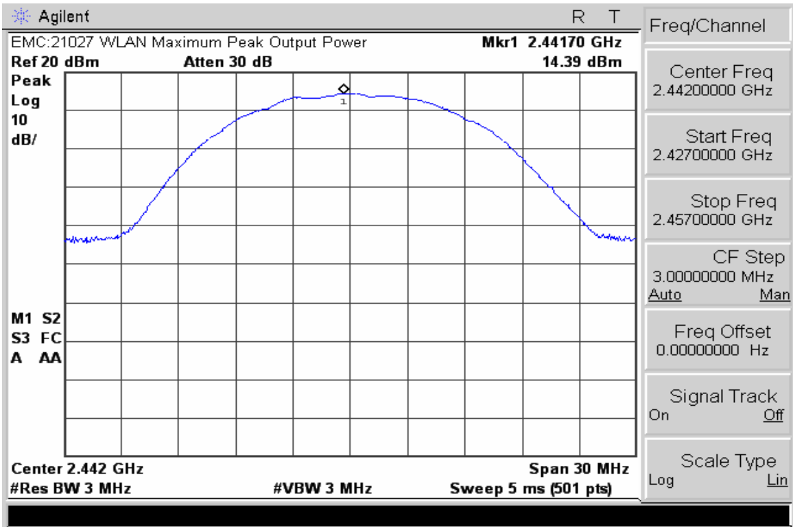
Max. Power Channel 7 @ 11 Mbps
