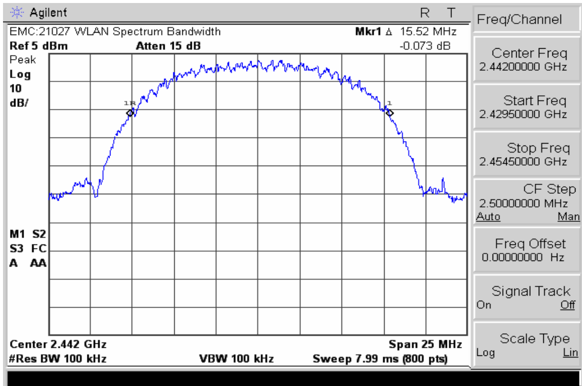
20dB Bandwidth Channel 7 @ 11 Mbps
